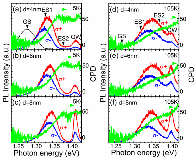
FIG. 1. 5 K (a)–(c) and 105 K (d)–(f) circular-polarized PL spectra and corresponding CPD from QW-QD tunnel-coupled structures with 4 nm, 6 nm, and 8 nm-thick barriers. The QD GS PL measured by another detector is shown as dashed line in (a).
