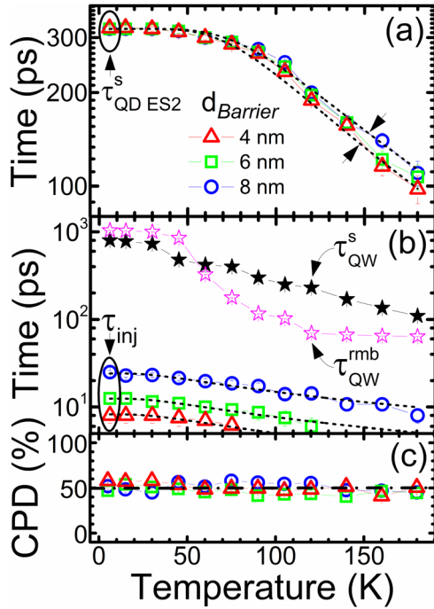
FIG. 5. The temperature dependence of electron spin relaxation time, \tau_{QD,ES2}^s , at QD ES2, phonon-assisted carrier injection time, \tau_{inj} , and initial CPD, CPD_{t=0} , of QD ES2 is summarized in (a), (b), and (c), respectively, for 4 nm (triangle), 6 nm (square), and 8 nm (dot) barrier samples. For comparison, a reference single QW sample was measured, whose recombination, \tau_{QW}^{rmb} , and electron spin relaxation time, \tau_{QW}^s , are displayed as open and solid stars in (b). Fittings to \tau_{QD,ES2}^s and \tau_{inj} are provided as dashed lines.
