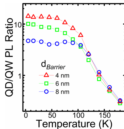
FIG. 2. PL intensity ratio between entire QD emission and QW as a function of temperature for samples with 4 nm, 6 nm, and 8 nm-thick barriers.
