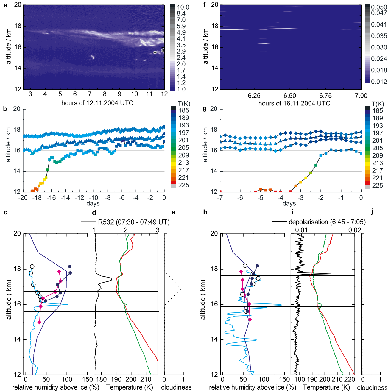
Figure 6. Same as Figure 5 but for (a–e) 12 November and (f–j) 16 November 2004, except for Figure 6f which shows the volume depolarization instead of the backscatter ratio at 532 nm, because of the extremely thin layer of particles was not visible in the parallel backscatter. In Figures 6d and 6i the existence temperature of NAT is plotted in green. The balloons that measured relative humidity and temperature in Figures 6c, 6d, 6h, and 6i were launched at 0644 UTC (12 November 2004) and 0626 UTC (16 November 2004).
