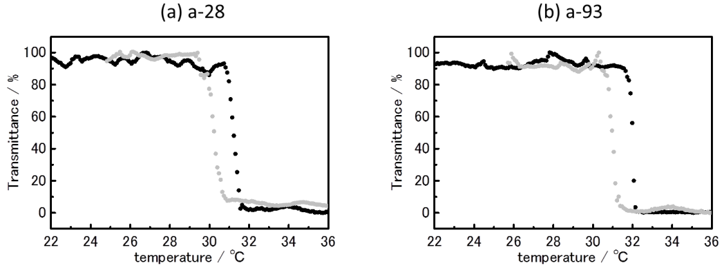
Figure 3-3. Temperature dependences of the optical transmittance at 532 nm observed for aqueous (a) a-28, and (b) a-93 solutions. The black and gray curves show the transmittance changes upon heating and cooling, respectively. Heating and cooling rate = 0.2 °C min -1 .
