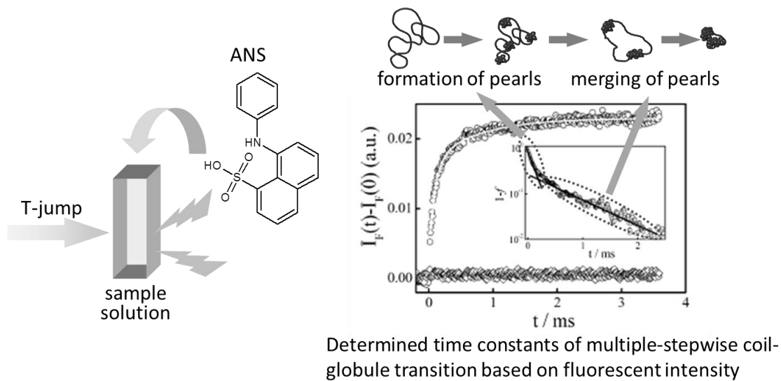
Figure 1-5. Schematic illustration of a laser-induced T-jump study on the coil-globule transition in an aqueous PNIPAM solution based on the fluorescence intensity change of 8-anilino-1-naphthalensulfonic acid (ANS) added to the solution upon transition [88], [89]. The graph shows the time dependences of the fluorescence intensity changes of ANS after a T-jump with and without PNIPAM. The inset shows a semilogarithmic plot of (1 - f) vs time ( t ), where f is defined as [I_F(t) - I_F(0)]/[I_F(\infty) - I_F(0)] = 1 - A \exp(-t/\tau_{\text{fast}}) - (1 - A) \exp(-t/\tau_{\text{slow}}) . Reprinted with permission from the American Chemical Society.
