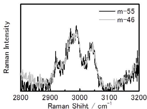
Figure 4-9. Raman spectra of aqueous m-46 and m-55 solutions (5.0 wt%) at room temperature. The observed peaks at 2923, 2967, 2983 and 3043 \text{cm}^{-1} are ascribed to those of the C-H stretching vibrations.
