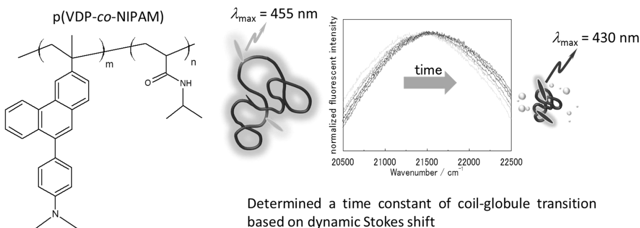
Figure 1-6. Structure of p(VDP-co-NIPAM) and microsecond-time-resolved dynamic Stokes shift of the fluorescence in an aqueous p(VDP-co-NIPAM) solution (1.0 wt.%) after a T-jump. The direction of the temporal evolution is indicated by the arrows in the figure. Reprinted with permission from Elsevier.
