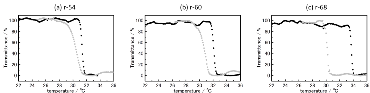
Figure 5-8. Temperature dependences of the optical transmittance at 532 nm for the aqueous (a) r-54, (b) r-60, and (c) r-68 solutions. The black and gray curves show the transmittance changes upon heating and cooling, respectively. Heating and cooling rate = 0.2\text{ }^{\circ}\text{C min}^{-1} .
