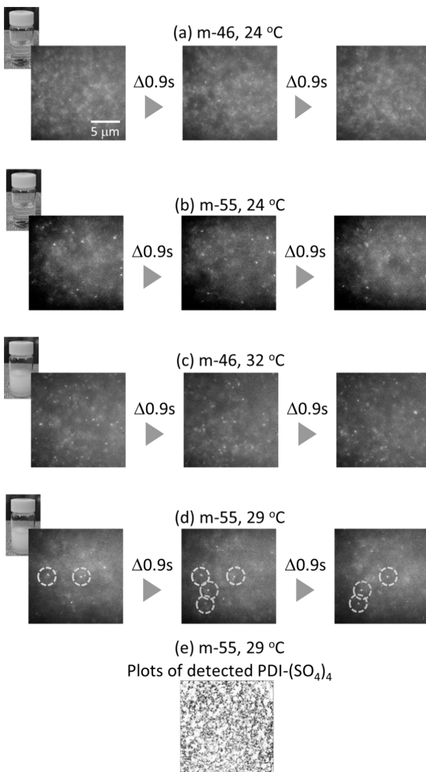
Figure 4-10. Fluorescence images of PDI-(SO 4 ) 4 in aqueous solutions of (a) m-46 at 24 °C, (b) m-55 at 24 °C, (c) m-46 at 32 °C, (d) m-55 at 29 °C. The concentrations of the polymers and PDI-(SO 4 ) 4 are 5.0 wt% and 10 -10 M, respectively. Scale bar = 5 μm. (e) Fluorescence intensity distribution of PDI-(SO 4 ) 4 observed for an aqueous m-55 solution at 29 °C accumulated for 200 frames. The black color corresponds to the fluorescence.
