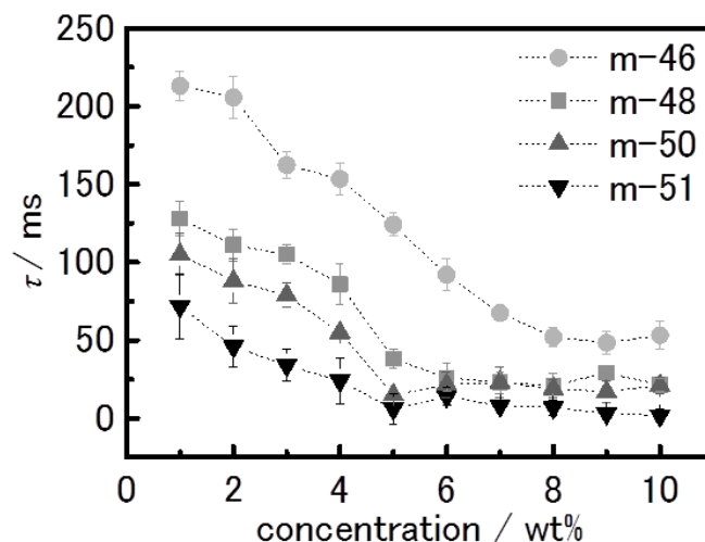
Figure 4-7. Phase separation time constants as a function of the concentration of the polymer (1.0 – 10 wt%) observed for aqueous m-51, m-50, m-48 and m-46 solutions. ●: m-46, ■: m-48, ▲: m-50, ▼: m-51.
