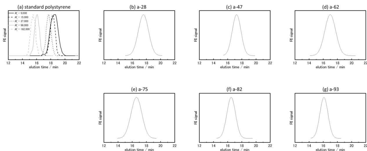
Figure 3-2. SEC chromatograms of (a) standard polystyrene samples (solid black line: M_n = 9,000 , dashed black line: M_n = 15,000 , dotted black line: M_n = 37,000 , solid gray line: M_n = 98,000 , and dashed gray line: M_n = 182,000 ), (b) a-28, (c) a-47, (d) a-62, (e) a-75, (f) a-82, and (g) a-93. These chromatograms were measured at 40 °C using N,N -dimethylformamide containing 0.1 M of LiBr as an eluent.
