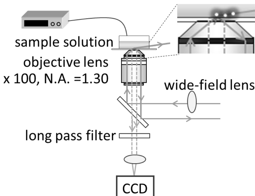
Figure 4-4. Schematic illustration of the optical setup for quasi-total-internal-reflection fluorescence microscopy.
