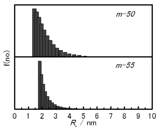
Figure 4-8. Hydrodynamic radius distributions of m-50 and m-55 in aqueous solutions (1.0 wt%) at room temperature.
