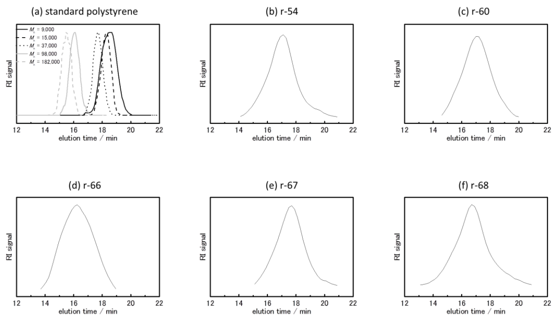
Figure 5-1. SEC chromatograms of (a) standard polystyrene samples (solid black line: M_n = 9,000 , dashed black line: M_n = 15,000 , dotted black line: M_n = 37,000 , solid gray line: M_n = 98,000 , and dashed gray line: M_n = 182,000 ), (b) r-54, (c) r-60, (d) r-66, (e) r-67, and (f) r-68. These chromatograms were measured at 40 °C using N,N -dimethylformamide containing 0.1 M of LiBr as an eluent.
