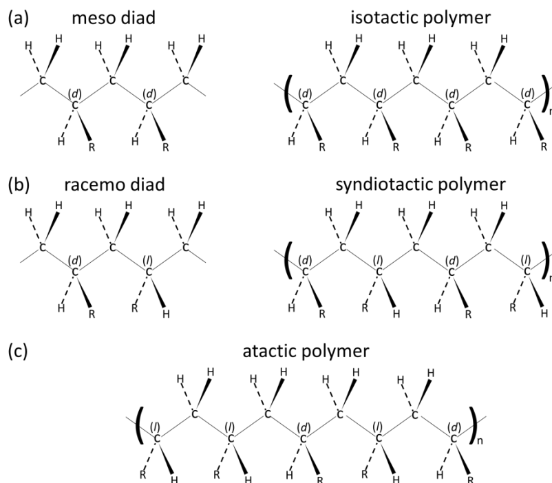
Figure 1-3. Schematic illustration of the definition of the stereoregularity of an asymmetric chain of the type [(CH_2)-(CHR)]_n .
