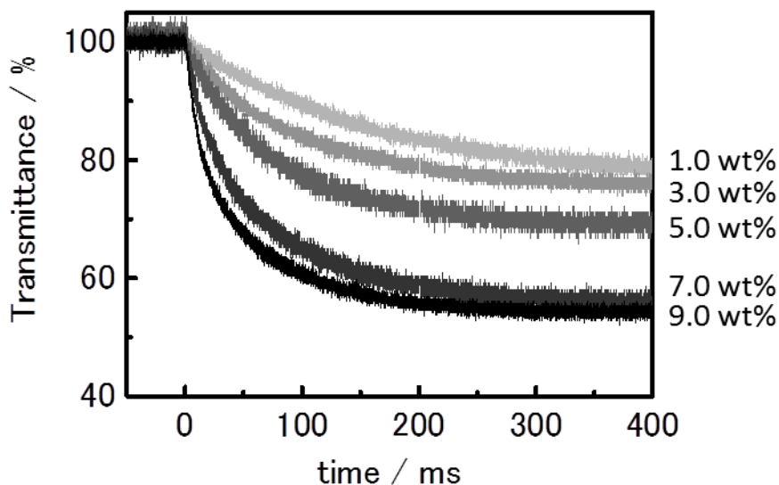
Figure 3-4. Representative curves of the time courses of the transient optical transmittance T(t) as a function of the polymer concentration of a-47 (1.0–9.0 wt%) in water. The origin of the time scale ( t = 0 ) is the time when the heating pulse reaches the cell.
