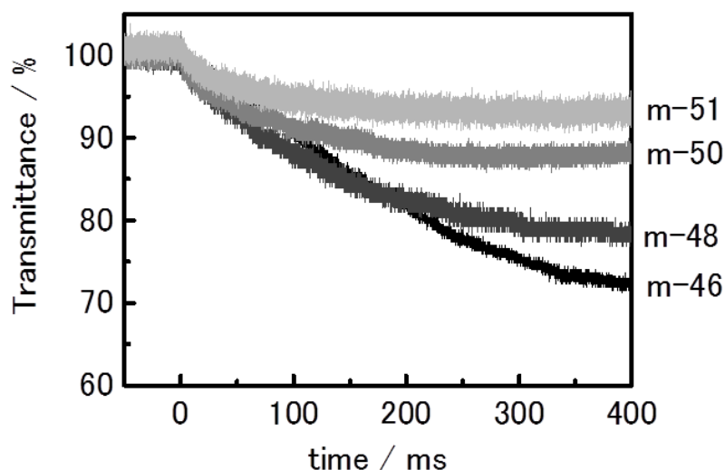
Figure 4-6. Typical examples of the time courses of the transient optical transmittance T(t) observed for aqueous m-51, m-50, m-48 and m-46 solutions (1.0 wt%).
