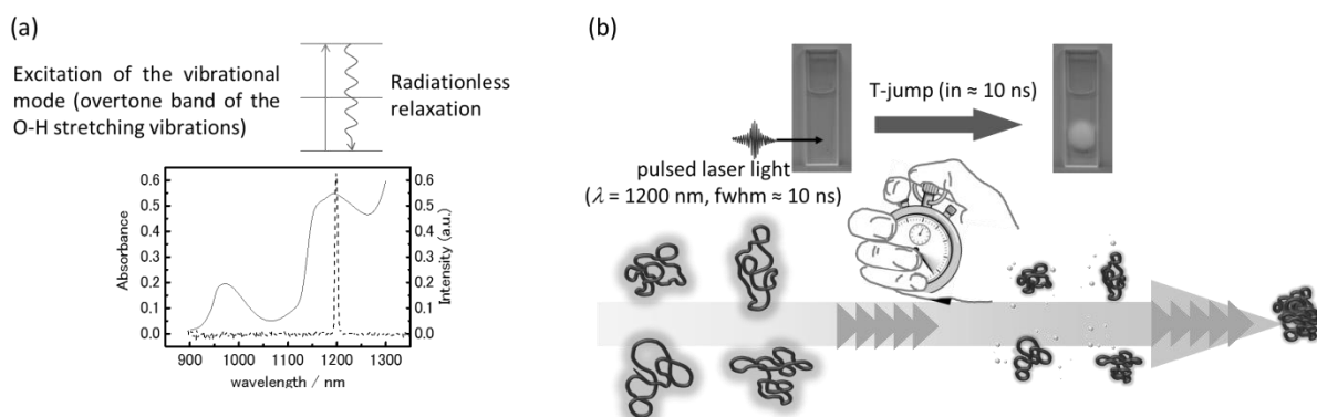
Figure 1-7. (a) Infrared absorption spectrum of water (solid line) and laser spectrum used in this thesis (dashed line) (Spectra Physics, PRO-130-10, \lambda = 1200 nm, \text{fwhm} \approx 10 ns). An aqueous solution absorbs 1200 nm light through the overtone band of the O-H stretching vibrations of water and accordingly the temperature of the irradiated volume in the sample solution can be raised within the time scale of the incident laser pulse width: nanosecond time scale ( \approx 10 ns). (b) Basic concept of the present study. Phase separation of the aqueous PNIPAM solution is triggered by irradiation with an infrared laser beam and the time constants of the phenomena are determined.
