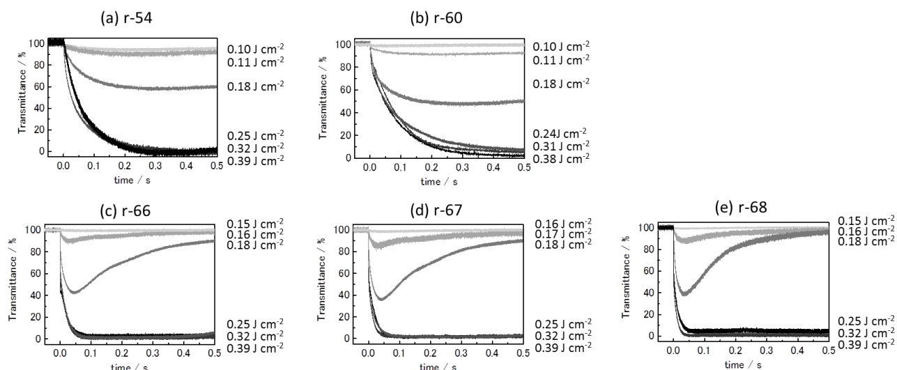
Figure 5-4. Typical examples of the time courses of the transient transmittance T(t) in aqueous (a) r-54, (b) r-60, (c) r-66, (d) r-67, and (e) r-68 solutions (5.0 wt%) in the presence of crystal violet (0.50 mM) as a function of an incident heating laser pulse energy.
