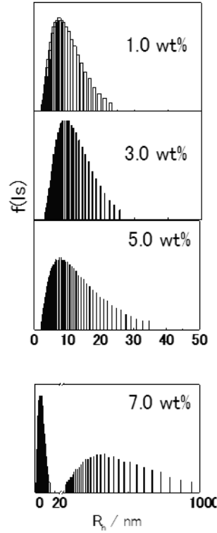
Figure 3-6. Typical examples of the concentration dependence of the hydrodynamic radius histogram observed for a-47 by dynamic light scattering measurements. The concentration of the sample solution is given in the figure.
