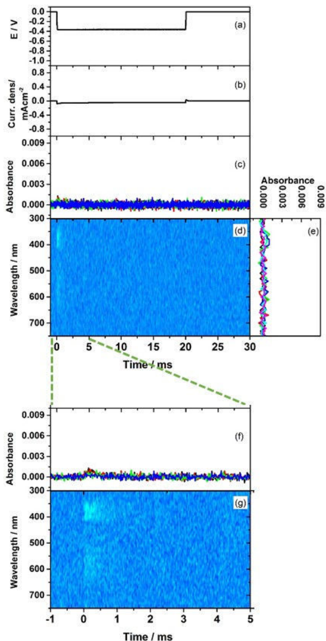
Figure 5-8. (a) potential profile (from 0 to -0.36 V), (b) current response, (c) absorbance response at 375 (black), 400 (red), 550 (blue), and 600 nm (green), (d) contour of the absorbance as functions of probe wavelength and time after the potential step, and (e) time resolved spectra at -0.5 (black), 0 (red), 0.1 (green), 0.2 (blue), 0.5 (light blue) and 2 ms (pink) after the potential step of 1LV-ITO/Pt-complex. (f) Absorbance response 375 (black), 400 (red), 550 (green), and 600 nm (blue), and (g) contour of the absorbance as functions of probe wavelength and time after the potential step of the initial 5ms to the potential step.
