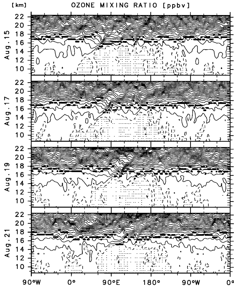
Figure 5. Longitude-altitude distributions of ozone mixing ratio between 9 and 22 km at the equator ( 1.3953^\circ\text{N} ) on August 15, 17, 19, and 21 of the fifteenth year. The contour interval is 100 ppbv. Dashed lines are added for 50 ppbv. The shaded regions correspond to those of less than 50 ppbv. The location of the tropopause is indicated by solid circles. Note that the region 90^\circ\text{W} - 0^\circ is duplicated.
