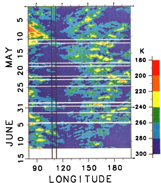
Plate 3. Variation of the infrared equivalent blackbody temperature, which represents the convective activity, along the latitudinal band between 5.5^\circ\text{S} and 9.5^\circ\text{S} from the Geostationary Meteorological Satellite data. The observational sites are indicated by lines.
