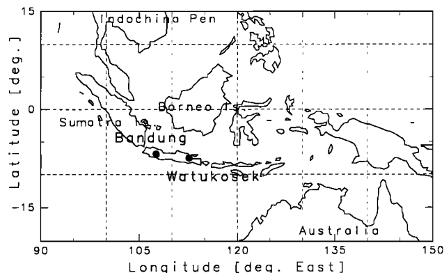
Figure 1. The locations of the observational sites, Watukosek (7.5°S, 112.6°E) and Bandung (6.9°S, 107.6°E).
