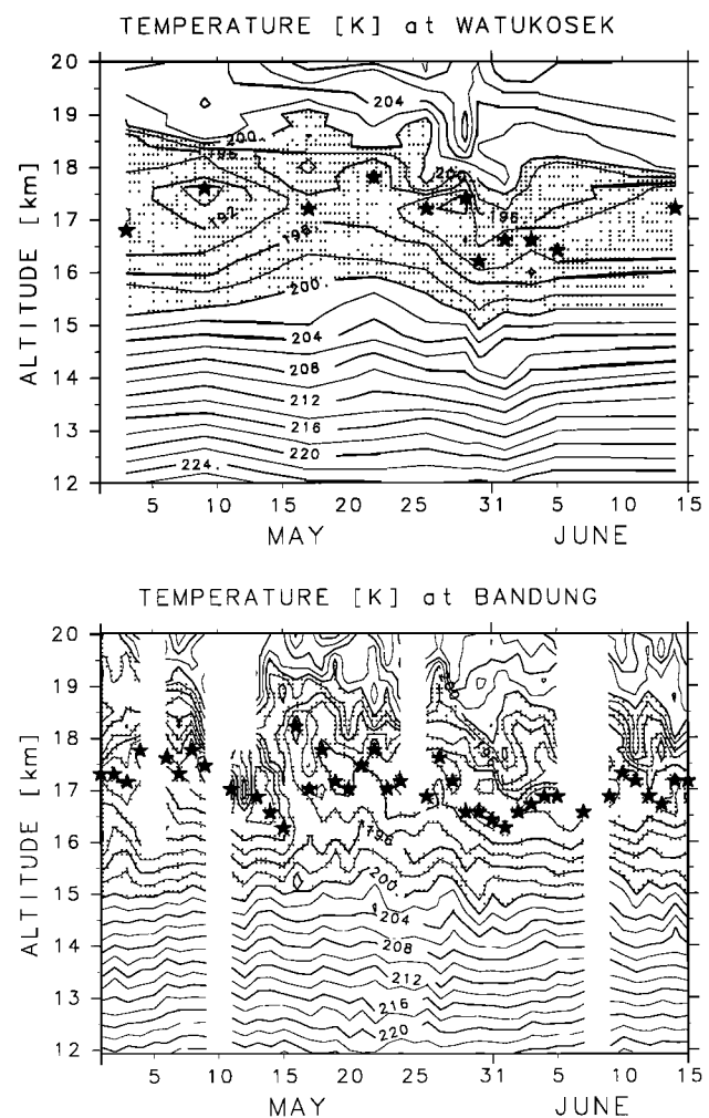
Figure 4. Variations of vertical distribution of atmospheric temperature at (top) Watukosek and (bottom) Bandung from May 1 to June 15. The contour interval is 2 K. The shaded regions correspond to those of less than 200 K. The tropopause height is also indicated at each station.
