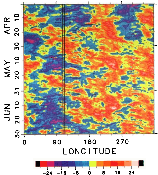
Plate 2. Variation of zonal wind along the 7.5^\circ\text{S} latitude line on the 100-hPa level ( \sim 16 \text{ km} altitude) from the GANAL data. The observational sites are indicated by lines.
