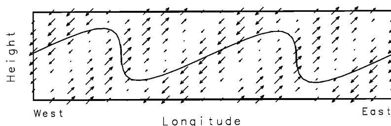
Figure 8. Schematic illustration of the wind perturbation ( u' , w' ) indicated by arrows associated with the equatorial Kelvin wave. The observer is moving eastward with the wave at the speed of c^{(x)} relative to the ground. A hypothetical air parcel moves at a velocity of (-c^+ + u', w') in this coordinate system, where c^+ \equiv c^{(x)} - \bar{u} . Its trajectory can be interpreted as the isotherm, hence the material surface, deformed by the wave. See the text for further discussions.
