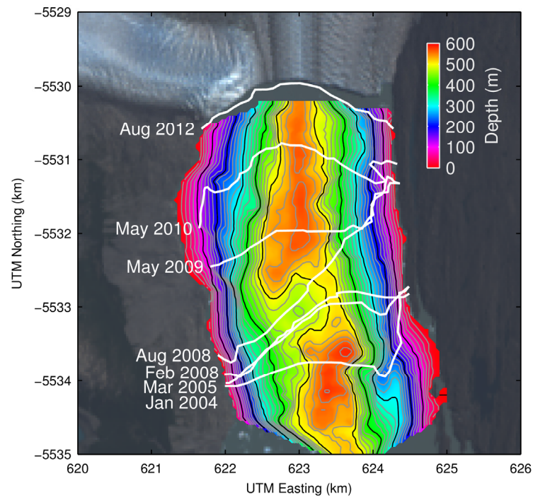
Figure 5.3. Frontal margins of Upsala Glacier and color-coded bathymetry of Brazo Upsala. Background is a Landsat 8 OLI band 8 image acquired on 12 February 2014.
