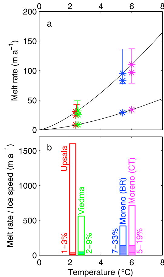
Figure 12. (a) Subaqueous melt rates estimated from water temperature measured in each lake. The asterisks were obtained from equations (2)–(4), and the ranges given by the vertical lines from equation (5) with water current assumed as 0.1–0.2 m s -1 . The upper and lower curves are melt rates computed using equations (3) and (4), respectively. (b) Ice flow speed at the glacier front (open column) compared with the estimated melt rate (shaded). The numbers indicate the ranges of proportion of the melt rates to the ice speed.
