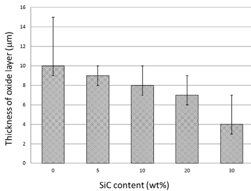
Fig. 5 Thickness of oxide layer of \text{ZrB}_2 -SiC composites after exposure to air for 12 h at 1273 K.
