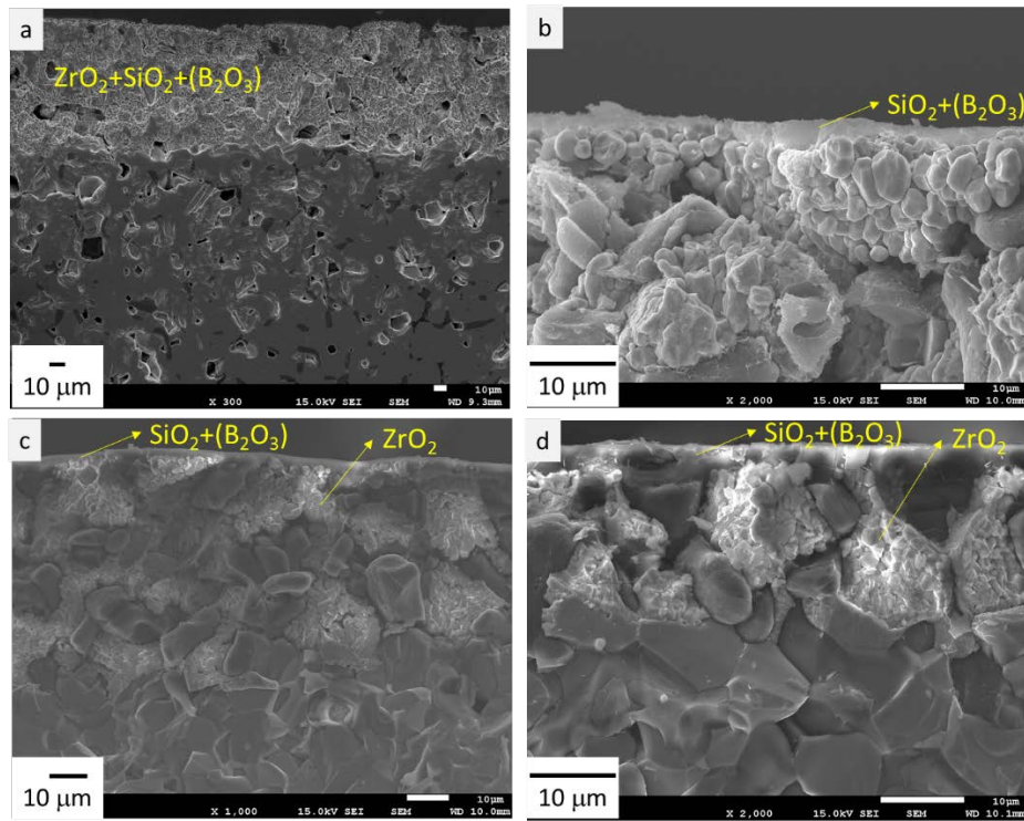
Fig. 6 SEM images of cross section of \text{ZrB}_2\text{-SiC} specimens after exposure to air for 12 h at 1473 K. (a) \text{ZrB}_2\text{-5\%SiC} ; (b) \text{ZrB}_2\text{-10\%SiC} ; (c) \text{ZrB}_2\text{-20\%SiC} ; (d) \text{ZrB}_2\text{-30\%SiC} .
