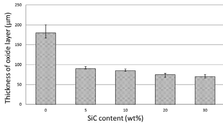
Fig. 8 Thickness of oxide layer of \text{ZrB}_2 -SiC composites after exposure to air for 12 h at 1473 K.
