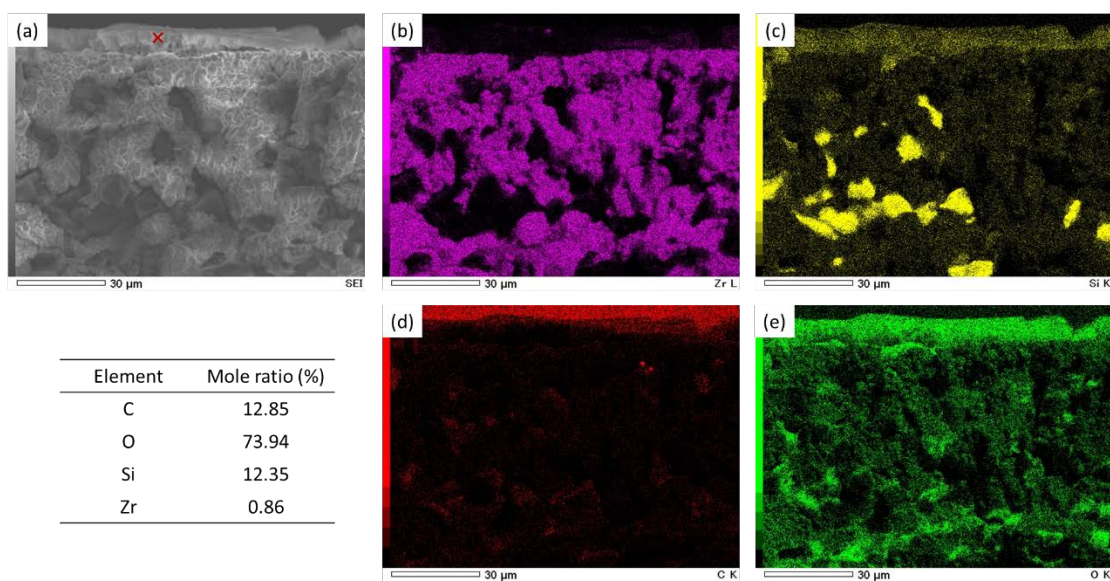
Fig. 3 EDS maps for \text{ZrB}_2 -10%SiC specimen after oxidation at 1273 K in air for 12 h. (a) SEM images of the cross section; (b) Zr map; (c) Si map; (d) C map; (e) O map. The inserted table is the analysis of the red point in (a).
