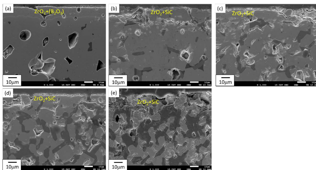
Fig. 2 SEM images of cross section of \text{ZrB}_2\text{-SiC} specimens after exposure to air for 12 h at 1273 K. (a) without SiC addition; (b) \text{ZrB}_2\text{-5\%SiC} ; (c) \text{ZrB}_2\text{-10\%SiC} ; (d) \text{ZrB}_2\text{-20\%SiC} ; (e) \text{ZrB}_2\text{-30\%SiC} .
