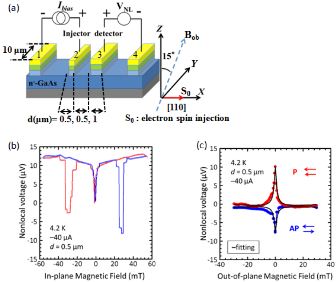
Fig. 2. (Color online) (a) Schematic structure of a four-terminal nonlocal device and circuit configuration for oblique Hanle effect measurements. (b) Spin-valve signal and (c) Hanle signals observed in GaAs with a \text{Co}_2\text{MnSi} spin source. Reprinted with permission from Ref. 17. Copyright 2013, American Physical Society.
