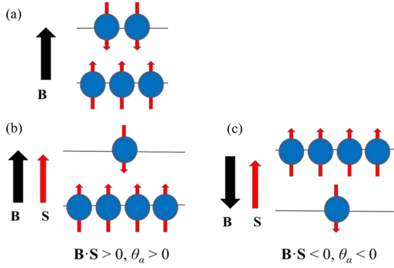
Fig. 1. (Color online) Schematic images of nuclear spin distribution (a) under an external magnetic field, (b) under the DNP process when \mathbf{B} \cdot \mathbf{S} > 0 , and (c) under the DNP process when \mathbf{B} \cdot \mathbf{S} < 0 , where \mathbf{S} is average electron spin.
