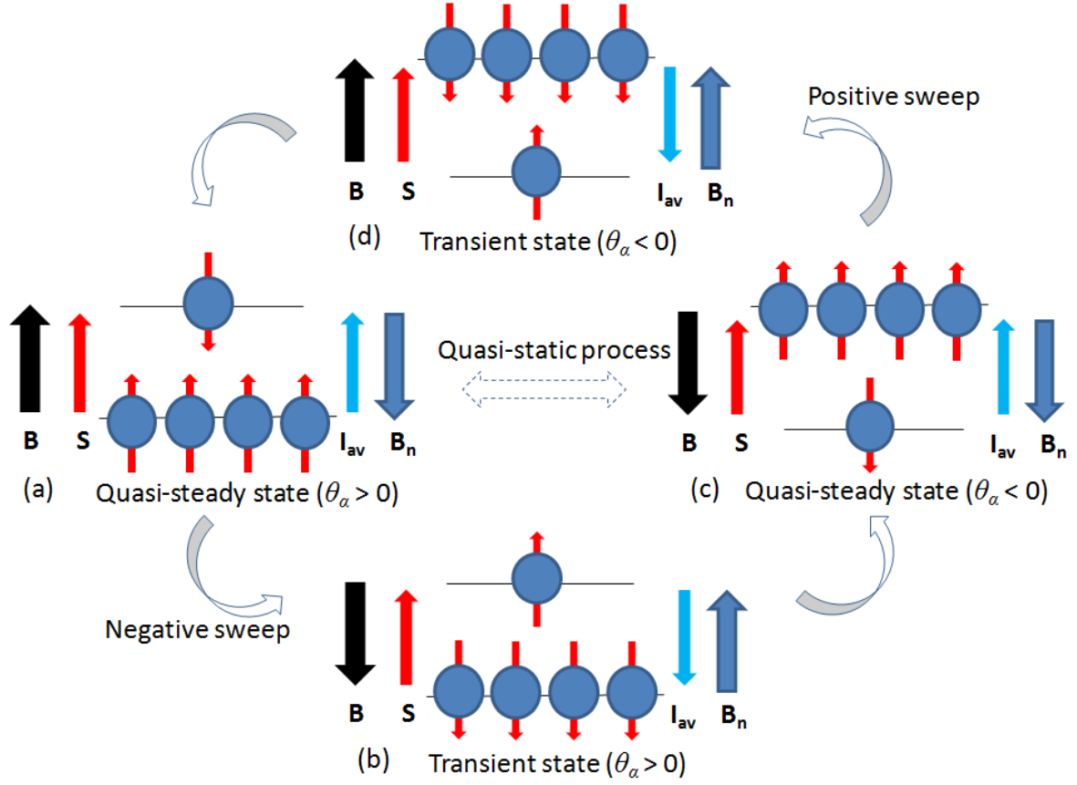
Fig. 5. (Color online) Schematic images of nuclear spin distribution of the transient oblique Hanle effect measurement for (a) state-1 and state-2, (b) state-3, (c) state-4, and (d) state-5.
