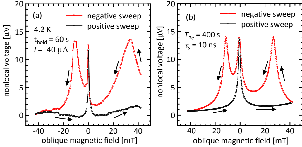
Fig. 3. (Color online) (a) Oblique Hanle signal observed in GaAs with a \text{Co}_2\text{MnSi} spin source. Reprinted with permission from Ref. 17. Copyright 2013, American Physical Society. (b) A corresponding simulation result obtained using Eqs. (1)-(7).
