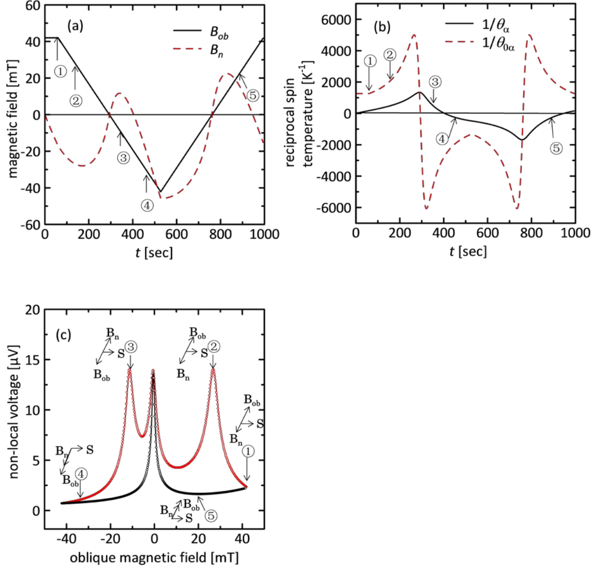
Fig. 4. (Color online) (a) Time evolution of (a) B_{ob} and B_n , (b) 1/\theta_\alpha and 1/\theta_{0\alpha} of ^{75}\text{As} isotope in GaAs. (c) A simulation result of oblique Hanle signal.
