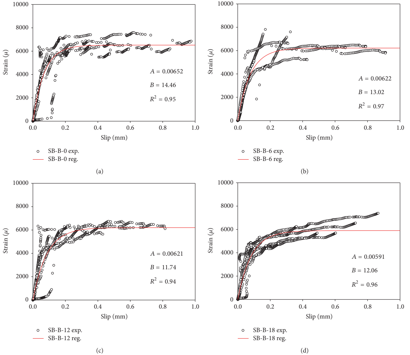
FIGURE 6: Regressed \epsilon - s curve from the experimental results for specimen SB-B.
