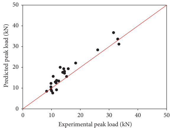
FIGURE 4: Comparison of predicted and experimental ultimate loads using Dai's method. Average ratio of predicted to experimental ultimate load = 1.12.
