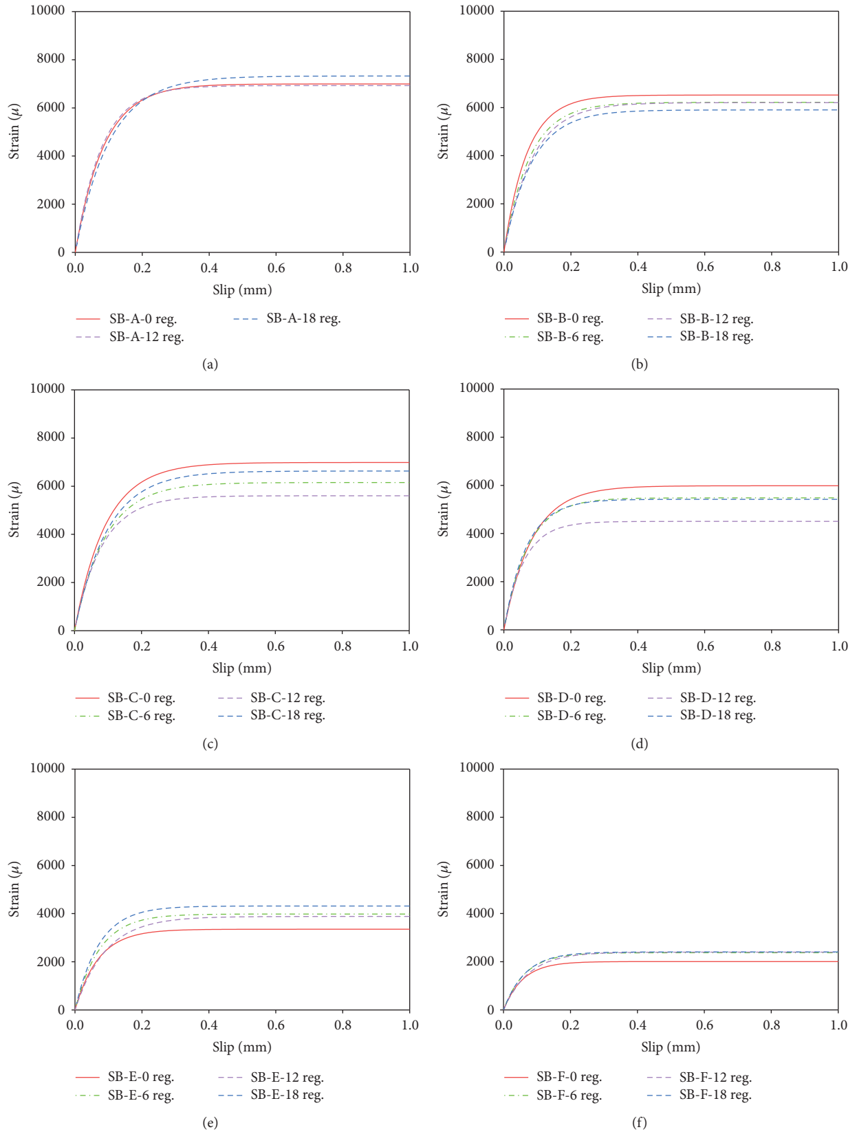
FIGURE 7: Regressed \epsilon - s curves for all the specimens.
