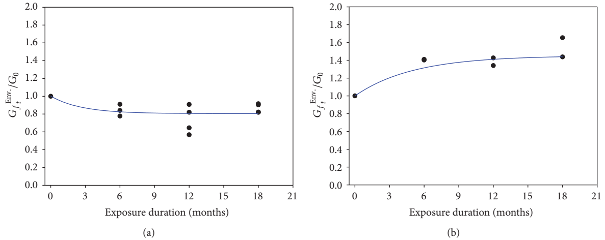
FIGURE 11: (a) Effect of exposure duration on the normalized G_f for wet-layup FRP system. G_{f_t}^{Env.}/G_f = 0.8 + 0.2e^{(-0.35t)} . (b) Effect of exposure duration on the normalized G_f for prefabricated FRP system. G_{f_t}^{Env.}/G_f = 1.45 - 0.45e^{(-0.20t)} .
