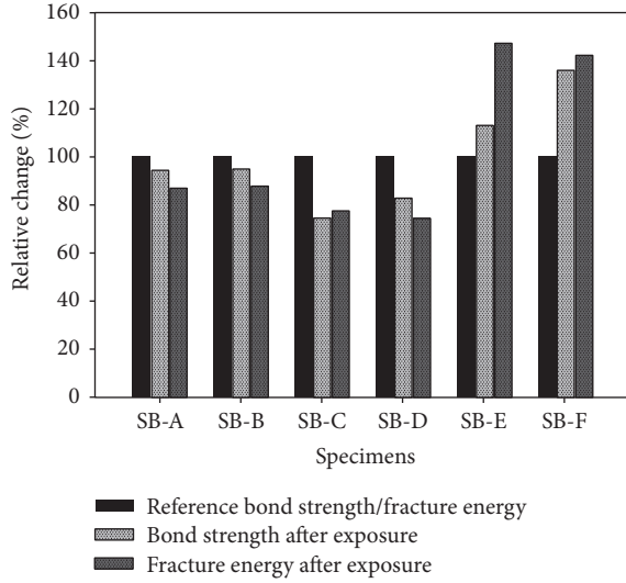
FIGURE 8: Relative change in bond strength and fracture energy after immersion.
