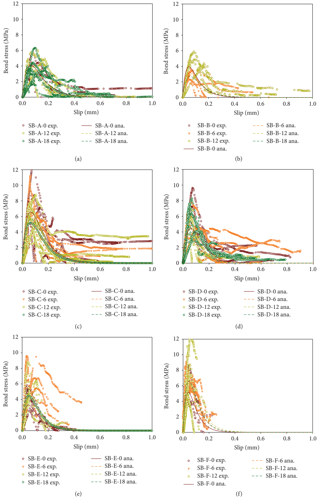
FIGURE 9: Comparison of predicted bond-slip models with the experimental data.
