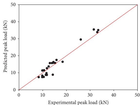
FIGURE 13: Comparison between predicted and experimental ultimate pull-out loads at 0, 6, 12, and 18 months taking all the 6 FRP systems.
