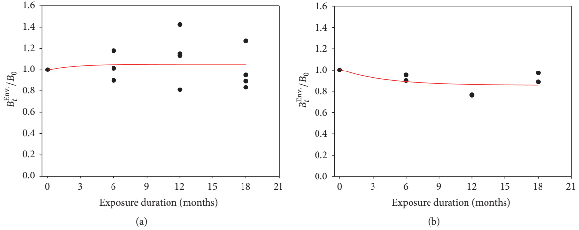
FIGURE 10: (a) Effect of exposure duration on the normalized B for wet-layup FRP system. B_t^{Env.} = B_0(1.05 - 0.05e^{-0.40t}) . (b) Effect of exposure duration on the normalized B for prefabricated FRP system. B_t^{Env.} = B_0(0.85 + 0.15e^{-0.25t}) .
