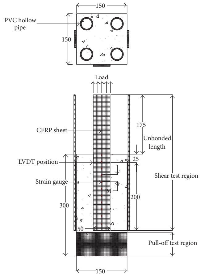
FIGURE 1: Details of bond specimen (unit: mm) for single lap shear test.
