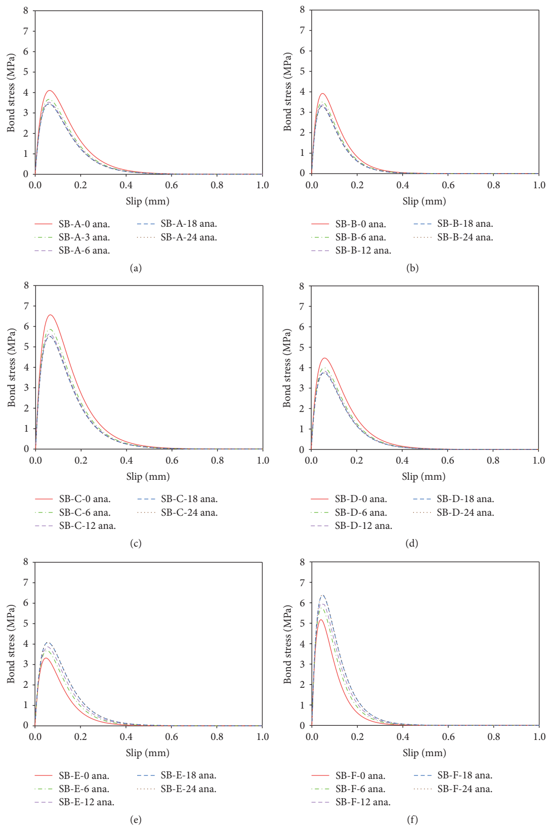
FIGURE 12: Modified bond-slip models incorporating moisture effect.
