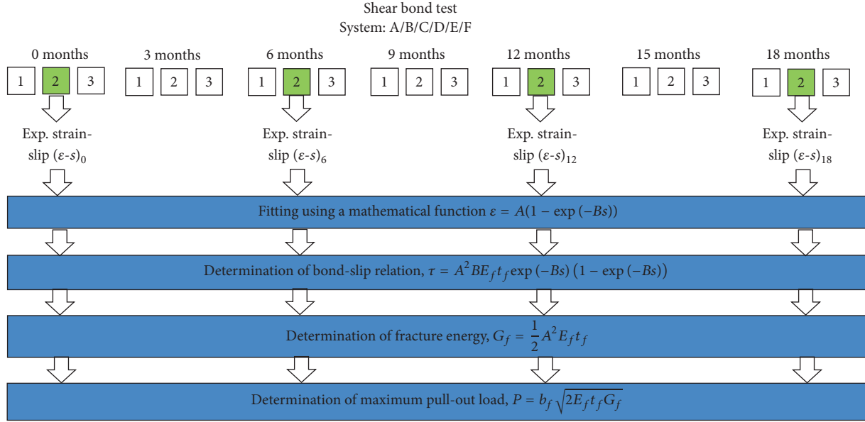
FIGURE 5: Brief procedure to determine bond-slip relations in moisture conditions.
