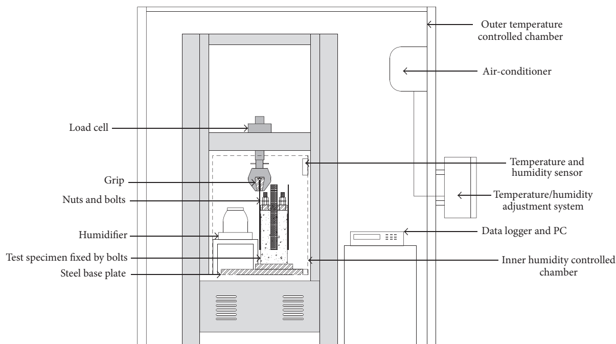
FIGURE 2: Test arrangement schematic for the bond specimen inside the environmental testing chamber.
