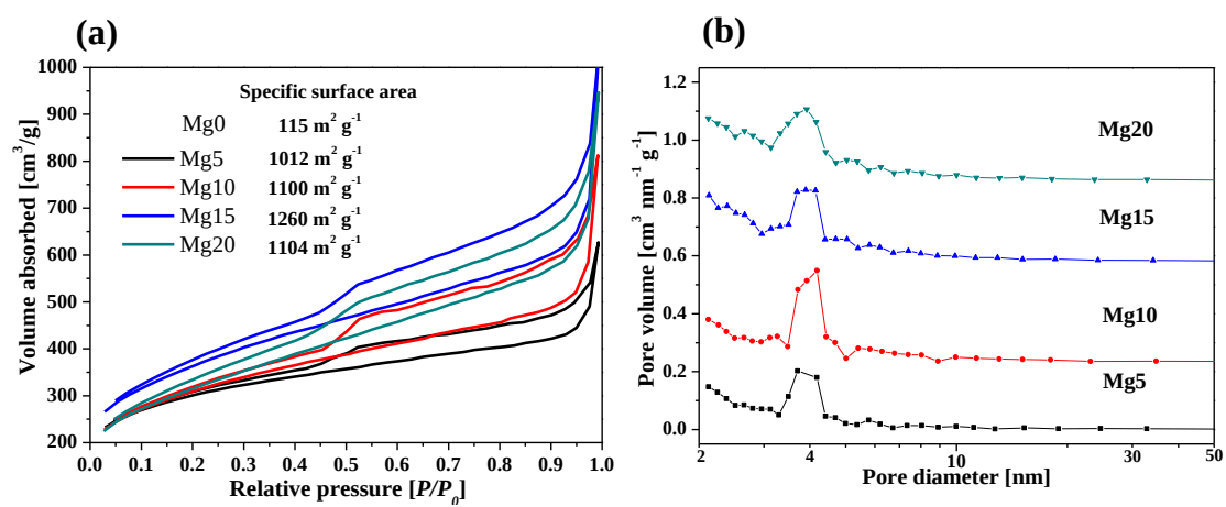
Figure 4. \text{N}_2 absorption-desorption isotherms (a) and pore size distribution (b) of the synthesized samples.
