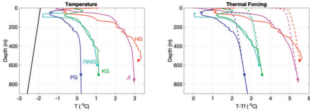
Figure 3 : Left: Temperature profiles near Greenland's largest glaciers: HG (Helheim Glacier), JI (Jakobshavn Isbrae), KG (Kangerdlugssuaq Glacier), 79NG (79 North Glacier), PG (Petermann Glacier). Black line shows freezing point temperature for constant salinity of 34.9. Right: Temperature above freezing for the 5 glaciers above for the same profile as shown in left (solid) or for a constant temperature equal to that at the grounding line depth (dashed). Squares show grounding line depths. Data described in Straneo et al. (2012).
