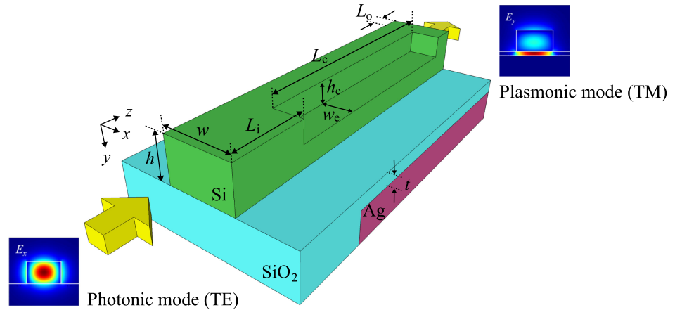
Fig. 1. Schematic of a photonic-plasmonic mode converter based on a polarization rotation. The defect is introduced at the upper corner of the silicon wire waveguide. In the converter, the photonic TE mode (left inset) is inputted and the plasmonic TM mode (right inset) is outputted.
