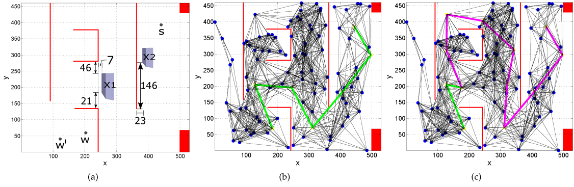
Figure 15. Experiment 4: Dynamic obstacle avoidance on SHP: (a) position of the two obstacles placed dynamically in the map; (b) initial path calculated by the PRM before dynamic obstacles were placed; (c) a new path calculated after sensing the dynamic obstacles
