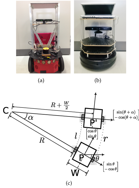
Figure 9. Robots used in the experiments: (a) Pioneer P3DX; (b) Kobuki TurtleBot; (c) motion model of two-wheeled differential drive robots
