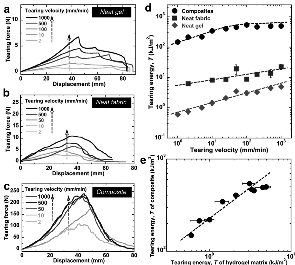
Figure 4. Tearing velocity dependent behaviors of the \text{H}_2\text{O} -equilibrated PA-GF hydrogel composite. Tearing force versus displacement curves for a) the neat gel, b) neat fabric, and c) the hydrogel composites at different tearing velocities. The sample width of both the neat fabric and composite is w = 45 \text{ mm} . d) Tearing energy, T , of the neat gel, neat fabric, and hydrogel composite versus tearing velocity. e) Tearing energy of the composite hydrogels versus the tearing energy of the hydrogel matrix, based on the above data. Dashed lines in (d) and (e) are manually drawn as visual guides.
