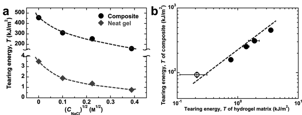
Figure 5. Tearing behaviors of the H 2 O-equilibrated PA hydrogel and PA-GF gel composites after achieving their equilibrium in NaCl solutions with different concentrations. a) Tearing energy, T , versus ionic strength, C_{\text{NaCl}}^{1/2} , for the PA gels and composites. The sample width of the composites is w = 45 mm, and the tearing velocity is 50 mm min -1 . b) Tearing energy of the hydrogel matrix versus tearing energy of the composite hydrogels for samples in different NaCl concentrations. The open circle represents the result of the as-prepared sample ( C_{\text{NaCl}} = 2.5 M) (see details in Figures S9–S11 in the Supporting Information). Dashed lines are manually drawn as visual guides.
