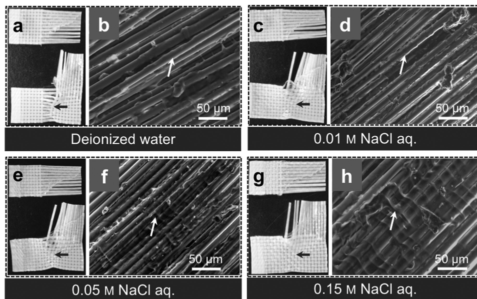
Figure 6. Macroscopic and microscopic images of the composite samples after fracture. The dark gray arrow in each image indicates the area where residual deformation is seen. As ionic strength increases, less residual deformation is present. The white arrow indicates the hydrogel matrix adhered on the fibers after the tearing test. a,b) The H 2 O-equilibrated PA-GF hydrogel composite. c–h) The PA-GF gel composites equilibrated in different saline solutions.
