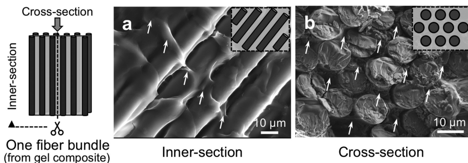
Figure 2. SEM images inside a fiber bundle of the PA-GF hydrogel composite after polymerization. To check the existence of hydrogel matrix inside the fiber bundles, one fiber bundle from the hydrogel composite was cut in two different orientations. Images were taken a) along the length of the fibers and b) of the cross-section of the fibers. The light gray color in the inserted schematics indicates the hydrogel matrix. The polymer matrix (indicated by white arrows) filled the interstitial space in the fiber bundles and connected the neighboring fibers.
