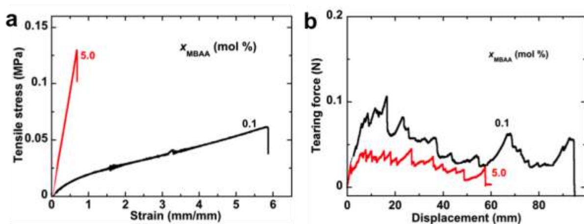
Figure S12. Tensile and tearing behaviors of as-prepared neat polyacrylamide (PAAm) hydrogels with different crosslinker (MBAA) fractions ( x_{\text{MBAA}} ) in relation to the total monomer concentration. (a) Stress-strain curves. The tensile velocity is 100 \text{ mm min}^{-1} . (b) Tearing force vs. displacement curves. The tearing velocity is 50 \text{ mm min}^{-1} . The detailed mechanical properties: (1) PAAm gel-0.10% MBAA: Young's modulus, E = 0.03 \pm 0.000 \text{ MPa} , fracture stress, \sigma = 0.08 \pm 0.021 \text{ MPa} , fracture strain, \varepsilon = 7.33 \pm 2.12 \text{ mm mm}^{-1} , and tearing energy, T = 0.06 \pm 0.01 \text{ kJ m}^{-2} ; (2) PAAm gel-5.0% MBAA: E = 0.19 \pm 0.01 \text{ MPa} , \sigma = 0.10 \pm 0.024 \text{ MPa} , \varepsilon = 0.49 \pm 0.13 \text{ mm mm}^{-1} , and T = 0.034 \pm 0.007 \text{ kJ m}^{-2} .
