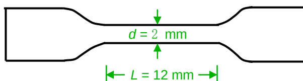
Figure S20. Geometry of the dumbbell-shaped sample for the tensile test. The neat hydrogel samples were cut into a dumbbell shape standardized as JIS-K6251-7 (2 mm in inner width, 12 mm in gauge length, and 1 ~ 2 mm in sample thickness) with a gel-cutting machine (Dumb Bell Co., Ltd.).
