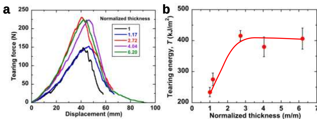
Figure S3. Tearing behavior of PA-GF hydrogel composites with different sample thicknesses. (a) The raw tearing force vs. displacement curves for the composites with different thicknesses. (b) The tearing energy vs. the normalized thickness. The sample width of all the composites is w = 45 mm, and the tearing velocity is 50 \text{ mm min}^{-1} . The thickness of hydrogel composites was tuned by changing the thickness of the silicone spacer. The normalized thickness represents the thickness of the as-prepared hydrogel composite divided by the thickness of GF ( t = \sim 0.59 mm). The critical thickness in our PA hydrogel composites appears to be \sim 3 times fabric thickness ( \sim 1.50 mm), which is smaller than the dissipation zone measured for neat PA gels ( \sim 5 mm). [5] The difference is probably due to the relatively small deformation in the z-axis (out of plane) direction due to the two-dimensional (x- and y-axes) plain structure of the fabric.
