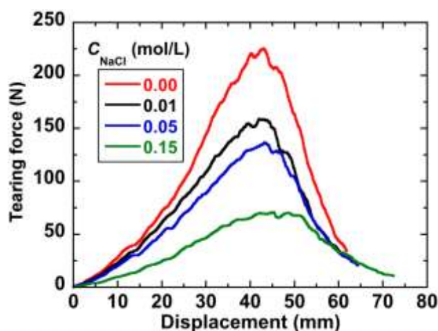
Figure S7. Tearing force vs. displacement curves of PA-GF hydrogel composites after the equilibrium in NaCl solutions with different salt concentrations. The tearing velocity is 50 mm min -1 .
