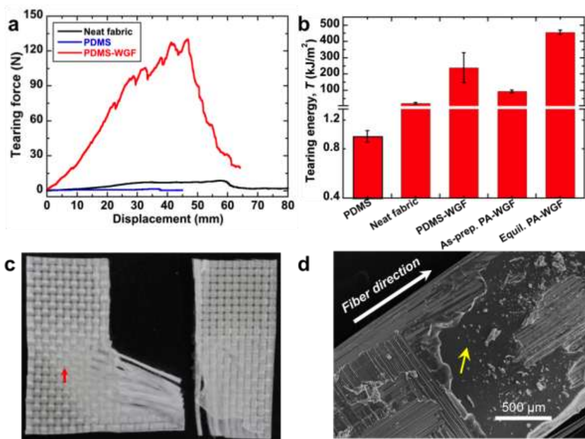
Figure S17. Tearing behavior of the PDMS-GF composite. (a) Tearing force vs. displacement curves for the neat fabric, PDMS elastomer, and PDMS-GF composite, with sample width w = 45 mm. The tearing velocity is 50 \text{ mm min}^{-1} . The thicknesses of the three groups are \sim 0.59 , \sim 1.98 , and \sim 2.00 mm, respectively. (b) Tearing energy, T , comparison of the neat fabric, PDMS elastomer, PDMS-GF composite, and as-prepared and \text{H}_2\text{O} -equilibrated PA-GF hydrogel composites. (c) Fracture image of the PDMS-GF composite. The red arrow in the macrograph indicates the area where residual deformation is seen. The composite sample shows negligible residual deformation. (d) SEM image of the PDMS-GF composite.
