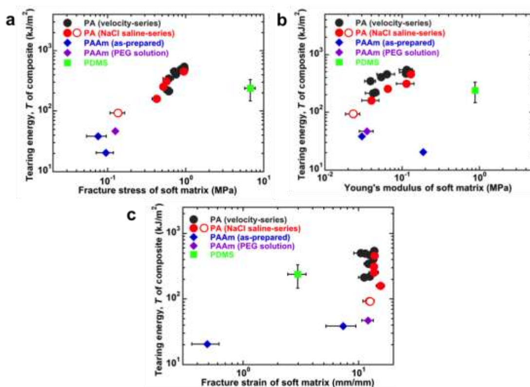
Figure S18. Tearing energy of the soft matrix-GF composite materials, T_{\text{composite}} , as a function of other mechanical properties based on different soft matrices. (a) T_{\text{composite}} vs. fracture stress of soft matrices. (b) T_{\text{composite}} vs. tensile modulus of soft matrices. (c) T_{\text{composite}} vs. fracture strain of soft matrices. In these plots, two series of polyampholyte (PA) tough hydrogels at different conditions, polyacrylamide (PAAm) weak hydrogels at different conditions, and a commercially available polydimethylsiloxane (PDMS) elastomer are utilized as soft matrices in the composites. In detail, in one series utilizing the PA hydrogel matrix (black circles, “PA (velocity series)”), the hydrogel toughness was tuned by changing the tearing velocity ranging from 1 to 1000 \text{mm min}^{-1} , based on the strong viscoelasticity of PA gels. In the other series of the PA hydrogel matrix (red circles, “PA (NaCl saline series)”), the hydrogel toughness was tuned using saline solutions with different salt concentrations (0 ~ 0.15 M), because the ionic complex in PA gel network is sensitive
