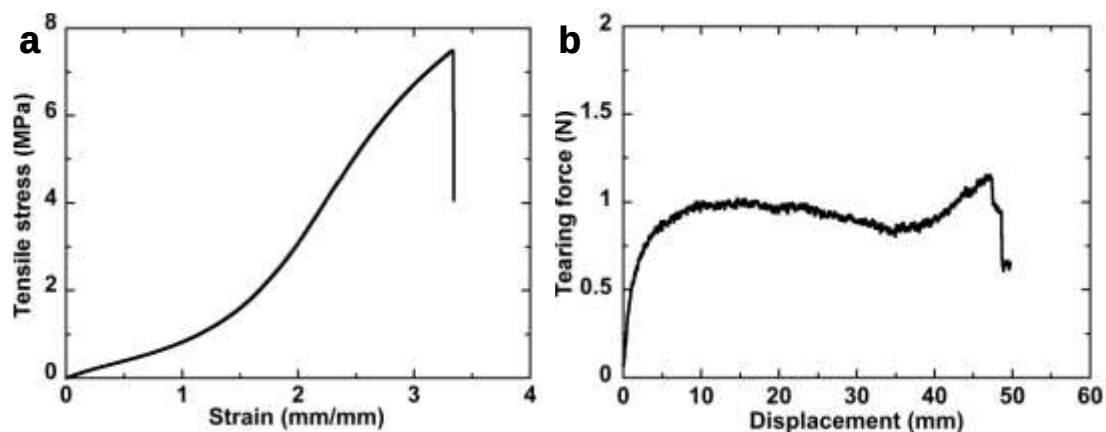
Figure S16. Tensile behavior and tearing behavior of neat PDMS elastomer. (a) Tensile stress vs. strain curve. The tensile velocity is 100 \text{ mm min}^{-1} . (b) Tearing force vs. displacement curve. The tearing velocity is 50 \text{ mm min}^{-1} . The sample thickness for the tearing test is \sim 1.98 \text{ mm} . The detailed mechanical properties of PDMS elastomer: Young's modulus, E = 0.88 \pm 0.03 \text{ MPa} , fracture stress, \sigma = 6.75 \pm 1.05 \text{ MPa} , fracture strain, \varepsilon = 2.97 \pm 0.53 \text{ mm mm}^{-1} , and tearing energy, T = 0.96 \pm 0.08 \text{ kJ m}^{-2} .
