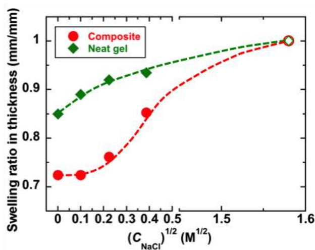
Figure S8. Swelling ratio (in thickness direction) vs. C_{\text{NaCl}}^{1/2} , for the PA hydrogel and the PA-GF gel composites. Here the swelling ratio is normalized by the thickness of their as-prepared samples. The open symbols represent the results of the as-prepared samples (salt concentration: 2.5 M). Dashed lines are manually drawn as visual guides.
