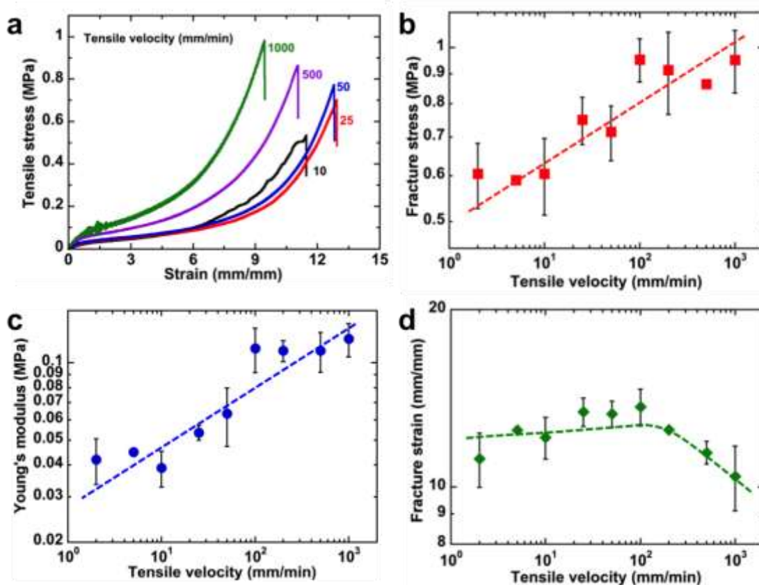
Figure S4. Tensile velocity dependent behaviors of neat H 2 O-equilibrated polyampholyte (PA) hydrogels. (a) Stress-strain curves; (b) Fracture stress; (c) Young's modulus; (d) Fracture strain. The initial gauge length of dumbbell-shaped sample is 12 mm. Dashed lines in (b), (c), and (d) are manually drawn as visual guides.
