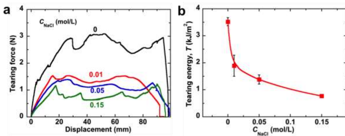
Figure S6. Tearing behavior of neat PA hydrogels after achieving the equilibrium in NaCl solutions with different salt concentrations. (a) Tearing force vs. displacement curves; (b) Tearing energy, T , vs. salt concentration, C_{\text{NaCl}} . The tearing velocity is 50 mm min -1 .
