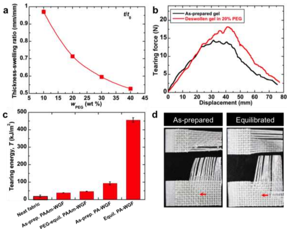
Figure S15. Tearing behavior of deswollen PAAm-GF hydrogel composite in concentrated poly(ethylene glycol) ( M_w = 20,000 ) solutions. (a) Swelling ratio (in thickness direction) of the composite hydrogel in PEG solutions with different concentrations. (b) Tearing force vs. displacement curves for the as-prepared hydrogel composite and deswollen hydrogel composite in 20 wt% PEG solution, with w = 45 mm. Here 20 wt% PEG solution was used to deswell the PAAm-GF hydrogel composite for achieving the similar deswelling ratio (in thickness direction) as that of PA-GF hydrogel composite. The tearing velocity is 50 \text{ mm min}^{-1} . (c) Tearing energy, T , of the above two groups and as-prepared as well as \text{H}_2\text{O} -equilibrated PA-GF hydrogel composites. (d) Fracture images of the composite hydrogel samples based on the above two groups. The red arrow in each graph indicates the area where residual deformation is seen. Both of the two samples show no sign of residual deformation.
