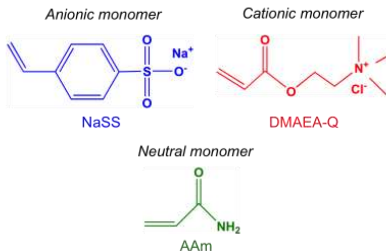
Figure S1. Chemical structures of the monomers used in this work. NaSS: sodium p -styrenesulfonate, DMAEA-Q: dimethylaminoethylacrylate quaternized ammonium, AAm: acrylamide.
