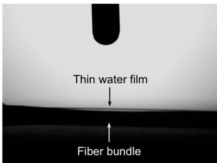
Figure S2. Photograph of a contact angle test in air. When a water droplet is placed on a glass fiber bundle, it immediately wets the hydrophilic glass fibers [1–4] and penetrates into the fiber bundle due to the capillary effect (indicated by the thin water film). Owing to this feature, the precursor solution of PA hydrogel can excellently penetrate into the fiber bundle to form a composite with good interfacial contact.
