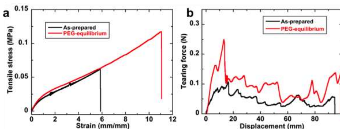
Figure S14. Tensile and tearing behaviors of as-prepared neat PAAm hydrogel and the PAAm hydrogel equilibrated in 20 wt% PEG solution. (a) Tensile stress vs. strain curves.
