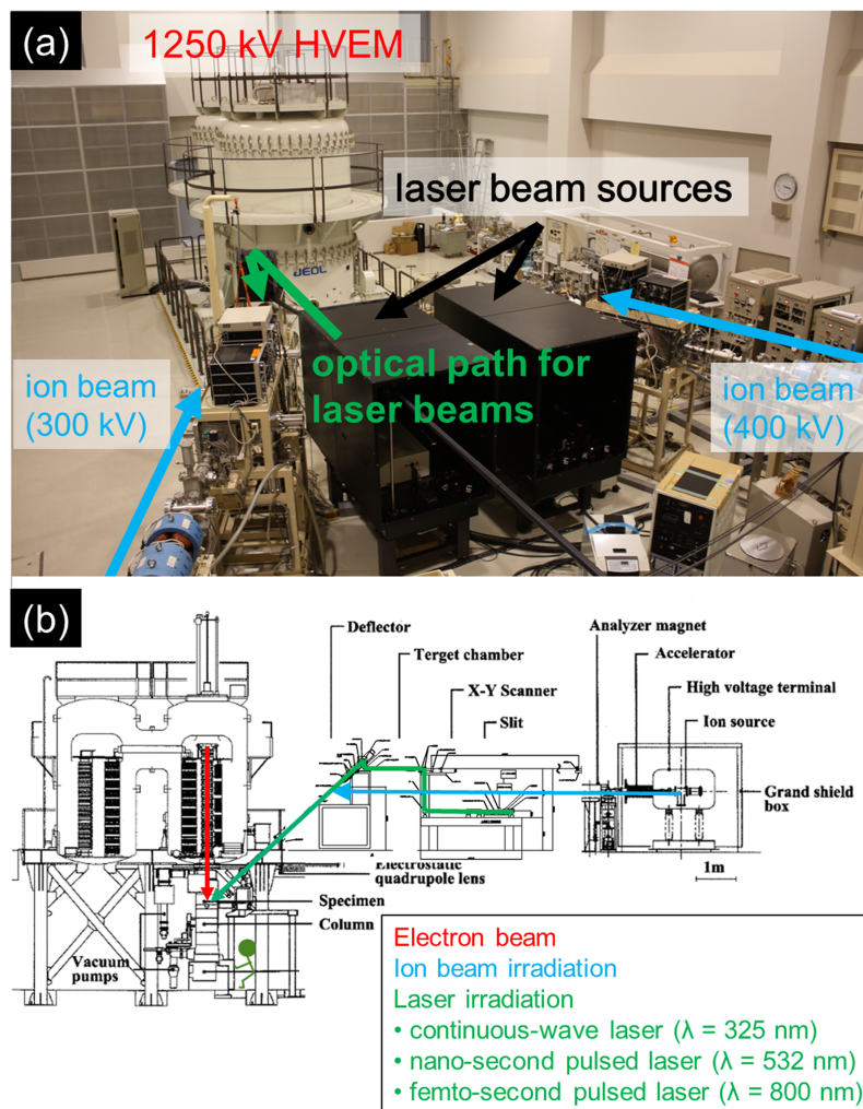
FIG. 1. Multi-quantum-beam high-voltage electron microscope (MQB-HVEM). (a) A photo of the upper half of the MQB-HVEM, including the electron accelerator, ion-beam lines, and optical systems, for which three laser sources can be selected. (b) A cross-sectional schematic of the MQB-HVEM, showing the three beam lines.
