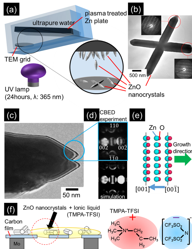
FIG. 3. Sample preparation via submerged photosynthesis of crystallites (SPSC), 19 and characterization of generated ZnO crystals by using 200 kV transmitted electron microscopy (TEM). (a) Schematic of ZnO crystal deposition and regrowth on a TEM grid. (b) TEM image of a ZnO nanocrystal with a twin structure along [1\bar{1}0] . (c) TEM image of the tip of a ZnO crystal with a pencil-like shape. (d) Convergent-beam electron diffraction (CBED) pattern obtained from the edge of the crystal shown in (c) and a numerically simulated pattern for a crystal with a thickness of 50 nm. (e) Atomic arrangement near a crystal tip, derived from CBED patterns. (f) Schematic of the observable area of ZnO crystals covered with TPMA-TFSI ionic liquid on a thin holey carbon film.
