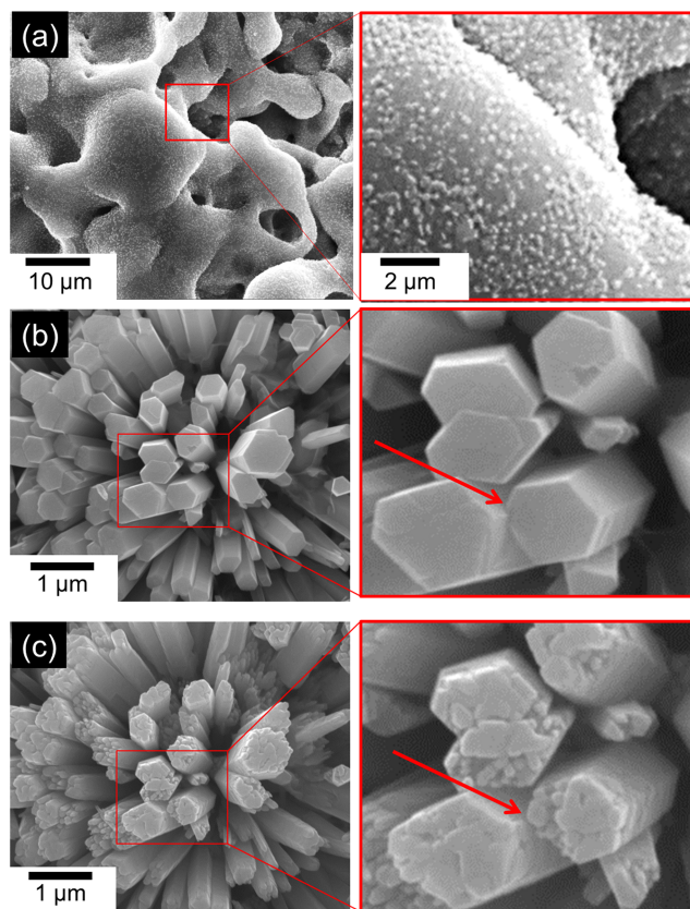
FIG. 2. Seeding, growth, and photocorrosion of ZnO nanocrystals. (a) Scanning electron microscopy (SEM) images of the plasma-treated Zn substrate, showing many nanoparticles embedded in its molten surface. (b) SEM images of typical ZnO nanoflowers, which were grown in ultrapure water irradiated by UV ( \lambda = 365 nm) light for 72 h. (c) SEM images of corroded ZnO nanoflowers, which were UV-irradiated in fresh, ultrapure water by the same experimental setup.
