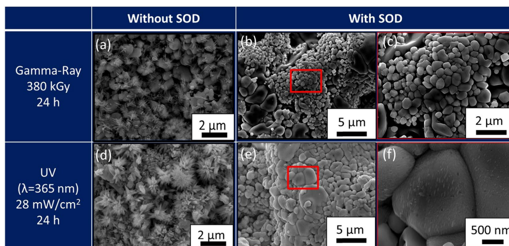
Figure 9. SOD addition test. FE-SEM images of the surface after irradiation of (a) 24 hours at 380 kGy gamma-rays without SOD in ultrapure water. (b) 380 kGy gamma-rays irradiation with SOD in ultrapure water. (c) Enlarged view of rectangle area in (b). (d) UV irradiation for 24 hours. (e) UV irradiation for 24 hours with the addition of SOD. (f) Enlarged view of rectangle in (e).
