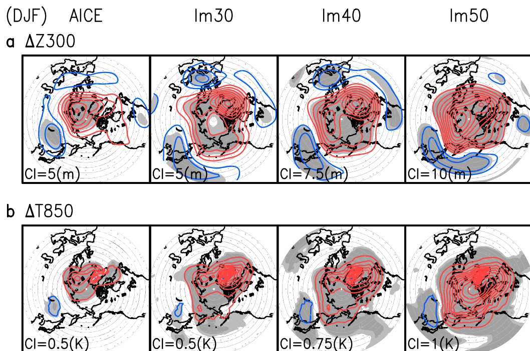
Figure 1. Differences in the 150 year average of the (a) geopotential height at 300 hPa (m) and (b) temperature at 850 hPa (K) in December-January-February. Anomalies of (from left to right) AICE, Im30, Im40, and Im50 runs from the CNTL run are shown. A positive (negative) anomaly is indicated by red (blue) contours. The zero line is omitted and the contour interval is displayed at the bottom left corner of the plot. Statistical significance greater than 95% and 99% are indicated by light and heavy gray shading, respectively. CNTL, high ice period, 1979–1983; AICE, low ice period, 2005–2009; Im30, Im40, and Im50: decrease of 30, 40, and 50 cm, respectively, from the CNTL.
