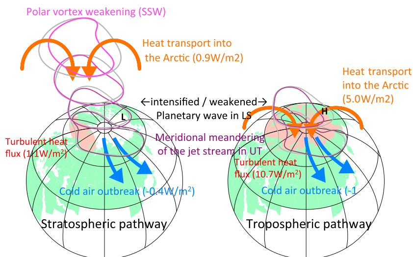
Figure 4. Schematic diagram of the two physical processes connecting Arctic sea ice loss and a negative Arctic Oscillation (AO)-like response. (left) The stratospheric pathway corresponding to the AICE case in January. (right) The tropospheric pathway corresponding to NDJFM Im50 case. Typical characteristics of the circumpolar jet stream at 10, 30, 100, and 300 hPa (only 100 and 300 hPa in the right plot) corresponding to the high and low sea ice cases are shown by gray and purple lines, respectively. Anomalous atmospheric heating due to associated meridional circulation changes (see sections 3.3, S2, and S6) and the turbulent heat flux are given in units of \text{W m}^{-2} . SSW, sudden stratospheric warming; LS, lower stratosphere; UT, upper troposphere.
