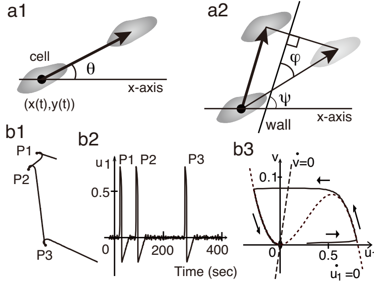
Figure 2: Schematic illustration of mathematical description of swimming motion for free swimming (a1) and when in contact with the vessel wall (a2). Simulation of normal free swimming in the case of an excitable u_1 (b1-b3). (b1) Typical trajectory of swimming. (b2) Time course of u_1 . The noise-induced spikes P1 , P2 and P3 correspond to the turning events P1 , P2 and P3 , respectively, in (b1). (b3) A typical trajectory of a spike in the state space of u_1 and v . The solid line is the solution trajectory, and the dotted and the dashed lines are the null clines for u_1 and v , respectively.
