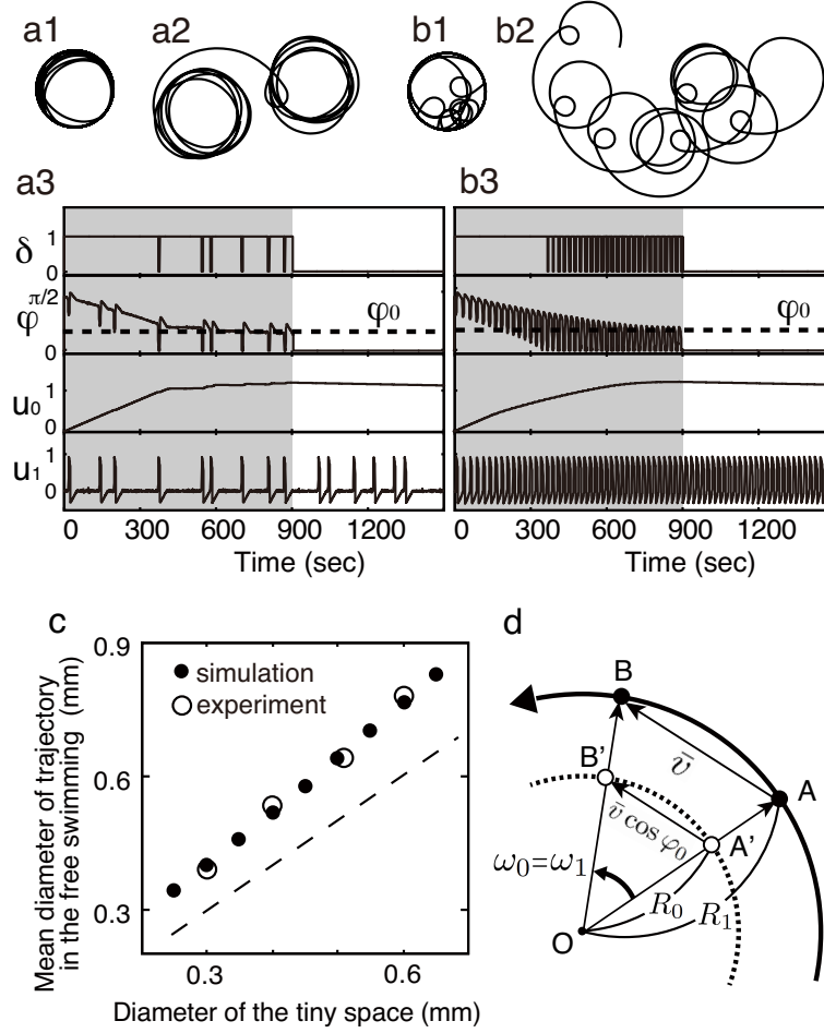
Figure 3: Mathematical modeling for swimming behaviour during and after confinement. Numerical simulations in case of excitable u_1 ( I = 0.0 )(a1-a3) and in case of oscillatory u_1 ( I = 0.15 )(b1-b3). Trajectories during (a1, b1) and after (a2, b2) the confinement. Time courses of key variables (a3, b3) and the confinement ended at time 900. The parameters for both cases were as follows: vessel size = 0.2\text{mm} , \bar{v} = 0.3\text{mm/sec} , \varepsilon = 0.0001 , s = 0.003 , \tau_u = 0.0025 , \tau_v = 20 , a_1 = -0.3 , a_2 = -1 , a_3 = 4 , b_0 = 1 , b_1 = 5 , \varphi_0 = 40^\circ , and \xi_{u_1}, \xi_v \in [-0.25, 0.25] . Figures 3a1, 3a2, 3b1 and 3b2 are drawn to the same scale. (c) Simulated relationship between the diameter of the confined space and that of the circular trajectory just after confinement. The dashed line indicates where the two diameters are equal. All parameters were the same as Fig.3c. (d) Schematic illustration of geometrical analysis of the relationship between the two diameters. See the main text for details.
