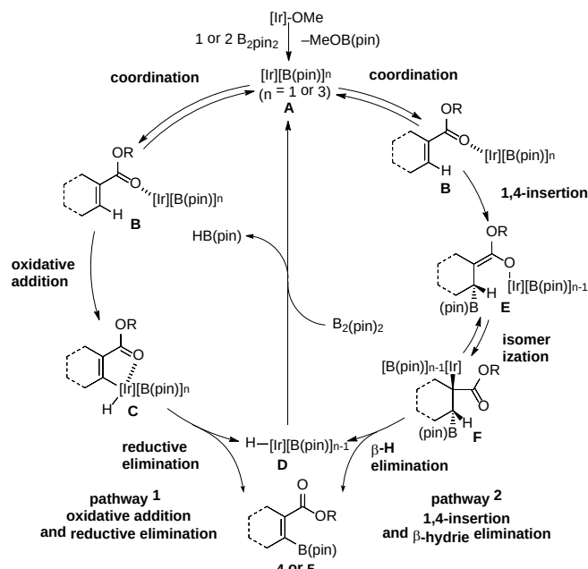
Scheme 3. Proposed mechanism.
