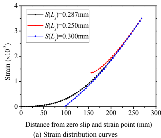
Fig. 5 Strain and slip distribution curves.
