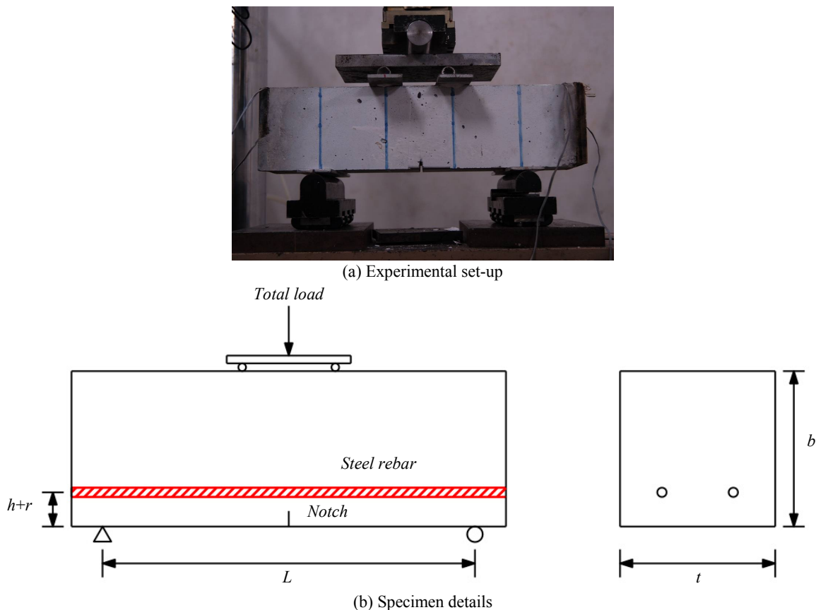
Fig. 7 Experimental set-up and specimen details.
