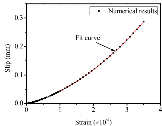
Fig. 6 Strain vs slip relation.
