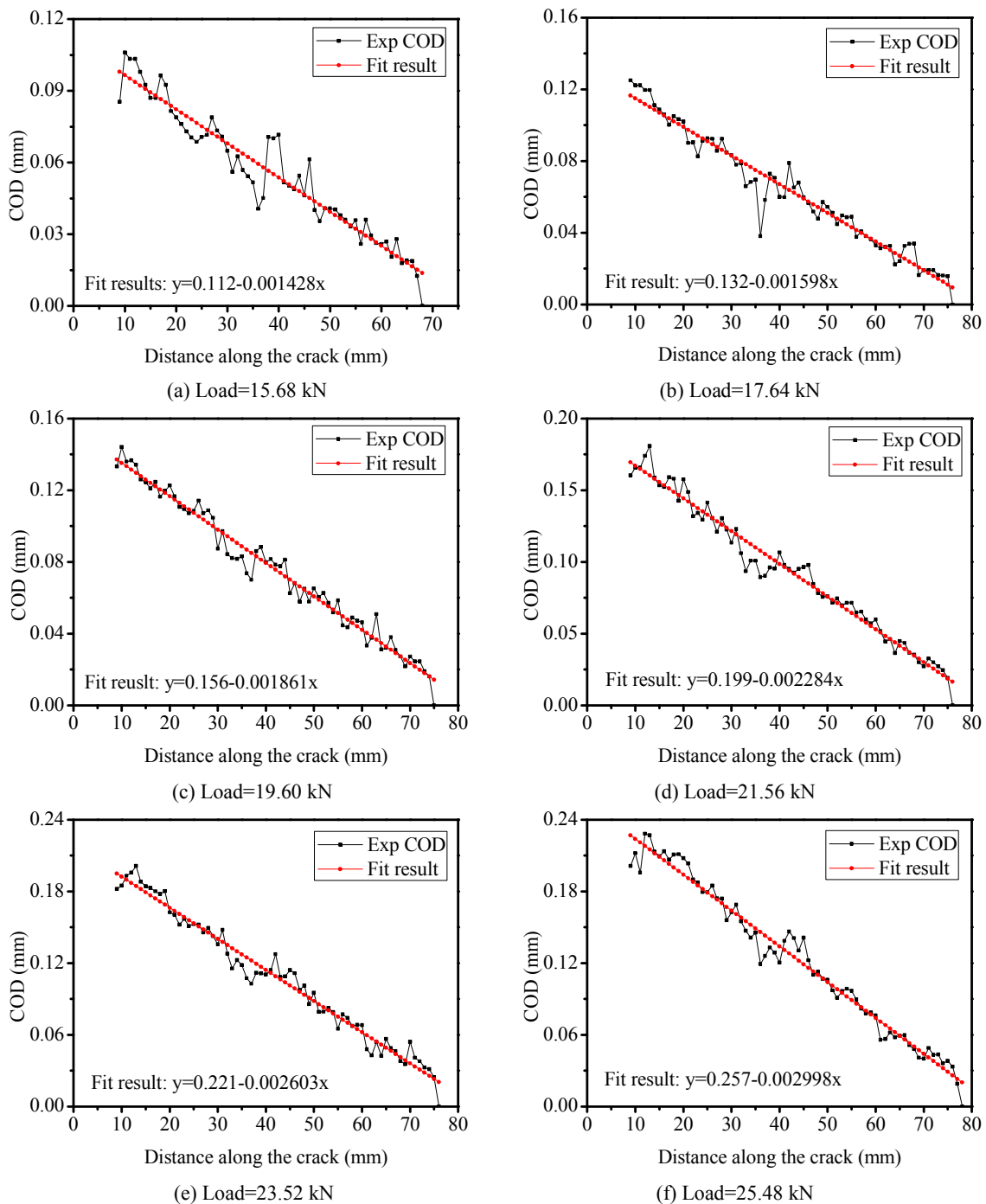
Fig. 9 Experiment COD profiles of an RC beam under static loads.
