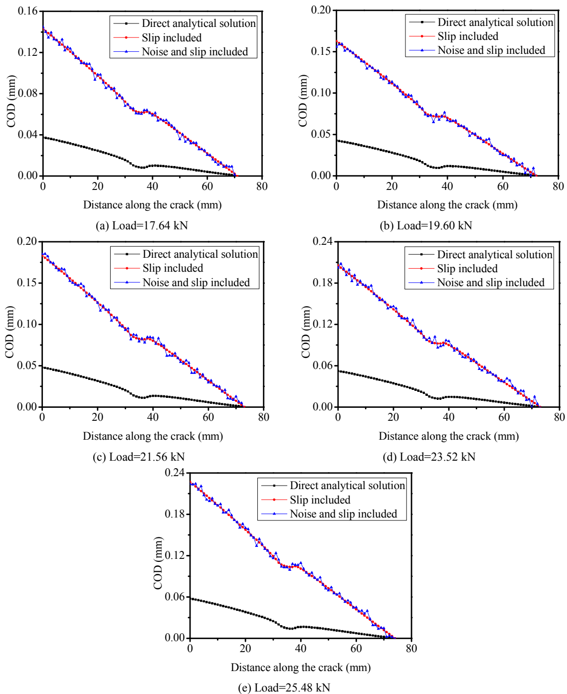
Fig. 8 Analytical COD profiles of an RC beam under static loads.
