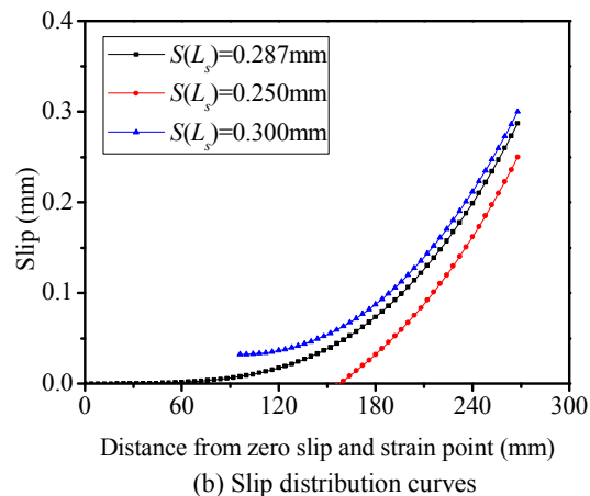
Fig. 5 Strain and slip distribution curves.
