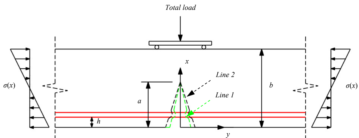
Fig. 1 Schematic diagram for the understanding of cracking process.
