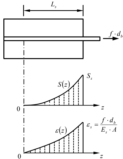
Fig. 2 Bond slip and rebar strain along rebar.
