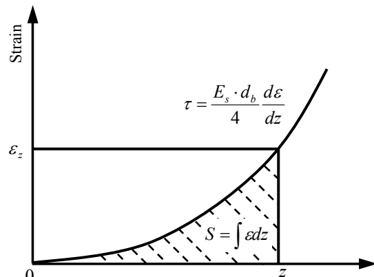
Fig. 4 Relation between rebar strain, bond stress and bond slip.
