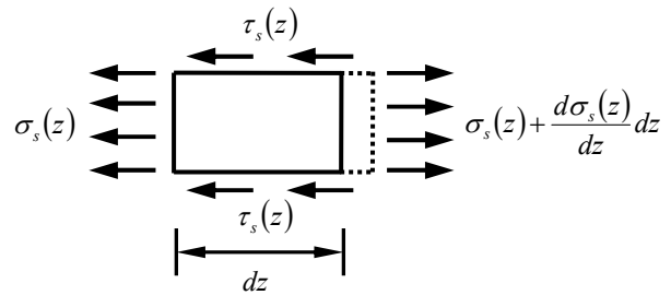
Fig. 3 Stresses acting on rebar element.
