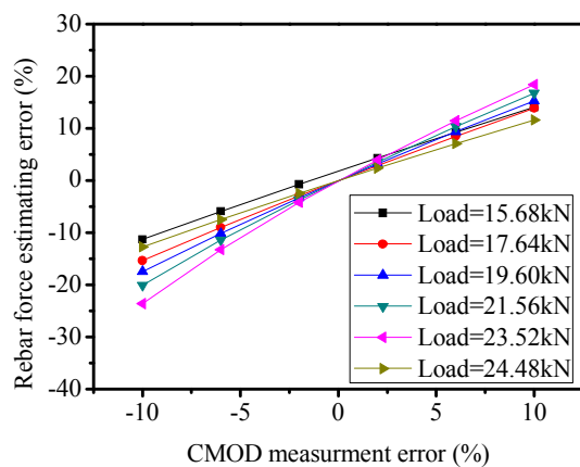
Fig. 10 Sensitivity study of CMOD measurement error.
