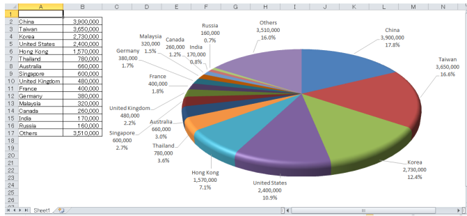
Fig. 12. Example of pie chart and corresponding table. Although pie chart displays percentages, they are not shown in table.
