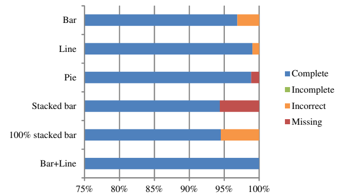
Fig. 15. Errors in cell values in aggregated tables for different types of charts
