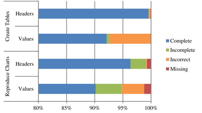
Fig. 9. Percentages for different types of errors in worker tables
