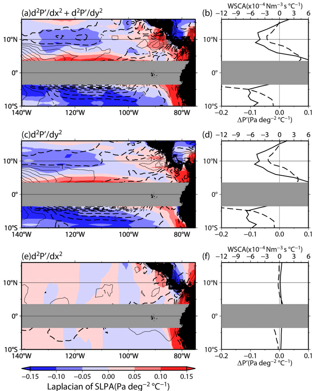
FIG. 9. (a) Regression map of Laplacian of SLPA (color, \text{Pa deg}^{-2} \text{°C}^{-1} ) and WSCAs (contours, dashed line for negative and solid line for positive with 2.0 \times 10^{-4} \text{ Nm}^{-3} \text{ s °C}^{-1} intervals) onto Niño-3.4 index. Laplacian of SLPA is smoothed with Gaussian filter with an e -folding scale of 3^\circ \times 3^\circ . (b) Meridional plots of these two variables zonally averaged over 135^\circ\text{--}110^\circ\text{W} (solid line for SLPA and dashed line for WSCA). Figs. 9c and 9d and Figs. 9e and 9f show regressed anomalies using only \partial^2(\text{SLPA})/\partial y^2 and -\partial(\tau^x/f)/\partial y and \partial^2(\text{SLPA})/\partial x^2 and \partial(\tau^y/f)/\partial x , respectively. Equatorial area at 3^\circ\text{S--}3^\circ\text{N} is masked by gray due to small Coriolis parameter.
