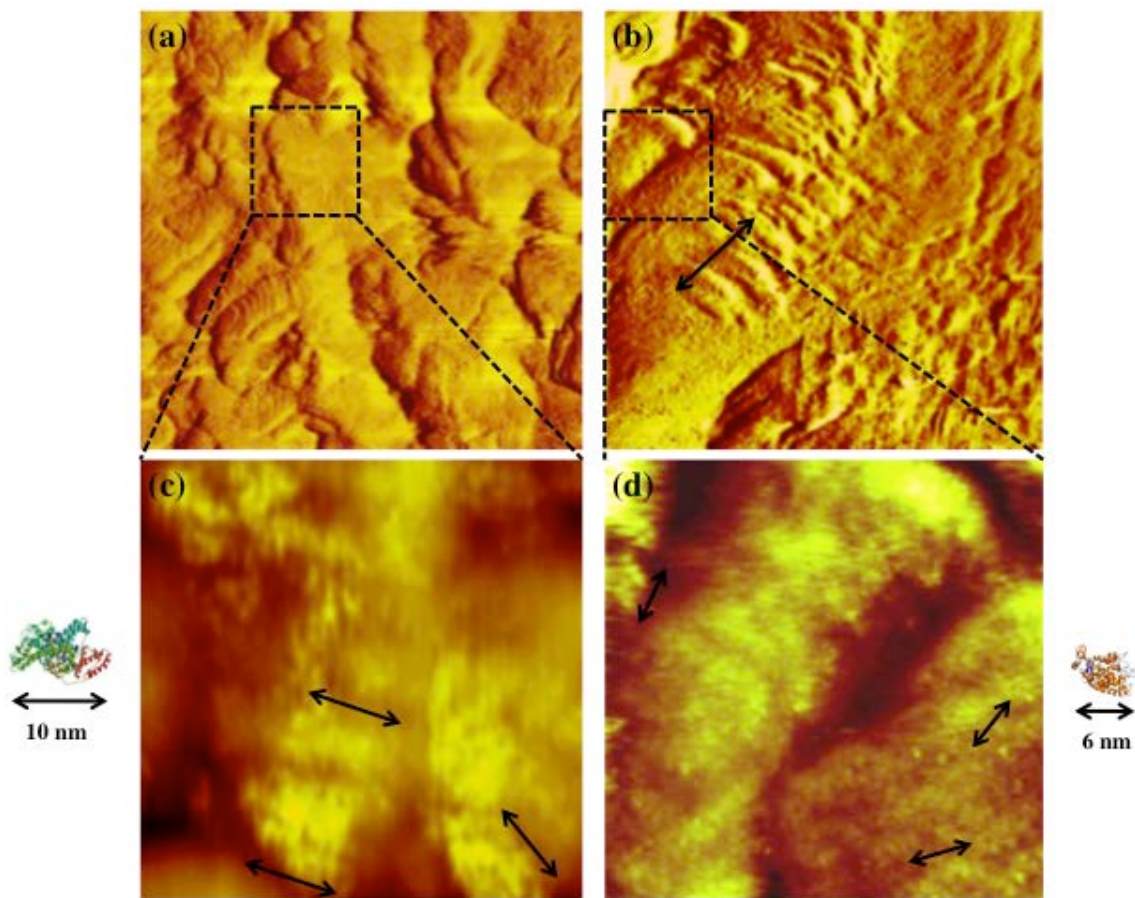
Fig. 5. STM images of a 200 nm × 200 nm area of the sensor surface: (a) ractopamine–BSA conjugate sensor surface, and (b) salbutamol–HRP conjugate sensor surface. STM images of a 50 nm × 50 nm area of the sensor surface: (c) ractopamine–BSA conjugate sensor surface, and (d) salbutamol–HRP conjugate sensor surface.
