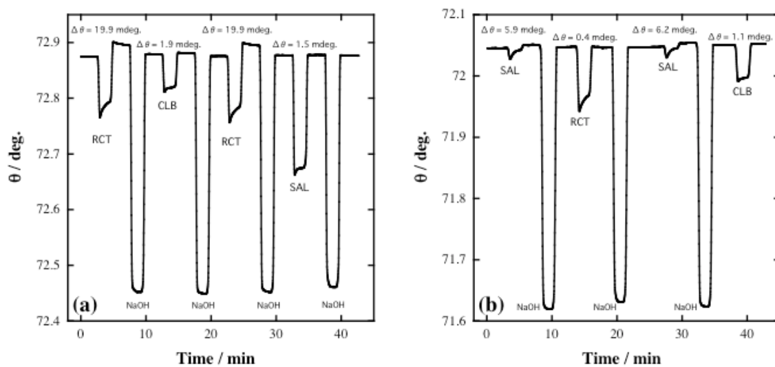
Fig. S1. Selectivity study of \beta -agonist sensor surfaces by multiple antibodies injection on: (a) RCT sensor surface and (b) SAL sensor surface.
