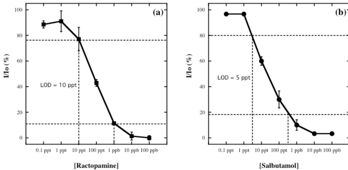
Fig. 3. Sigmoid curves of \beta -agonists solution concentration dependence obtained using the indirect competitive inhibition immunoassay. The inhibition rate was calculated from the angle shift in the presence ( I )/absence ( I_0 ) of \beta -agonists. In the premixing process, \beta -agonists Ab was mixed with a series of antigen concentrations. The incubation time was 2 min.
