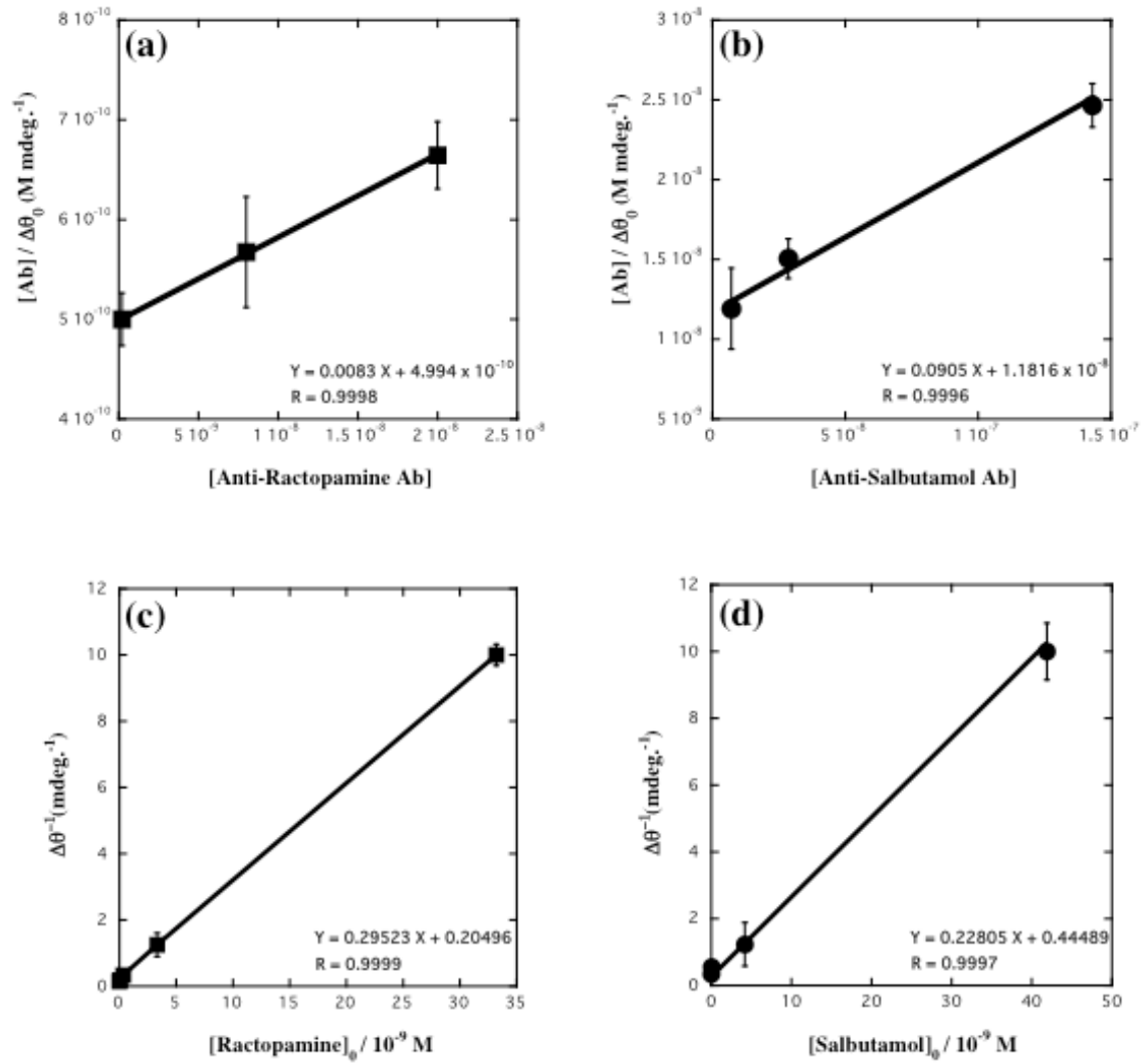
Fig. 4. Kinetic study of the \beta -agonists detection. Ab concentration dependence for (a) ractopamine and (b) salbutamol. Antigen concentration dependence for (c) ractopamine and (d) salbutamol.
