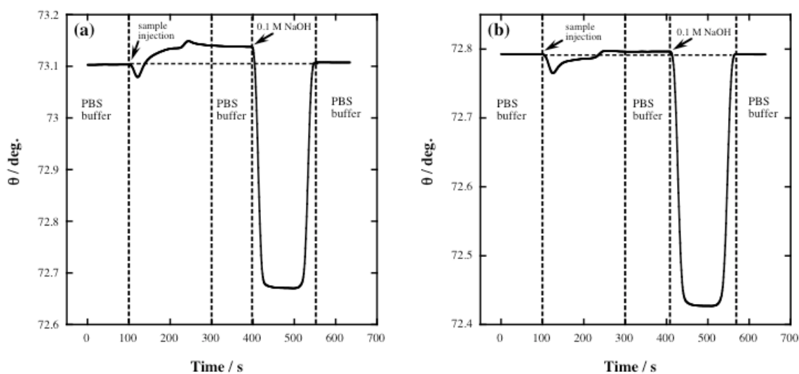
Fig. 2. SPR sensorgrams of the detection of (a) ractopamine and (b) salbutamol. The flow rate was 100 \mu\text{L}\cdot\text{min}^{-1} , PBS (10% ethanol) solution was used as the running solution, and 0.1 M NaOH aqueous solution was used to regenerate the sensor surface.
