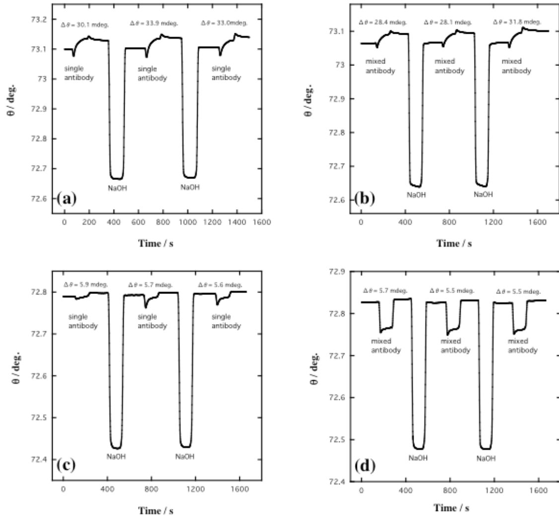
Fig. 6. Selectivity study of \beta -agonist antibodies: RCT sensor surface against RCT Ab in the (a) absence and (b) presence of SAL Ab and CLB Ab; SAL sensor surface against SAL Ab in the (c) absence and (d) presence of RCT Ab and CLB Ab.
