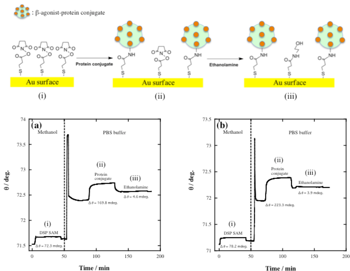
Fig. 1. SPR sensorgram of the fabrication of the sensor surface: (i) self-assembly of the succinimidyl-terminated propanethiol monolayer, (ii) immobilization of the \beta -agonistprotein conjugates (ractopamine–BSA and salbutamol–HRP), and (iii) blocking of the unreacted succinimidyl-terminated propanethiol with ethanolamine.
