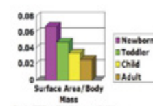
Figure 2. Ratio of surface area to body mass in children and adults. (In color in Annuals online.)
