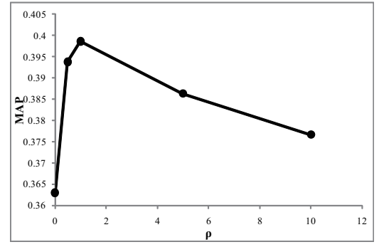
Figure 9: MAP of each \rho for the proposed method.
