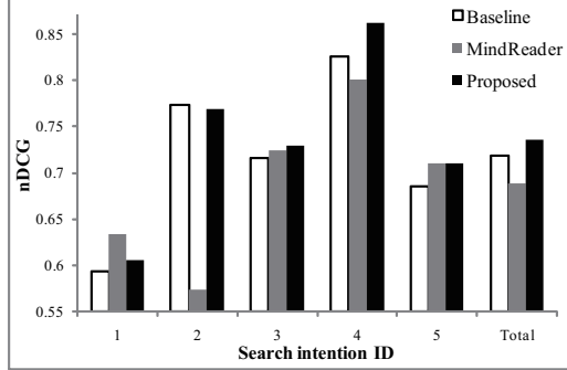
Figure 10: nDCG for the proposed method and the baselines.
