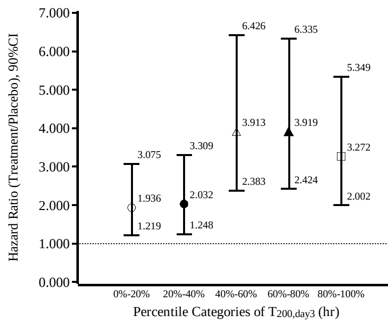
Figure 2-1- 2 Hazard ratio for comparison with placebo by the percentile categories: T 200,day3
