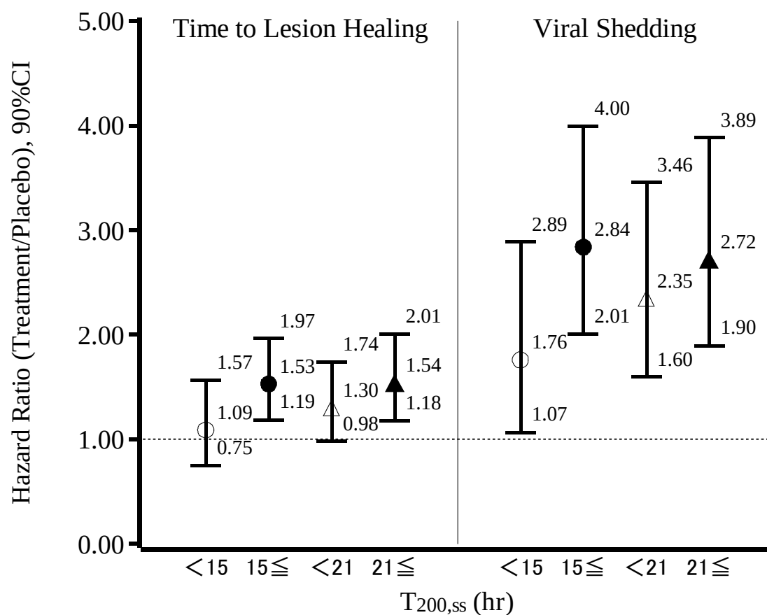
Figure 2-1- 3 Hazard ratio for comparison with placebo by the time categories: T_{200,ss}
