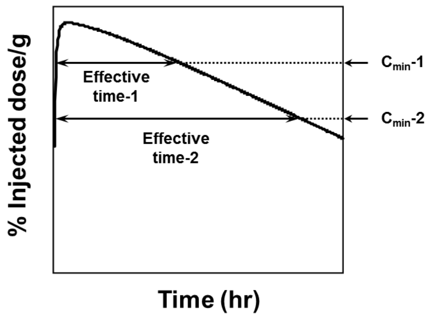
Figure 1- 2 Pharmacokinetic model of ECyd and scheme of description of C_{min} and effective time
