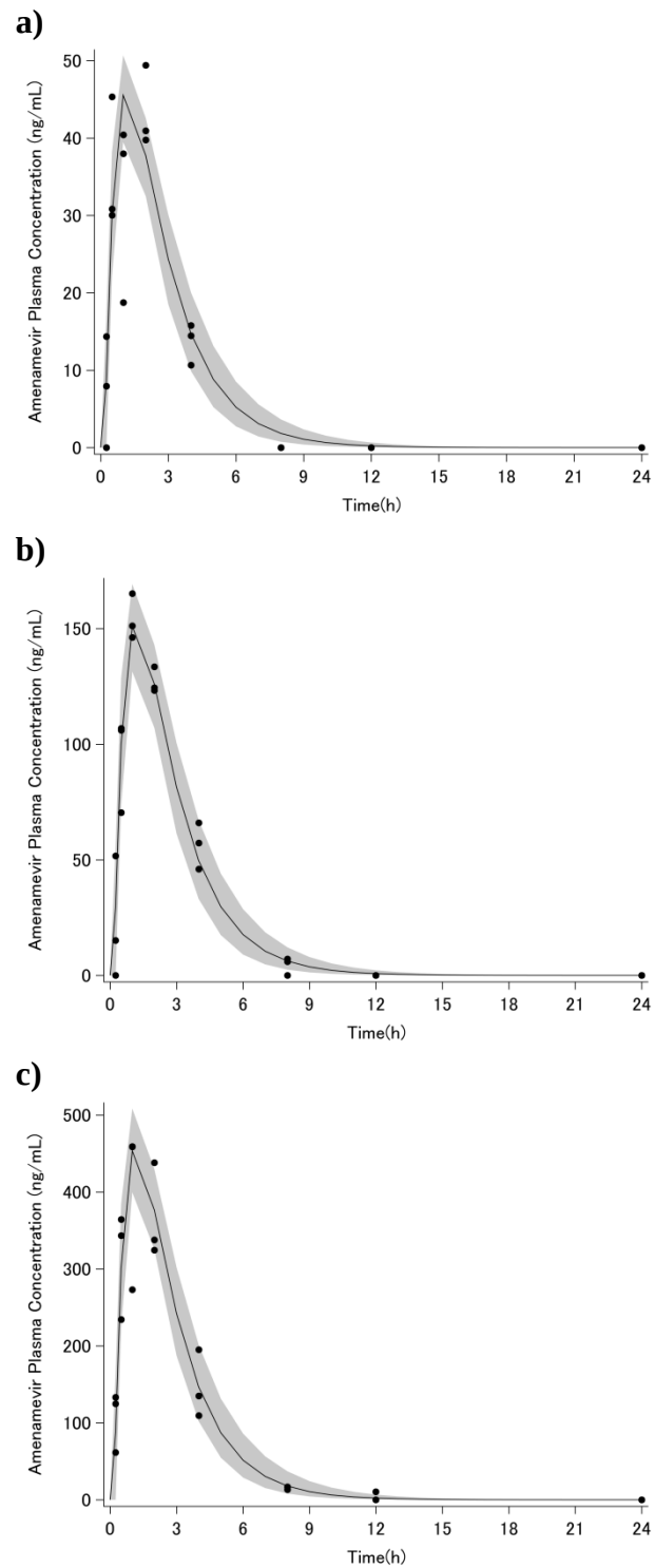
Figure 2-2- 3 Results of population PK modeling and visual predictive check in guinea pigs
