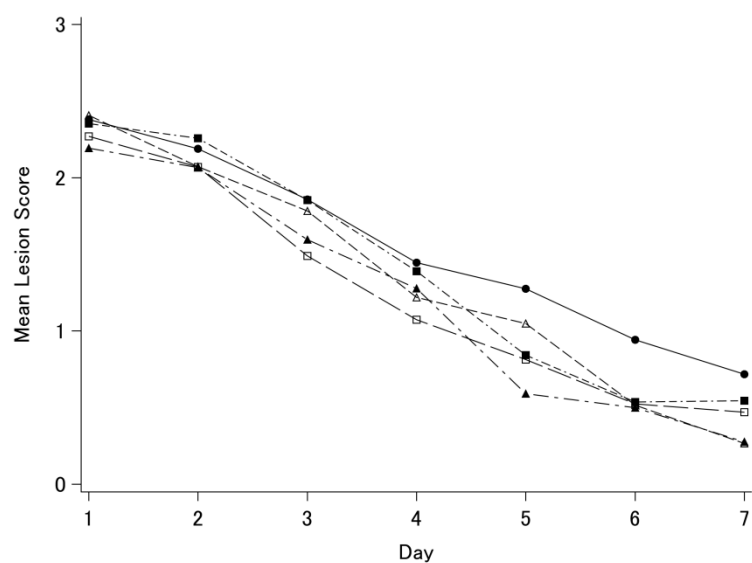
Figure 2-2- 1 Time course profiles of mean observed lesion scores in guinea pigs (a) and humans (b)
