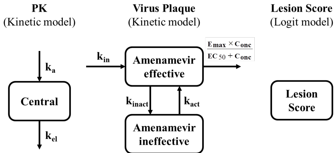
Figure 2-2- 2 Overview of the PK/PD model
