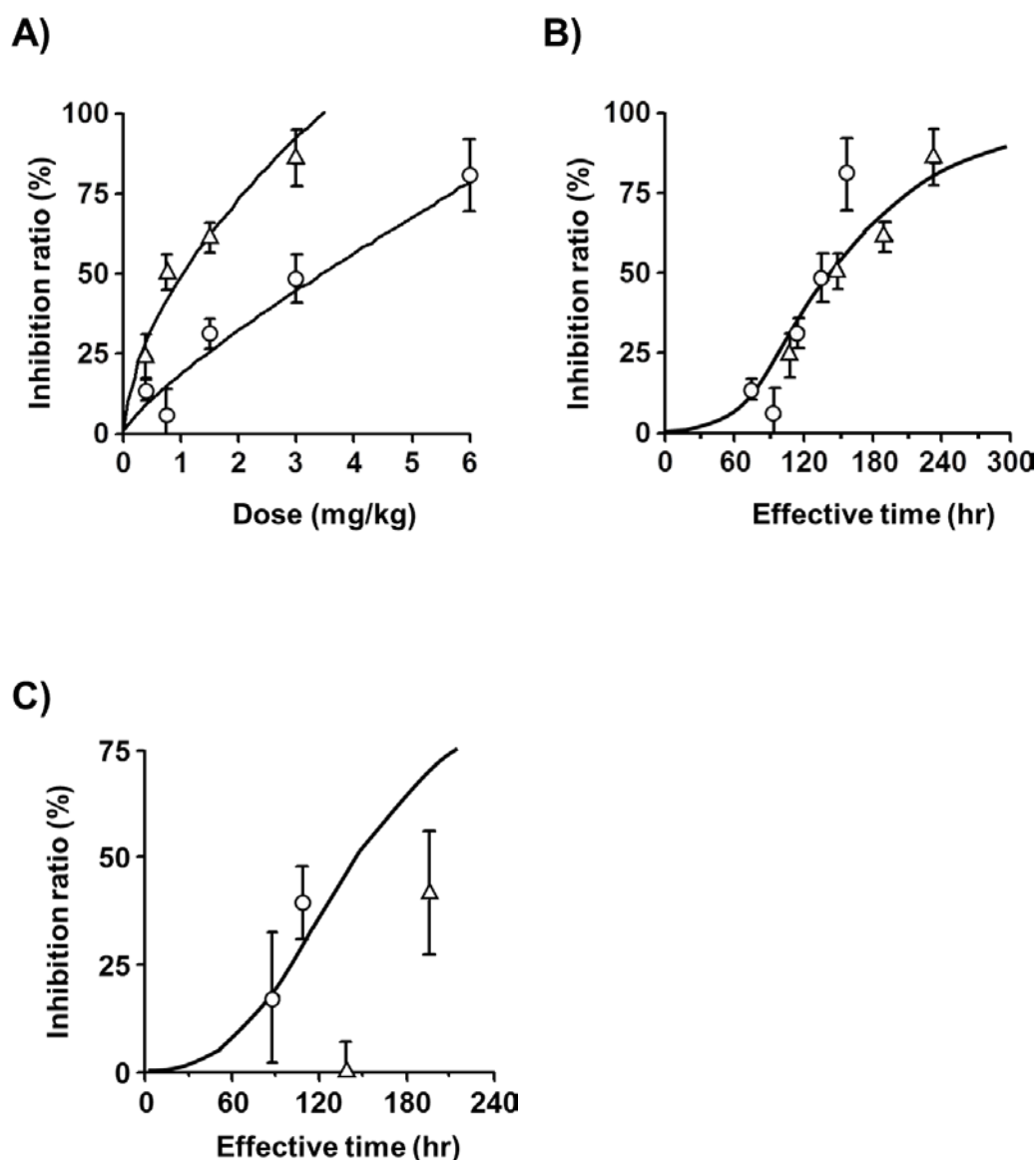
Figure 1-4 Relationships between administration dose / effective time and IR
