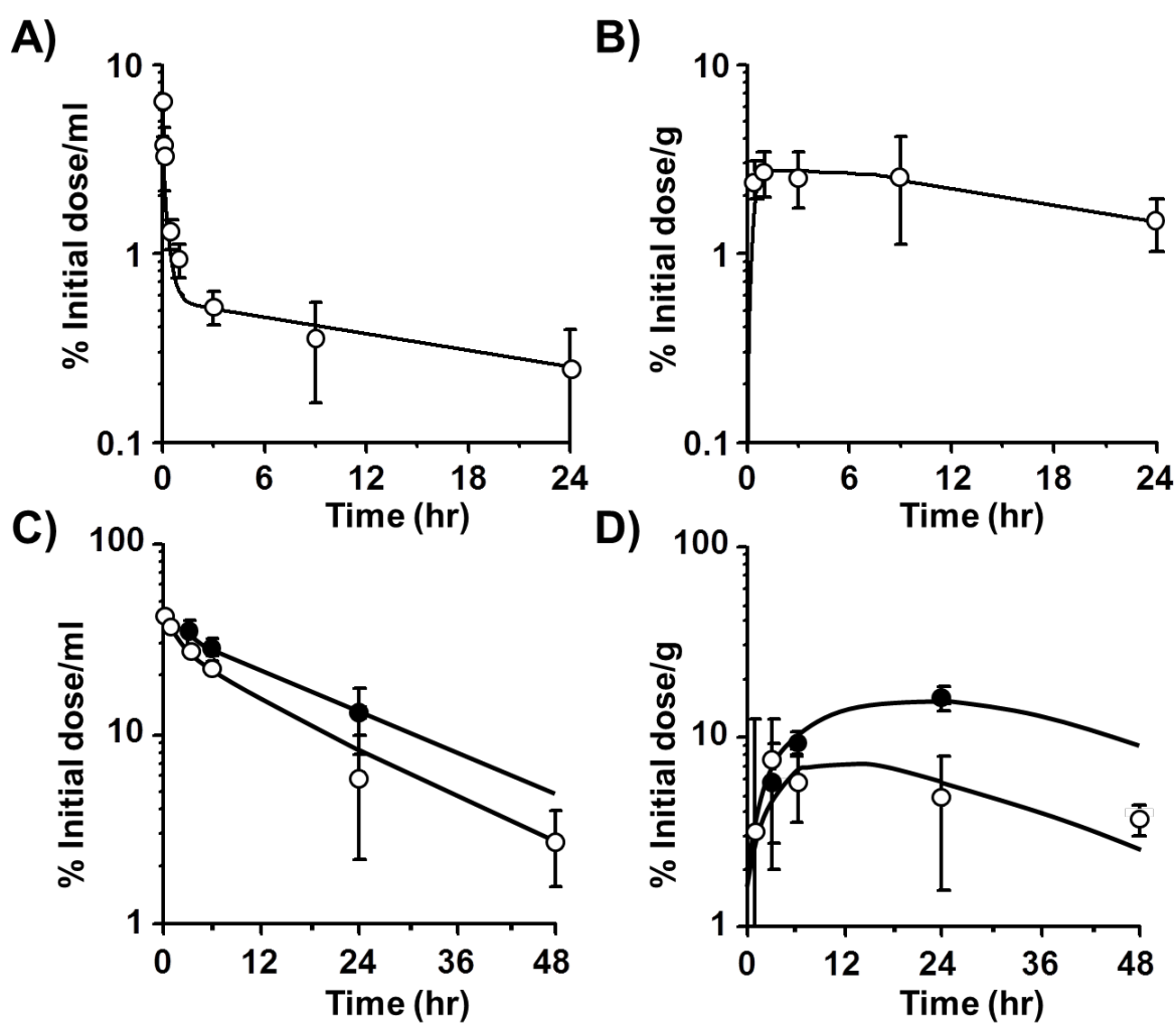
Figure 1-3 Concentration-time profile of ECyd and liposome
