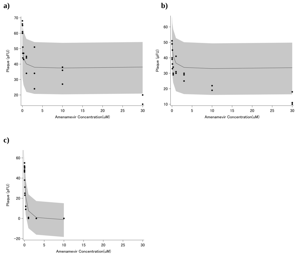
Figure 2-2- 4 Results of population PD modeling and visual predictive check for virus plaque data
