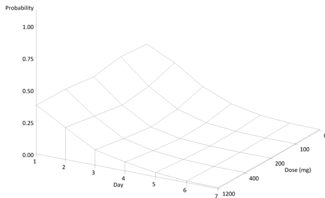
Figure 2-2- 6 Results of model predicted time course profiles in humans.
