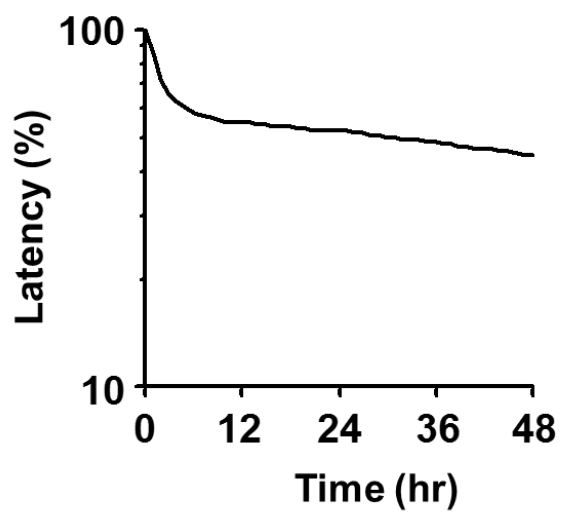
Figure 1- 5 Latency calculated based on the data shown in Figure 1- 3(C)
