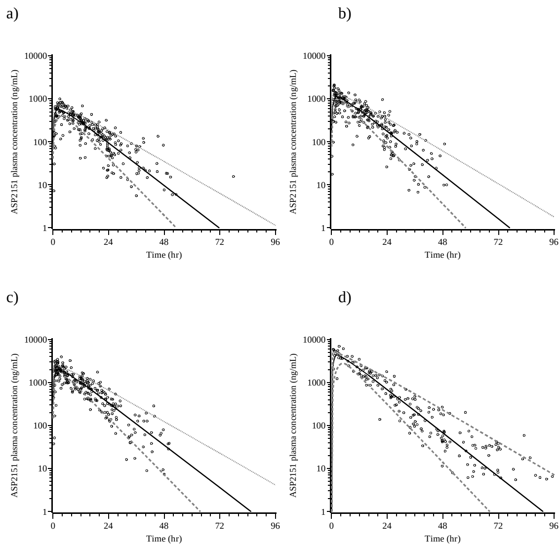
Figure 2-1- 1 Visual predictive check
