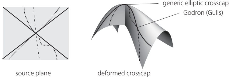
Figure 3: Non-generic elliptic crosscap is deformed to a generic one with producing a tangential point (gulls) of the parabolic curve and the flecnodal curve.
