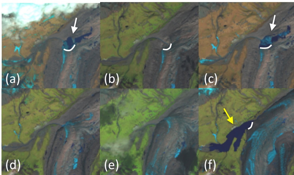
Figure 7-7: Spatial extent of supraglacial lake (white arrows in a and c) and formation of Hazard Lake (yellow arrow in f). The false-color composite images were derived from Landsat-8 taking on (a) 26 May 2014, (b) 23 August 2014, (c) 22 May 2015, (d) 14 June 2015, (e) 16 July 2015, (f) 16 June 2016. The white lines indicate the outlet tunnel from glacial inside. The Hazard lake is filled in (f).
