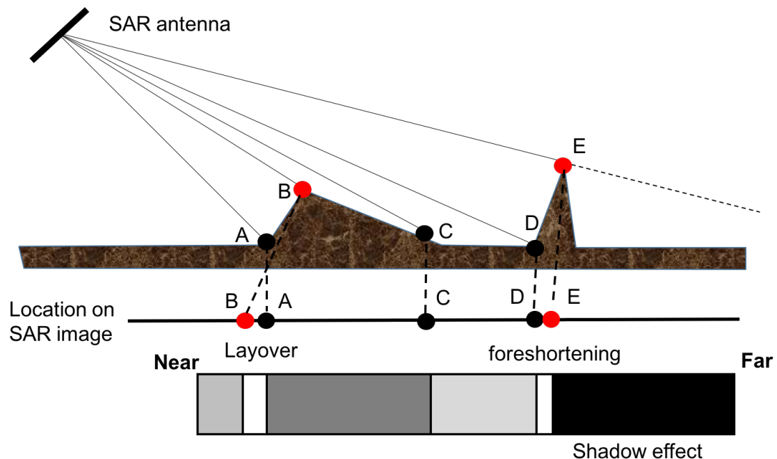
Figure 2-2: Schematic image of foreshortening, layover, and shadow effect. Modified from Ouchi (2009).
