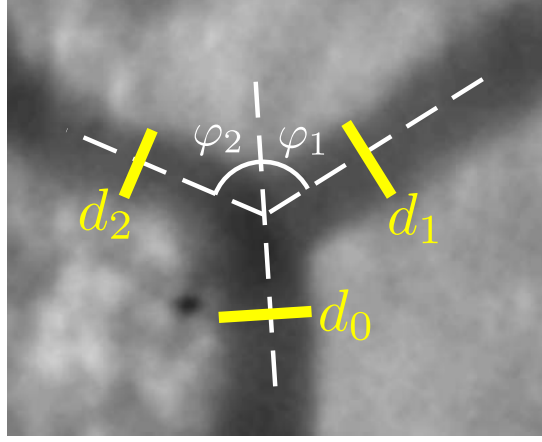
Fig. 3.2 Measurement of branching geometry.
