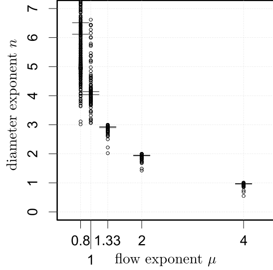
Fig. 5.7 Diameter exponents of triple junction in main veins of simulation plotted against flow exponents.
