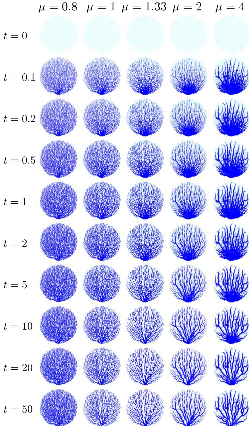
Fig. 5.1 Simulation results for varying flow exponent \mu in the circular shape. The main veins are drawn in proportion to the simulation result with the common limitation of maximum radius, whilst the very thin veins are drawn with dashed, dotted, or light blue line.
