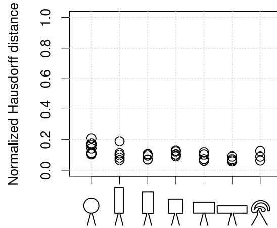
Fig. 4.8 Normalized Hausdorff distance for networks formed in each arena shape. The shapes tested are illustrated along the abscissa: from left to right, circle, tall rectangles, square, wide rectangles, and an irregular shape. The exit is located at the bottom of shapes, indicated by the trapezoid channel. ( n = 5 for the circular and the rectangular shapes, n = 3 for the irregular shape).
