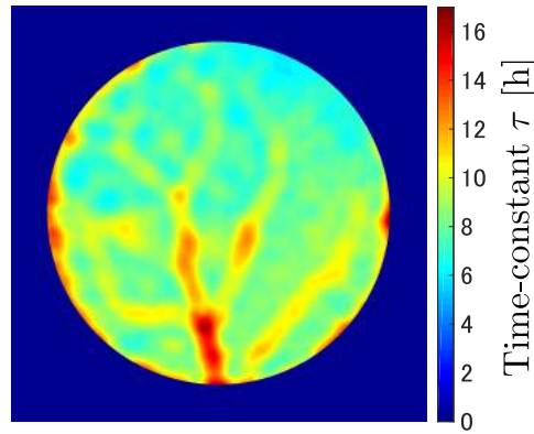
Fig. 4.4 Map of time-constant \tau by which time development of thickness h(t) in every point of arena is fitted to exponential formula h(t) = h_0e^{-t/\tau} where h_0 is another estimated parameter.
