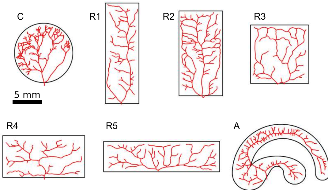
Fig. 4.7 Manually extracted evacuation network emerging in arenas.
