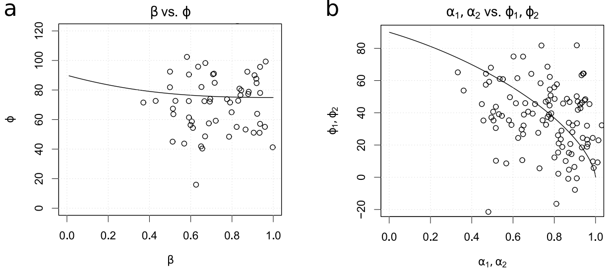
Fig. 4.12 Relationship between branching angle and thickness ratio. The solid lines of (a) indicate curves of Eq. (4.1), and that of (b) indicate Eq. (4.2) and Eq. (4.3).
