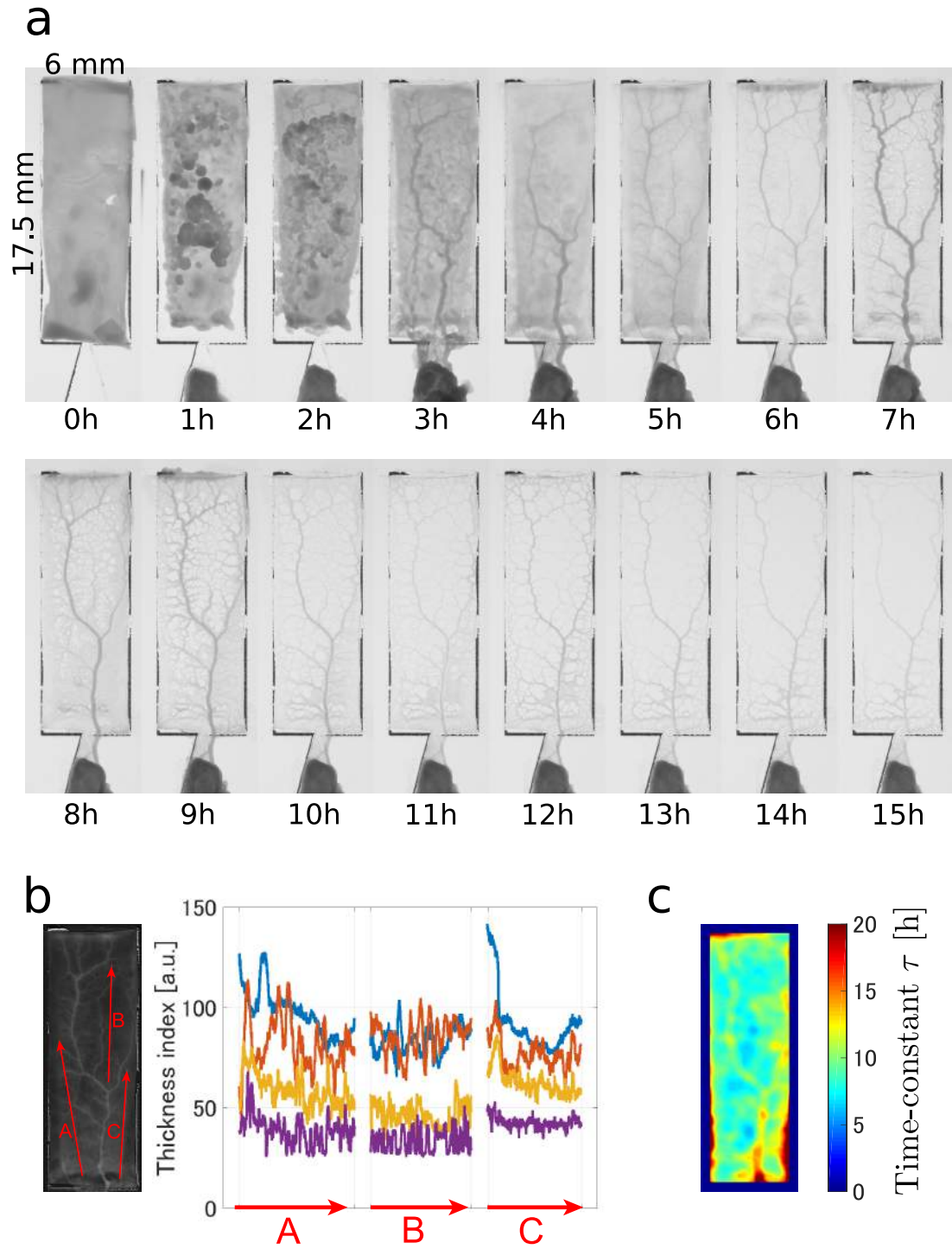
Fig. 4.5 Evacuation network emerging in a rectangular shape ( 6 \text{ mm} \times 17.5 \text{ mm} ). (a) Time-lapse images of evacuation. (b) Line-profile analysis. (c) Time-constant map.
