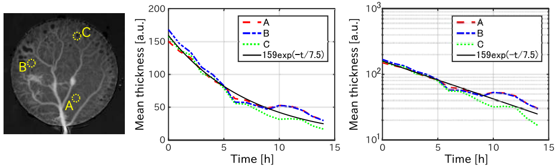
Fig. 4.3 Changes in the thickness of the plasmodium over time, monitored at three different inter-vein regions (left, A, B, and C). The plots show the time courses for the three points in addition to exponential fitting 159e^{-t/7.5} to the three lines with linear y-axis (middle) and logarithmic y-axis (right).
