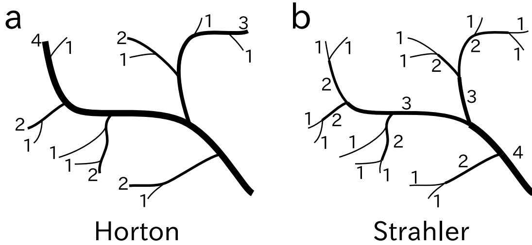
Fig. 2.1 Example of river ordering system of Horton (a) and Strahler (b).
