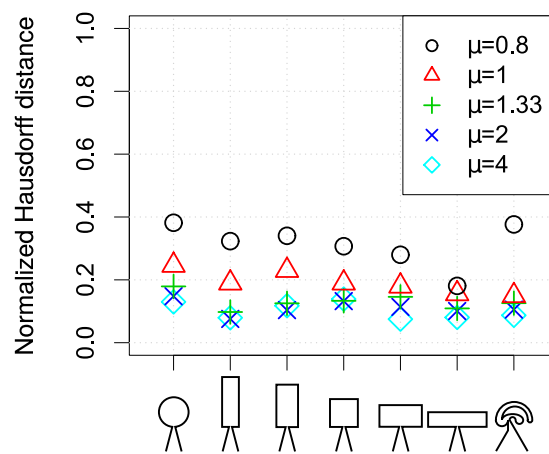
Fig. 5.6 Normalized Hausdorff distance between the simulated main network and all points in the arena.
