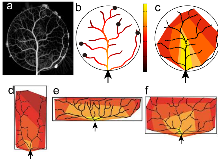
Fig. 4.9 Hydrodynamic conductivity of vein-network observed in the confined circular shape. (a) Thickness image of vein-network in the circle with diameter 1 cm. (b) Hydrodynamic conductivity along the main vein-network. A certain value of same HC was marked by the black dots on the network near the boundary of confined space. (c) Convex envelop for the dots marked in the figure b. (d, e, f) The same analysis on other shapes. Arrows indicate the location of exit.
