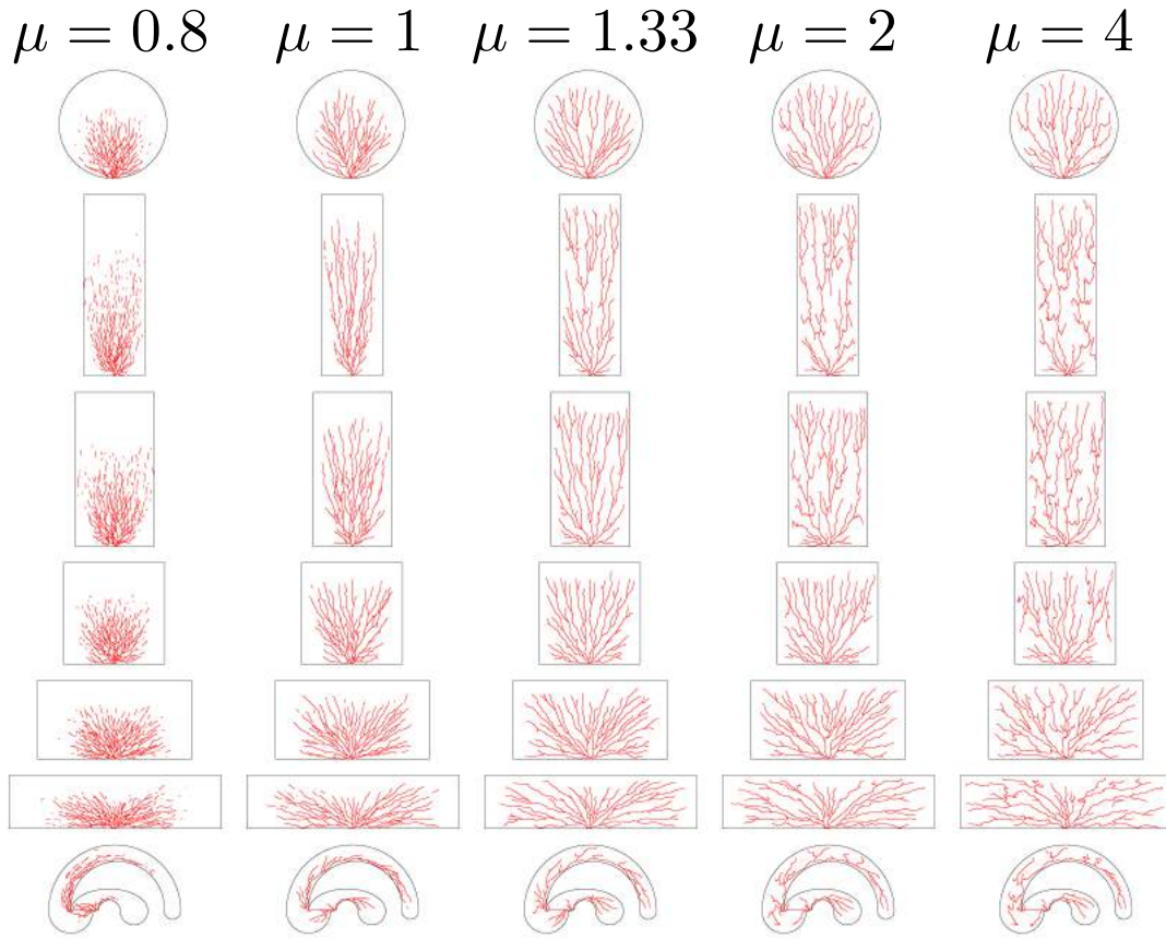
Fig. 5.5 Main networks from the simulation model, defined as the top 10% of the thickest veins.
