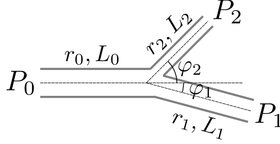
Fig. 2.3 A design of arteries transporting blood from fixed point P_0 to fixed points P_1 and P_2 .
