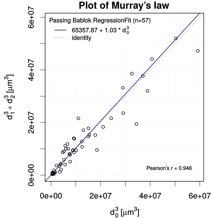
Fig. 4.10 Plot of d_1^3 + d_2^3 versus d_0^3 . The blue solid line is a regression fit by Passing-Bablok method, and the red dashed line indicates the identical line.
