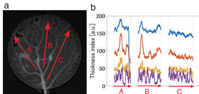
Fig. 4.2 Profile of plasmodial thickness along the monitored lines at times 0 (blue line), 4 (orange), 9 (yellow) and 14 (violet) hours after introducing the exit.
