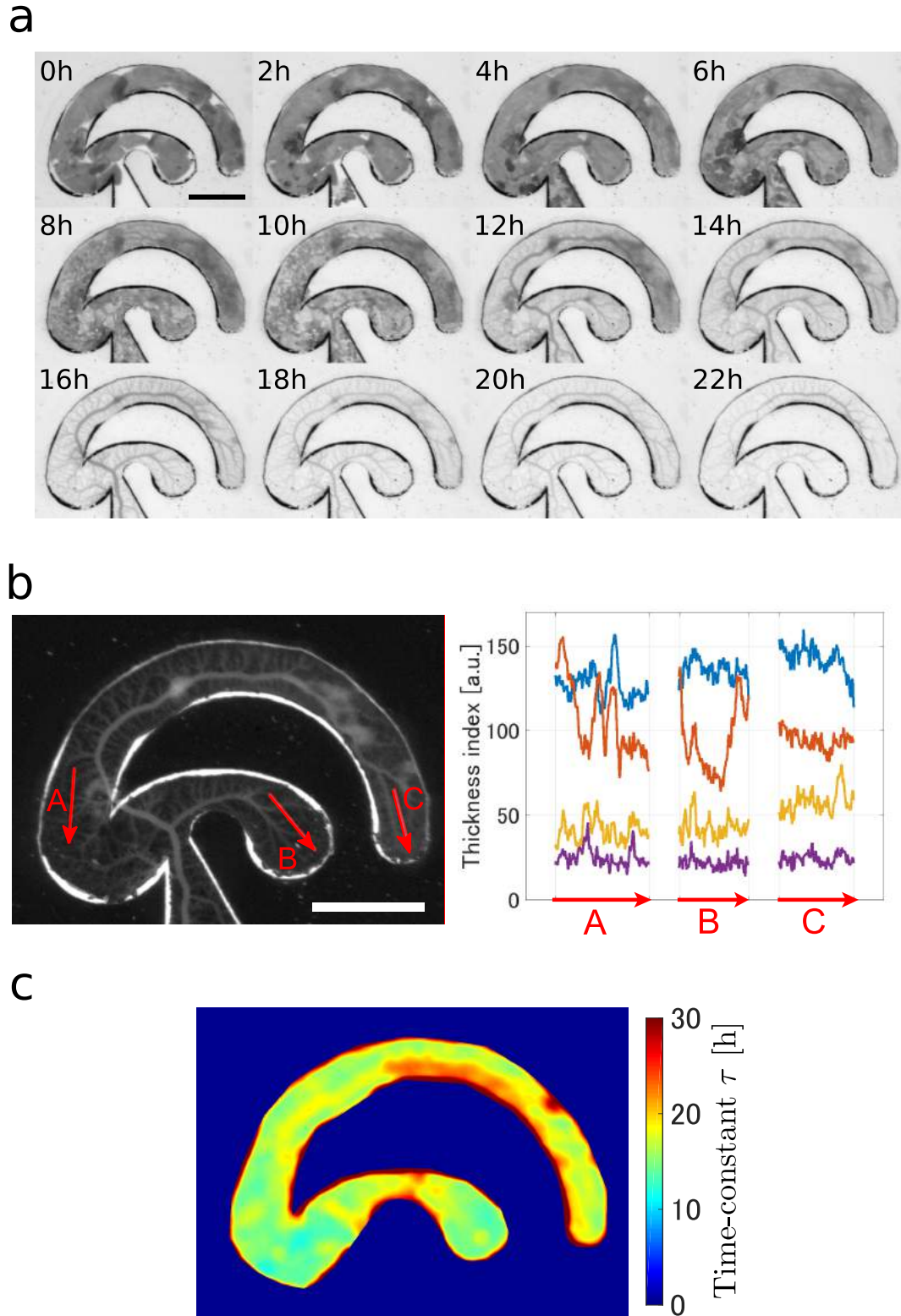
Fig. 4.6 Evacuation network emerging in an irregular shape (scale bar: 5 mm). (a) Time-lapse images of evacuation. (b) Line-profile analysis. (c) Time-constant map.
