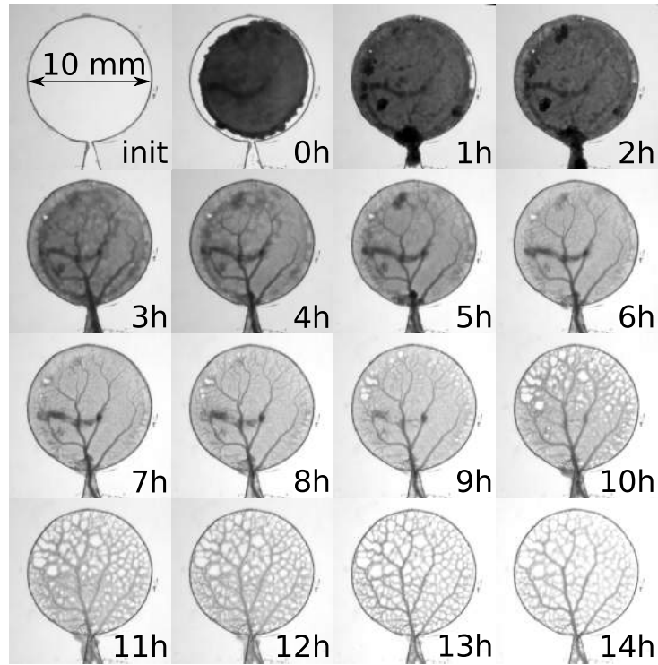
Fig. 4.1 Time course images following the development of a veination network by Physarum during evacuation from a confined circular arena.
