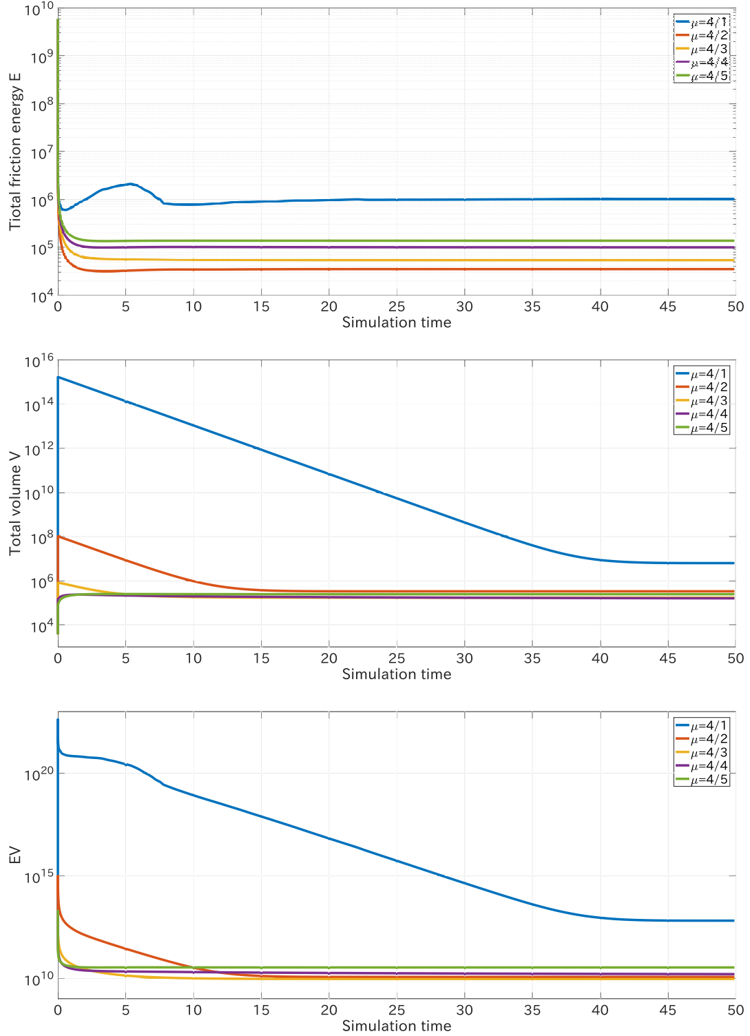
Fig. 5.8 Time courses for the change in frictional energy E (top), total volume V (middle), and their product EV (bottom) for the simulation results from the circular arena.
