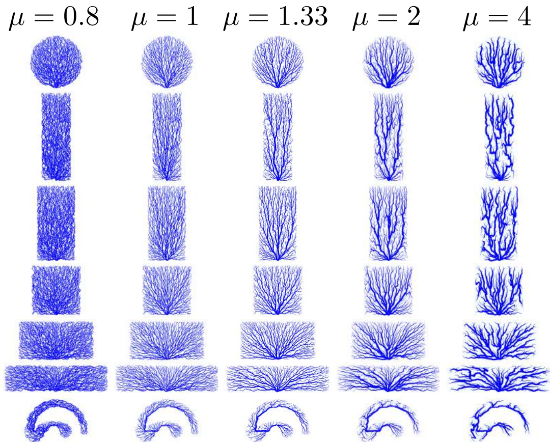
Fig. 5.4 The final states of simulations for varying flow exponent \mu in the different arena shapes (C, R1, R2, R3, R4, R5, and A, from top). The veins are drawn in the same way to Fig. 5.1
