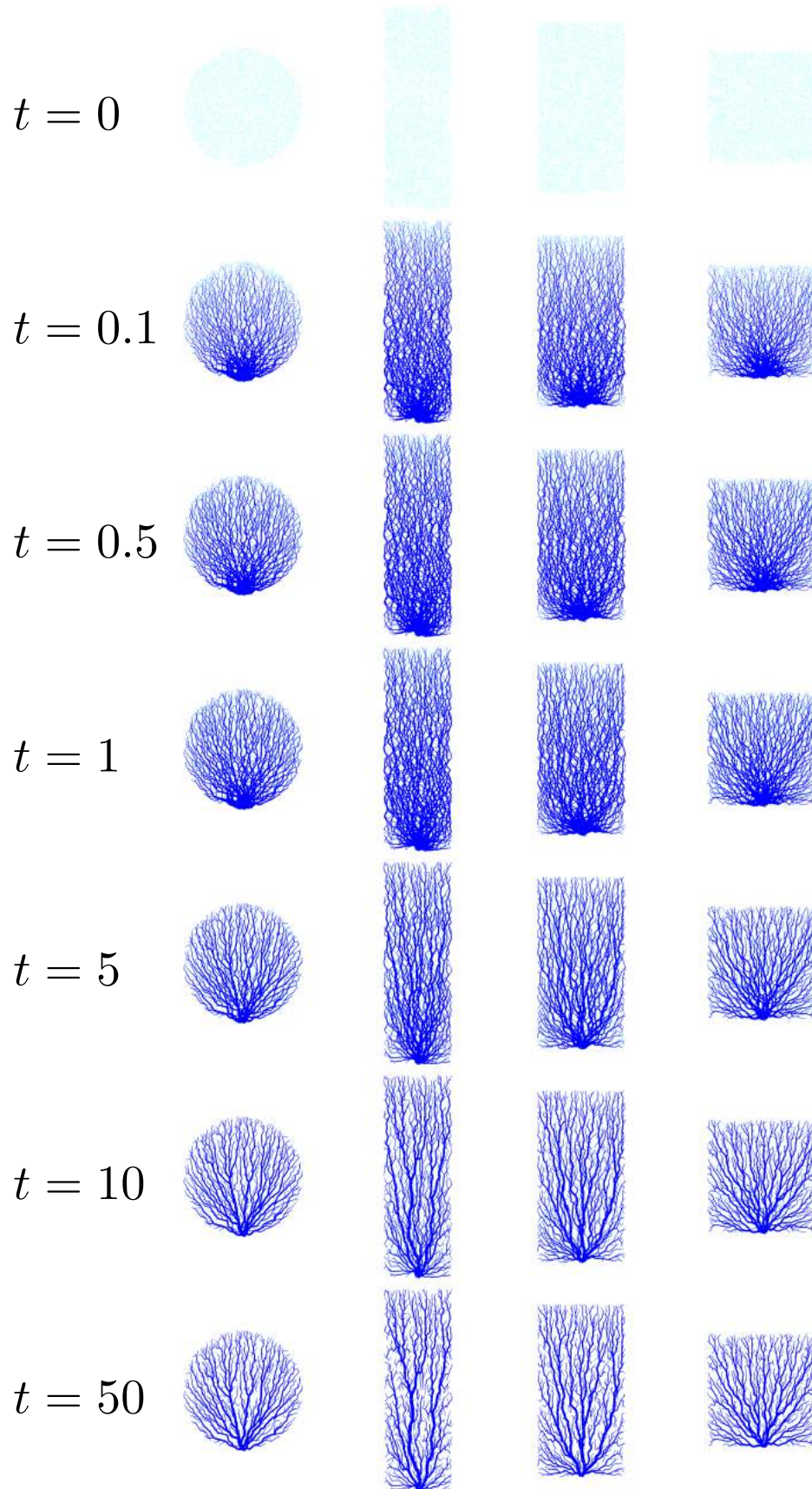
Fig. 5.2 Simulation results in the different arena shapes (C, R1, R2, and R3, from left) for flow exponent \mu = 1.33 . The veins are drawn in the same way to Fig. 5.1
