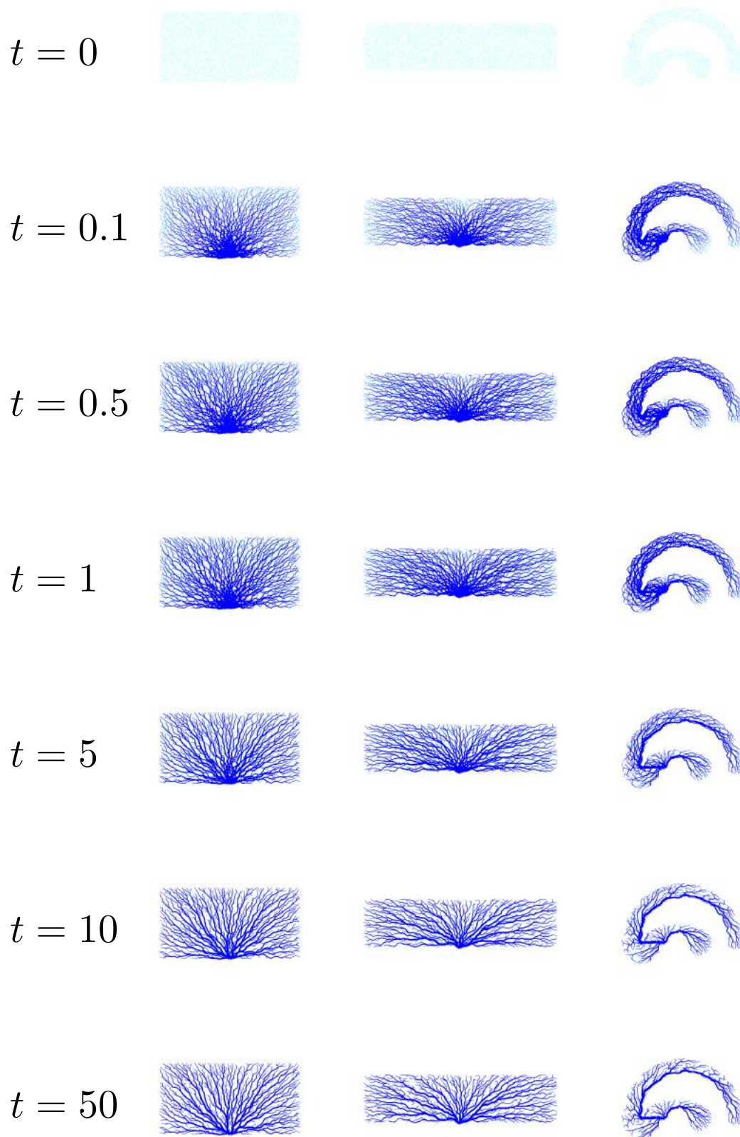
Fig. 5.3 Simulation results in the different arena shapes (R4, R5, and A, from left) for flow exponent \mu = 1.33 . The veins are drawn in the same way to Fig. 5.1
