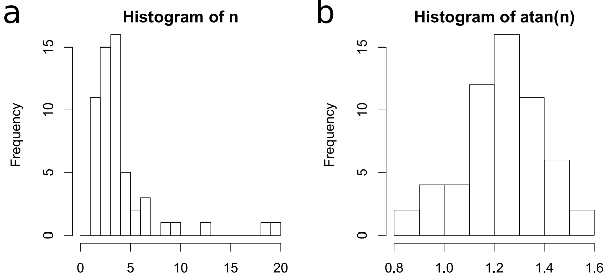
Fig. 4.11 (a) Histogram showing the distribution of the vessel scaling exponent n calculated from d_0^n = d_1^n + d_2^n for all bifurcations in the set of circular evacuation networks. (b) The arctan( n ) transformation normalised the data and gives a mean \pm S.D. of 1.235 \pm 0.045
