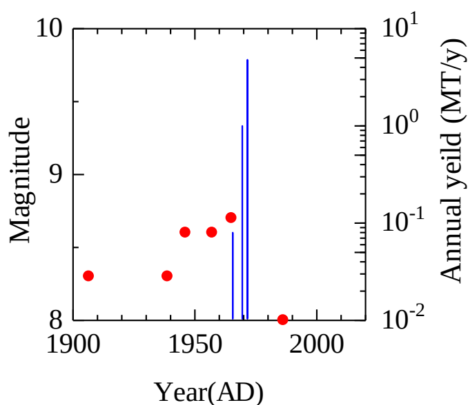
Fig. 5 Annual yield of underground nuclear explosions and magnitude of giant earthquakes in Alaska.
