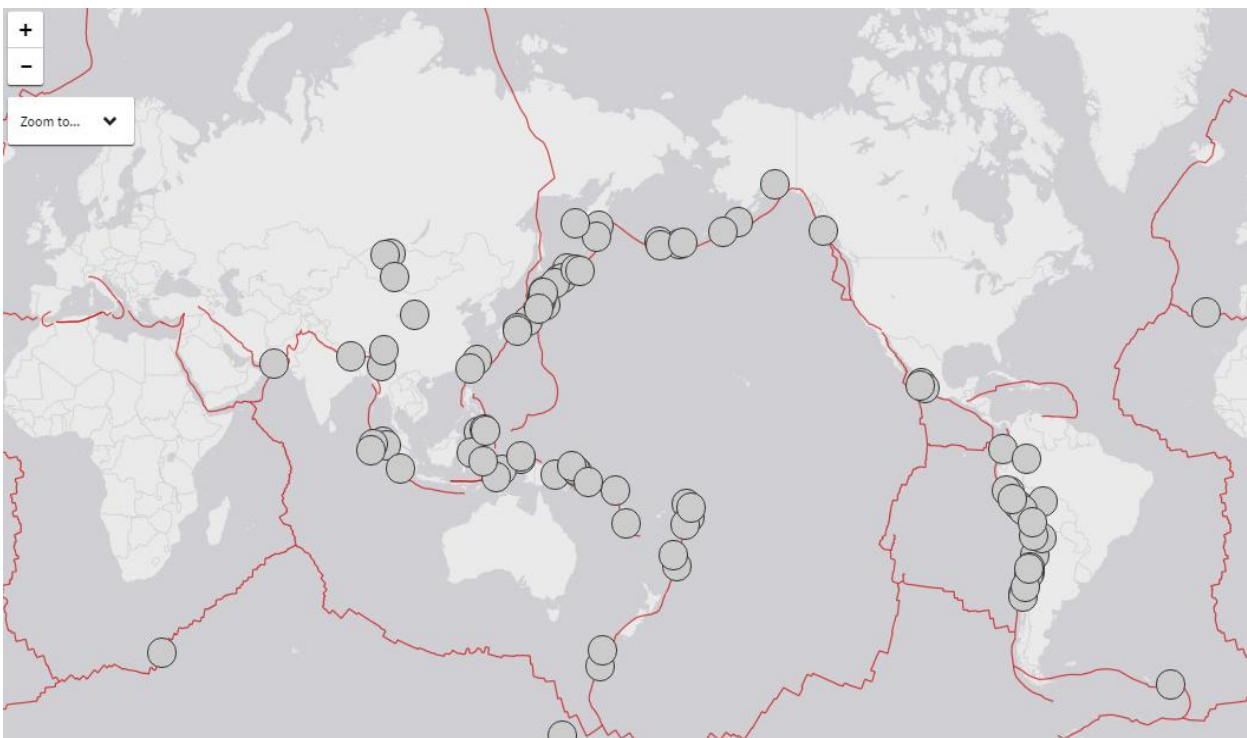
Fig. 4 Giant earthquakes between 1900 and 2016.
