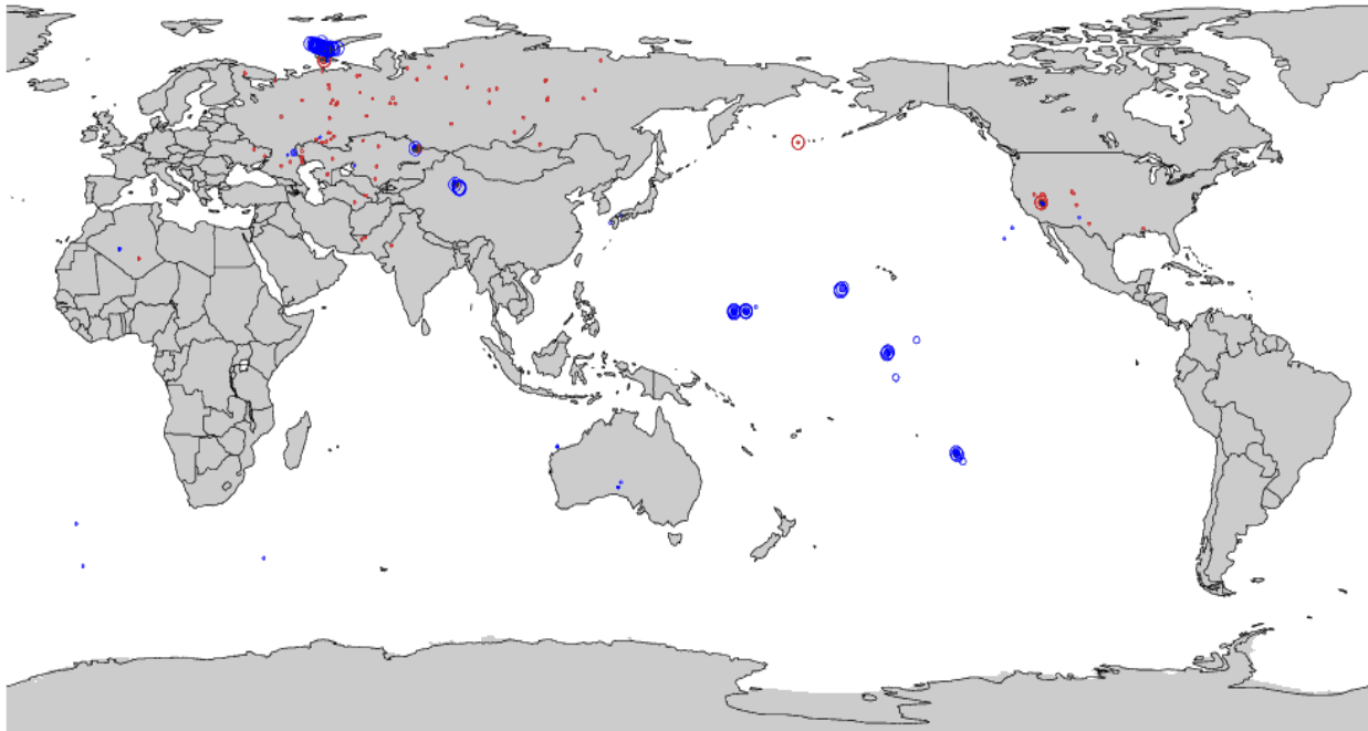
Fig. 3 Locations of underground nuclear explosions (red) and atmospheric nuclear explosions (blue).
