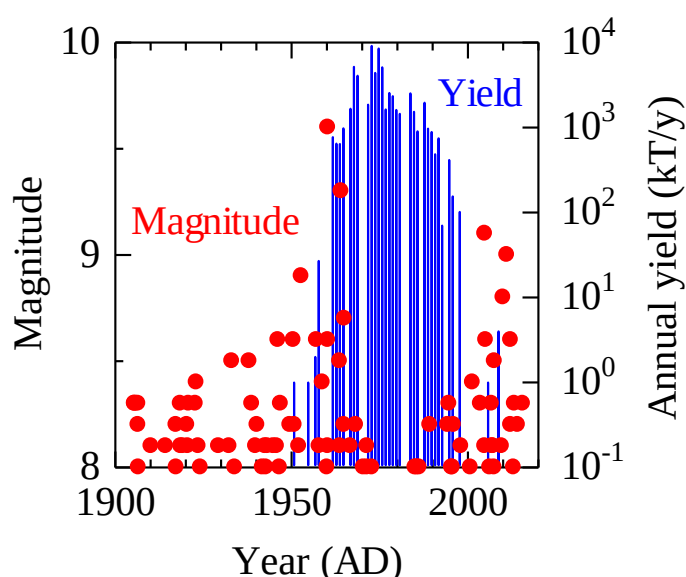
Fig. 1 Magnitude of giant earthquakes and annual yield of underground nuclear tests from 1900 to 2016.
