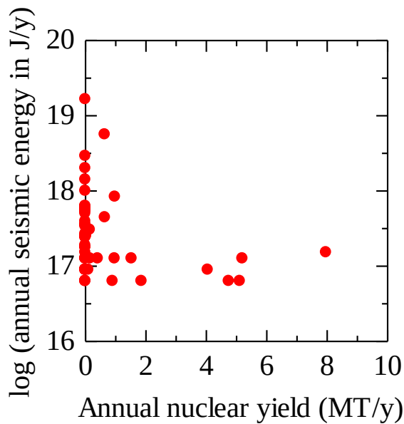
Fig. 2 Relationship between annual nuclear yield and annual seismic energy from 1900 to 2016.
