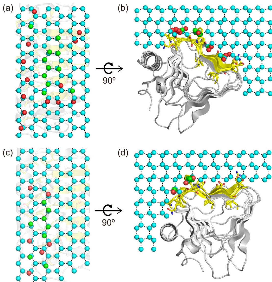
Figure 2.11 Superposing of the ice-like waters on TisAFP8 to the basal plane of the ice lattice.
