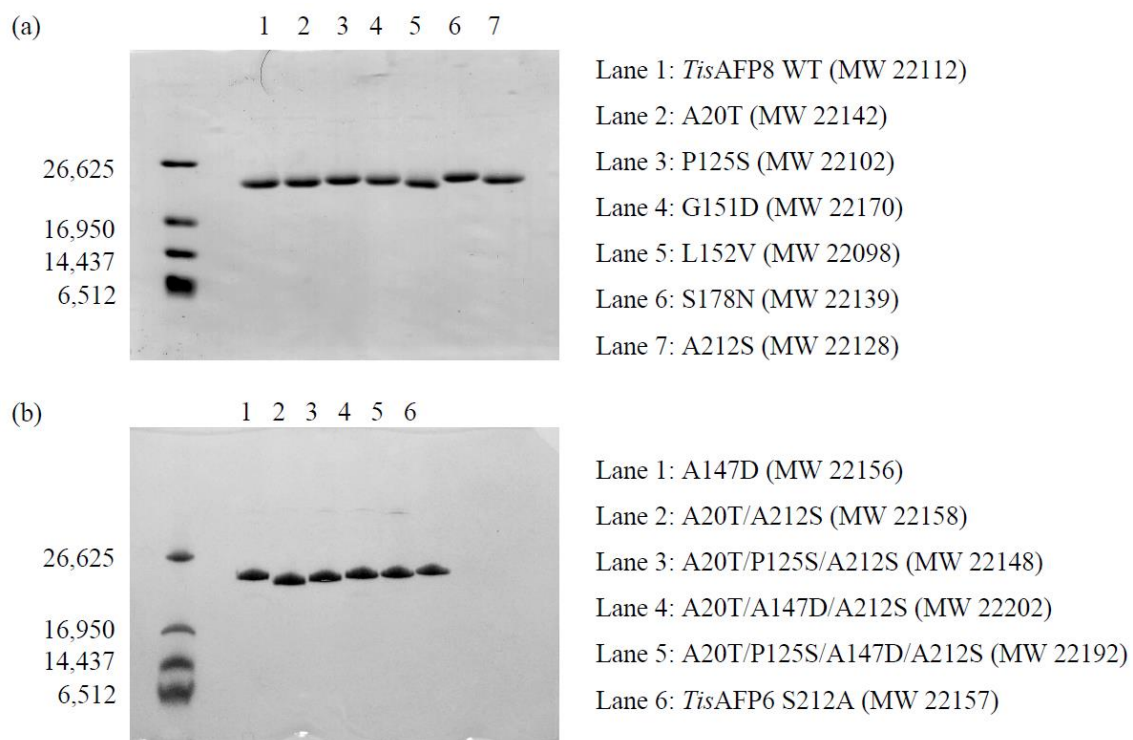
Figure 2.3 SDS-PAGE analysis of purified wild-type TisAFP s and their mutants.
