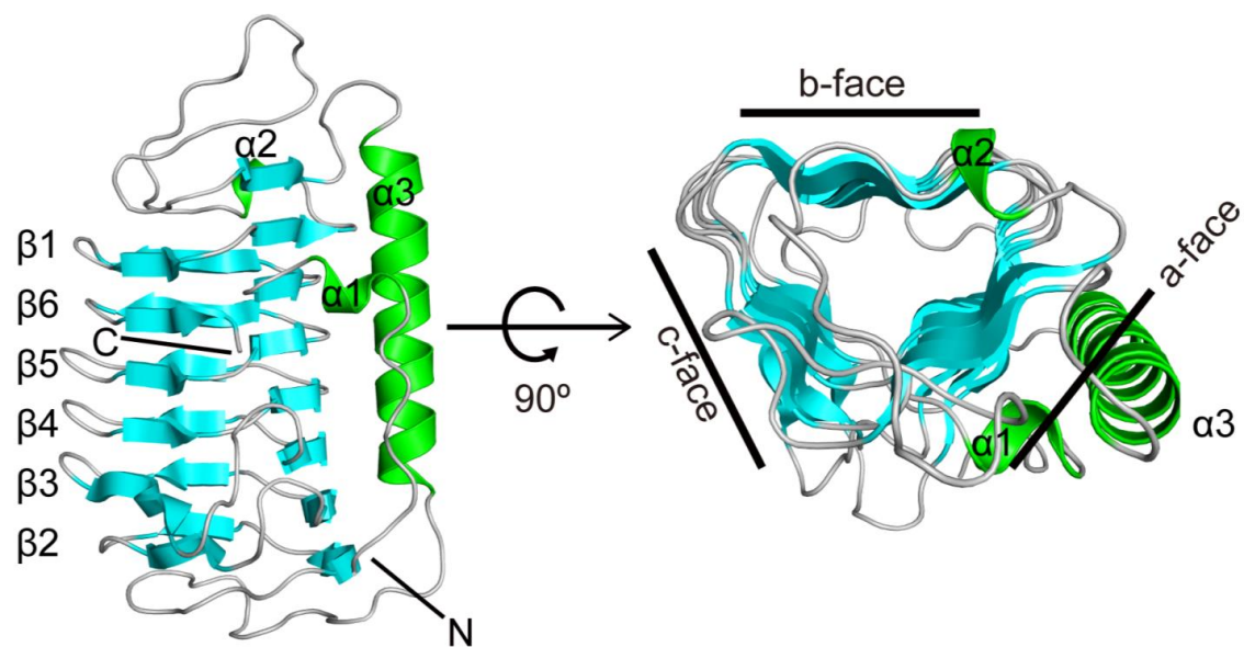
Figure 2.5 Crystal structure of TisAFP8 .
