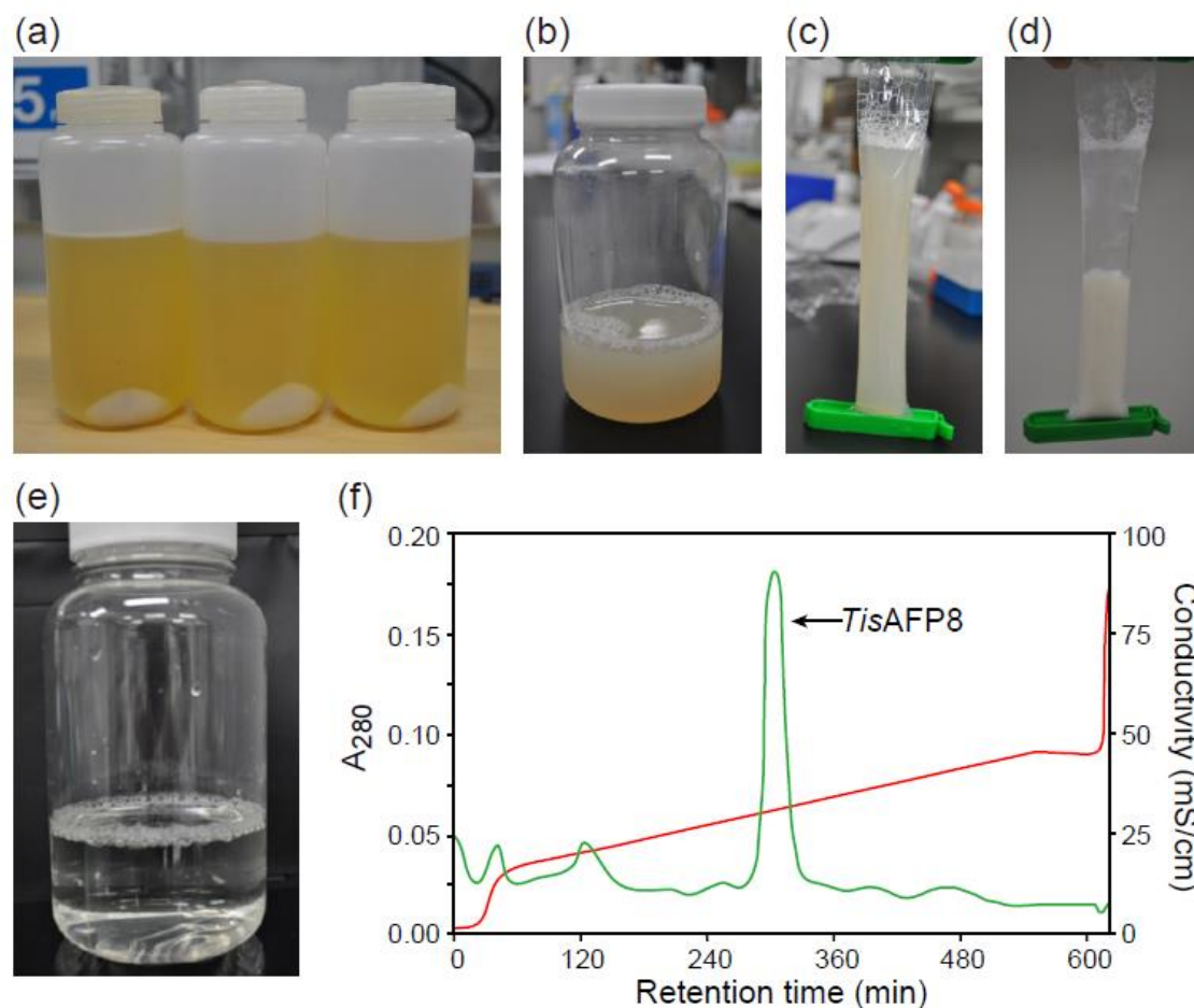
Figure 2.1 Purification of recombinant TisAFP8 wild type.
