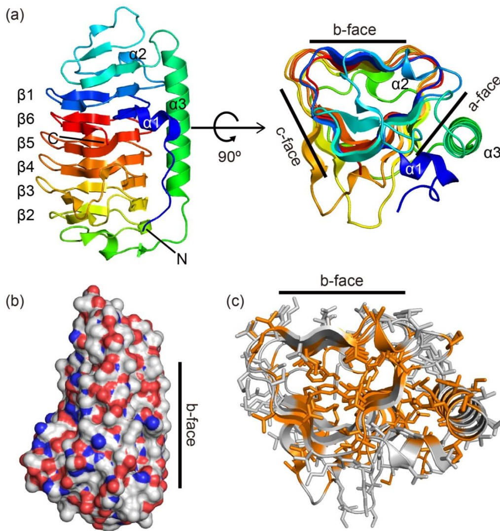
Figure 1.10 X-ray crystal structure of TisAFP6 .
