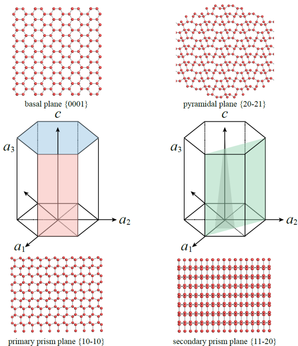
Figure 1.7 Hexagonal unit cell of ice lattice ( I_h ) and representative ice planes involving in AFP interactions.
