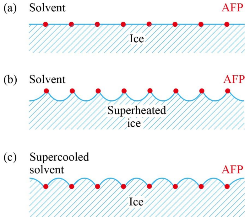
Figure 1.1 Simple model of adsorption-inhibition mechanism.
