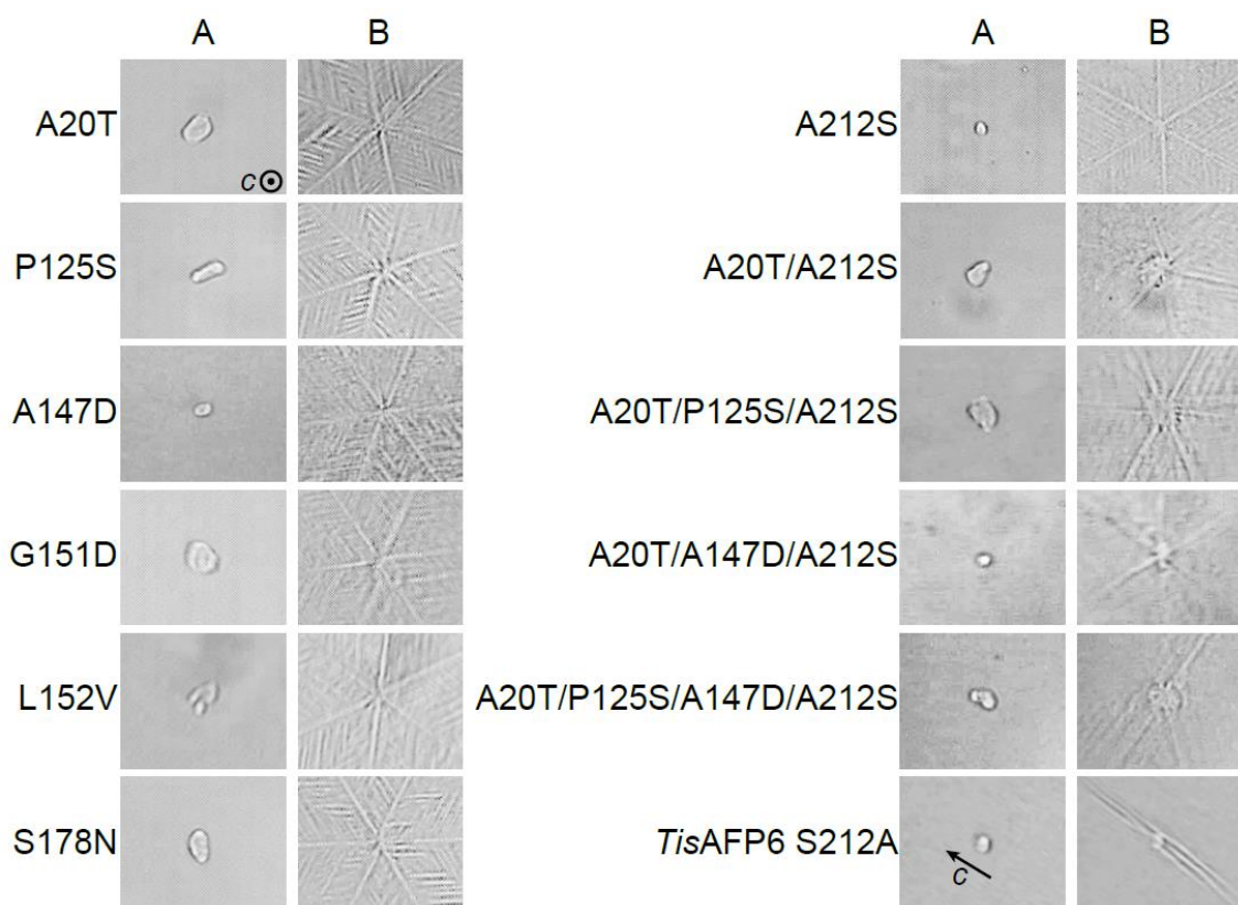
Figure 2.10 Ice crystal bursts in the presence of each mutant.
