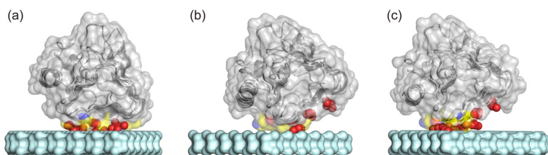
Figure 2.12 Docking of TisAFP8 and TisAFP6 to the basal plane of ice.
