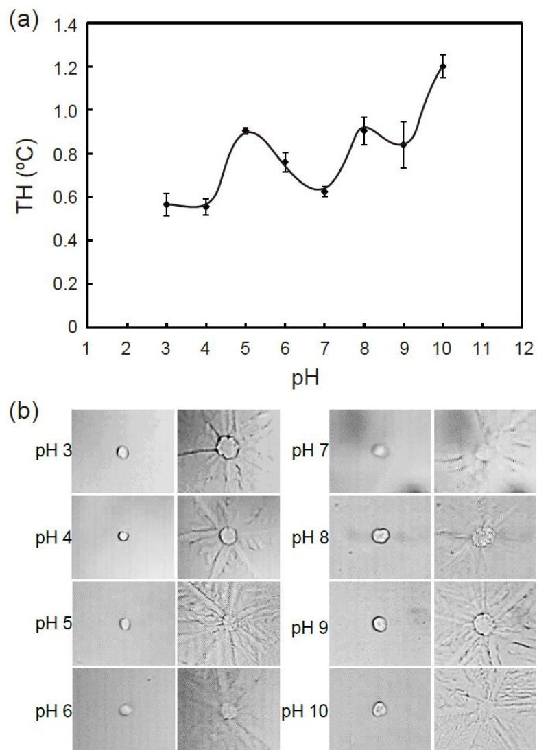
Figure S2.13 Effect of pH on TH activity and ice crystal morphology of TisAFP8 .
