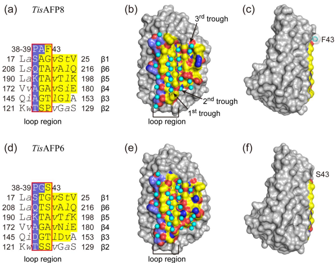
Figure 2.6 Comparison of the IBS of TisAFP8 and TisAFP6 .
