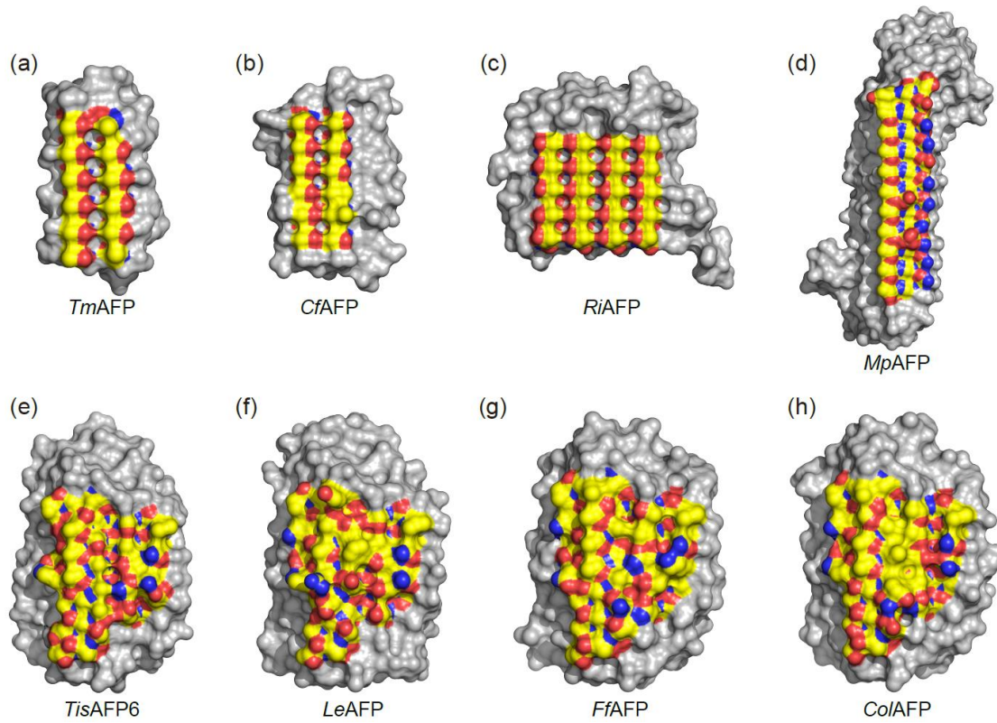
Figure 1.11 Regular and repetitive IBSs of hyperactive AFPs Vs complex IBSs of homologous AFPs to TisAFP6 .
