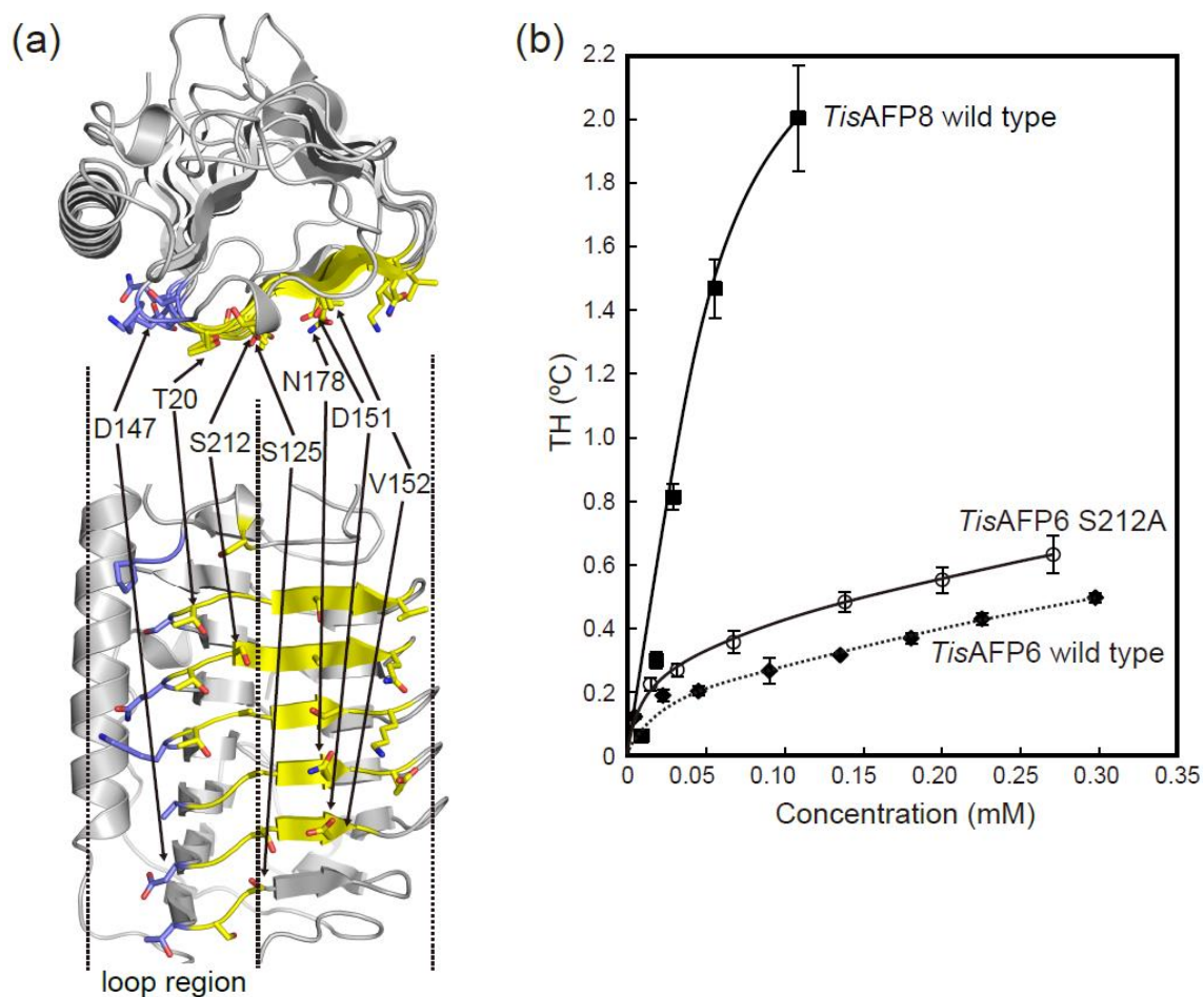
Figure 2.8 Site-directed mutants introduced to the IBS of TisAFP6 .
