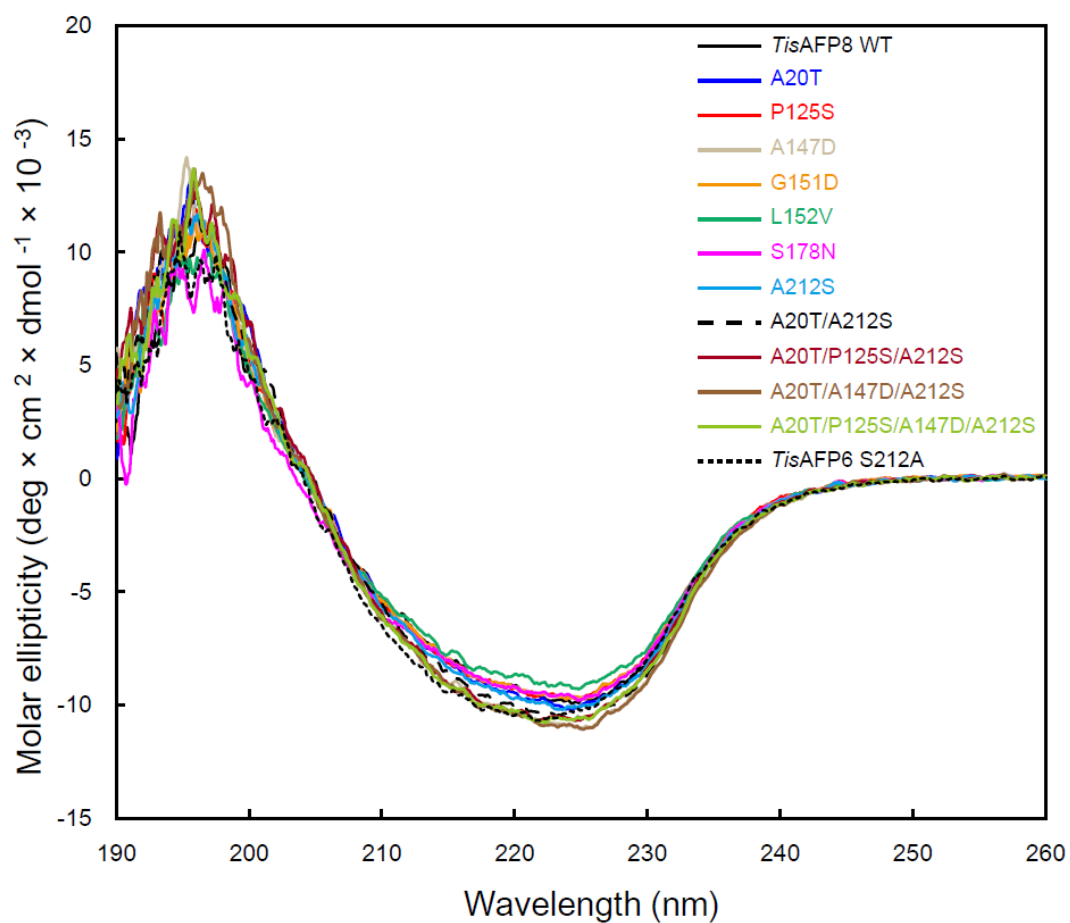
Figure 2.9 CD spectra of wild-type (WT) TisAFP8 and mutants.
