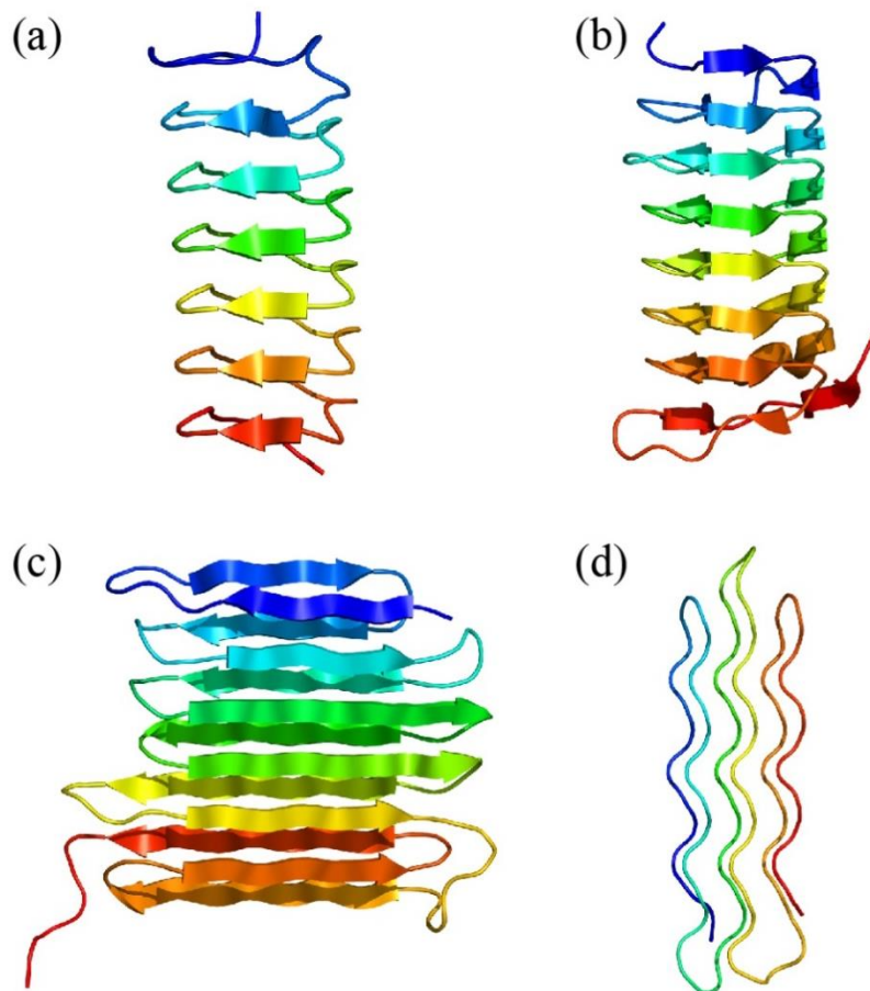
Figure 1.4 X-ray crystal structures of insect AFPs.
