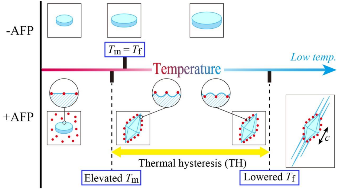
Figure 1.2 Schematic representation of thermal hysteresis.
