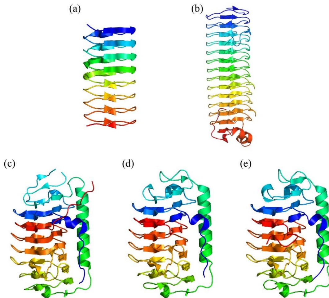
Figure 1.5 X-ray crystal structures of other AFPs.
