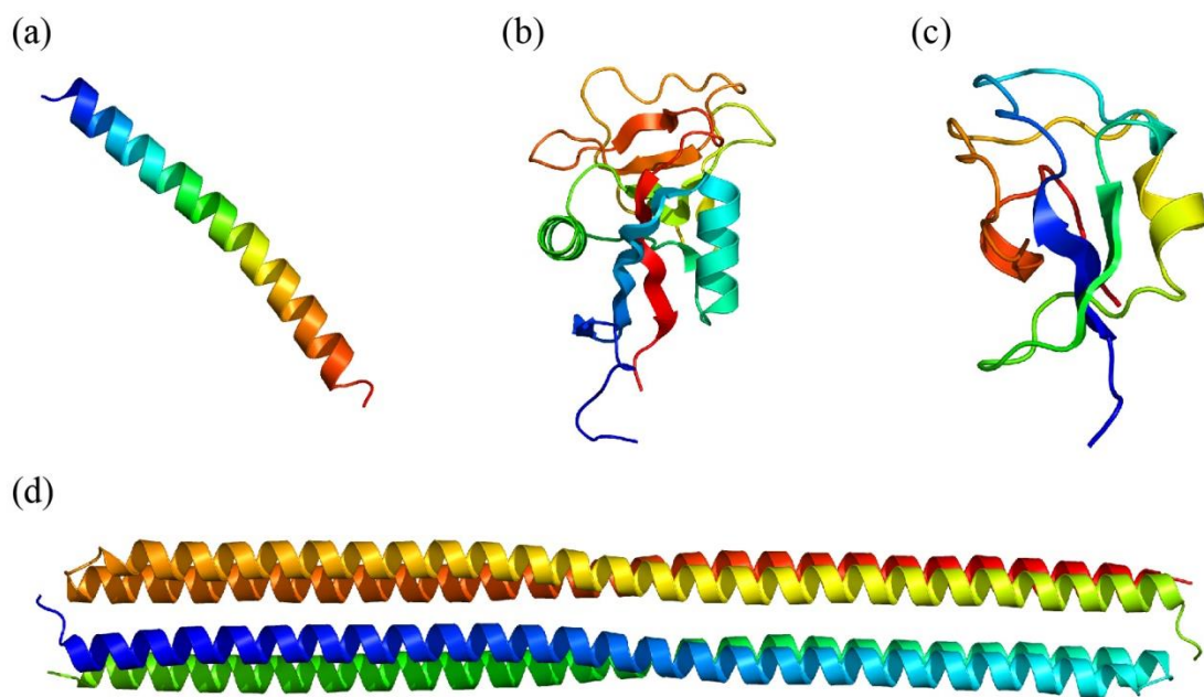
Figure 1.3 X-ray crystal structures of fish AFPs.
