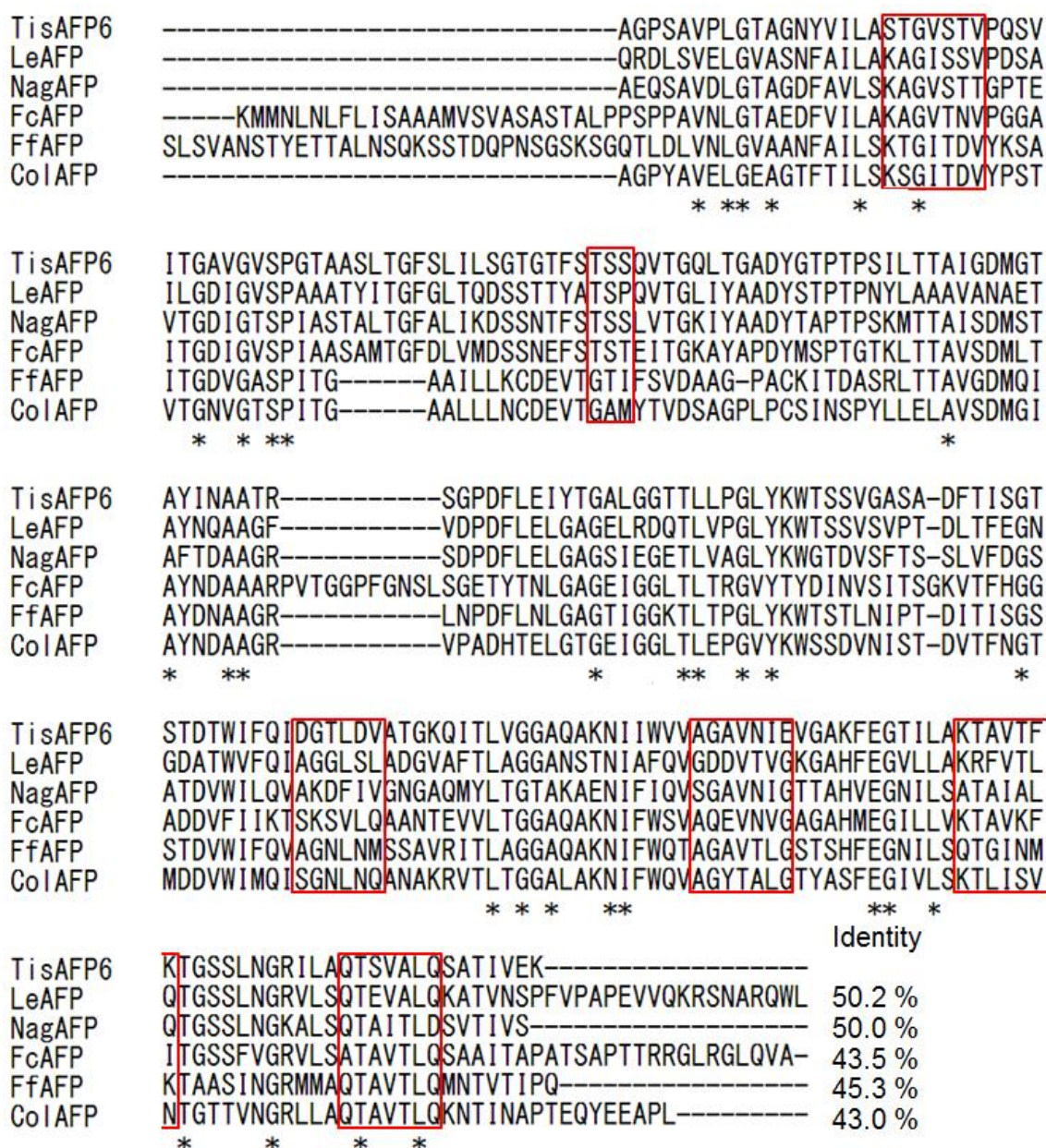
Figure 1.6 Amino acid sequence alignment of homologous AFPs to TisAFP6.
