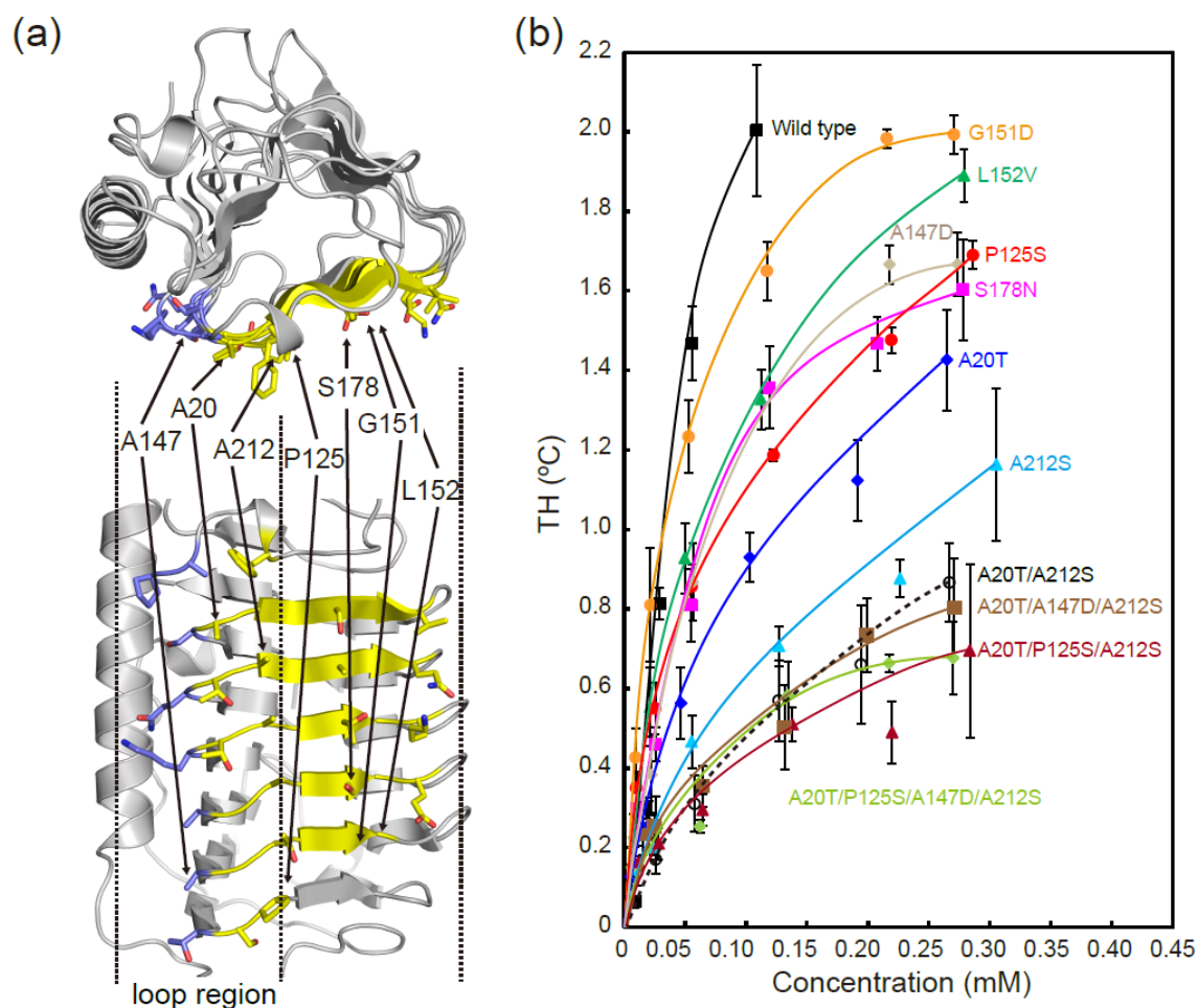
Figure 2.7 Site-directed mutants introduced to the IBS of TisAFP8 .
