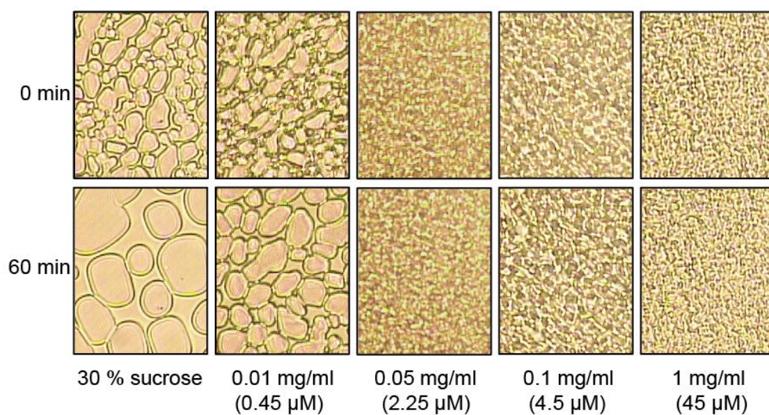
Figure S2.14 Inhibition of ice recrystallization by TisAFP8 .
