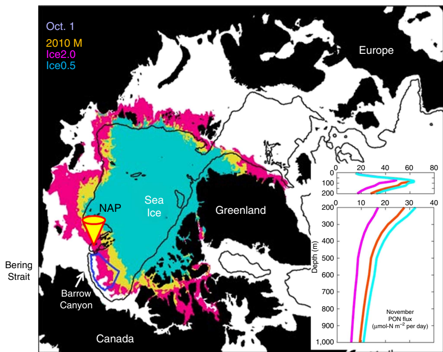
Figure 6 | Impact of sea ice reduction. Sea ice distribution on 1 October in the (orange) 2010 M, (pink) Ice2.0, and (sky blue) Ice0.5 cases. Black contours represent 1,000 m isobaths. The location of Station NAP is shown by a yellow cone. The inset shows the vertical profile of November mean PON flux in each case (μmol-N m -2 per day). The average region is the southwestern Canada Basin, which is outlined by a blue contour.
