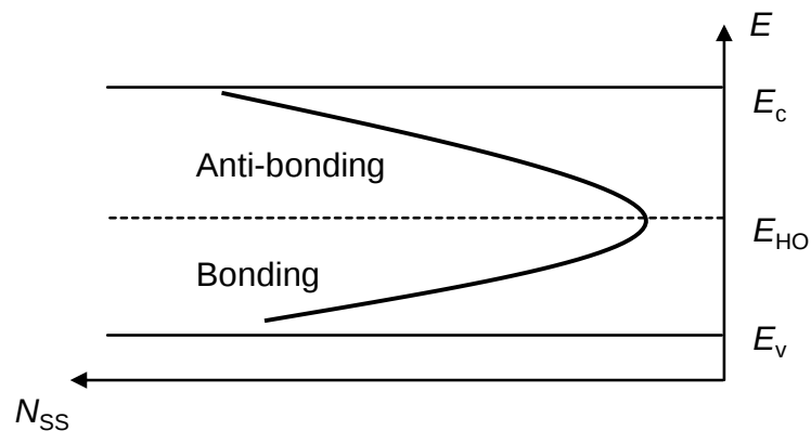
Fig. 2-3 Schematic image of interface state density distribution based on the DIGS model.
