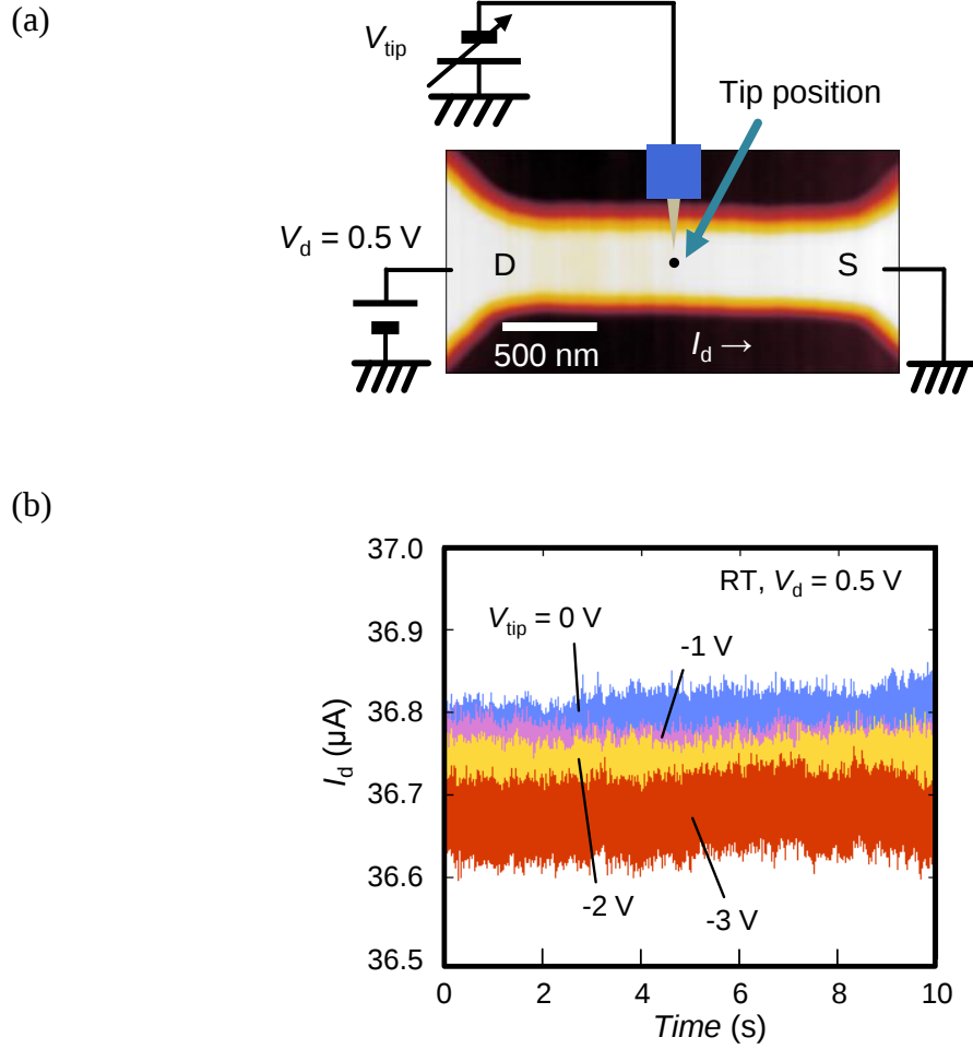
Fig. 6-8 (a) AFM image of the fabricated device with tip position and measurement circuit and (b) the tip bias dependence of drain current.
