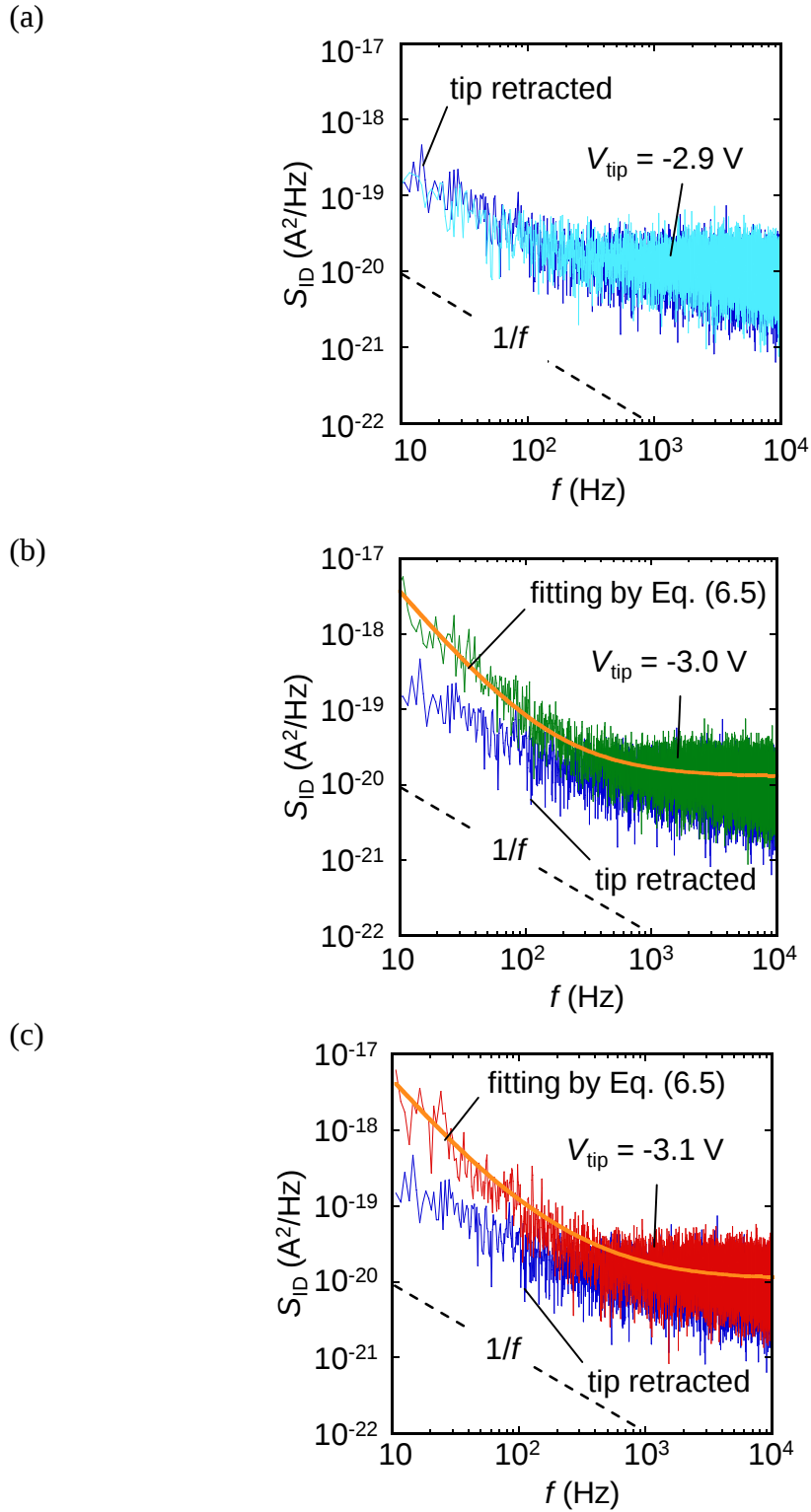
Fig. 6-10 Measured noise spectra with tip contact when (a) V_{tip} = -2.9 V, (b) -3.0 V, and (c) -3.1 V. Noise spectrum at which tip was retracted is also shown.
