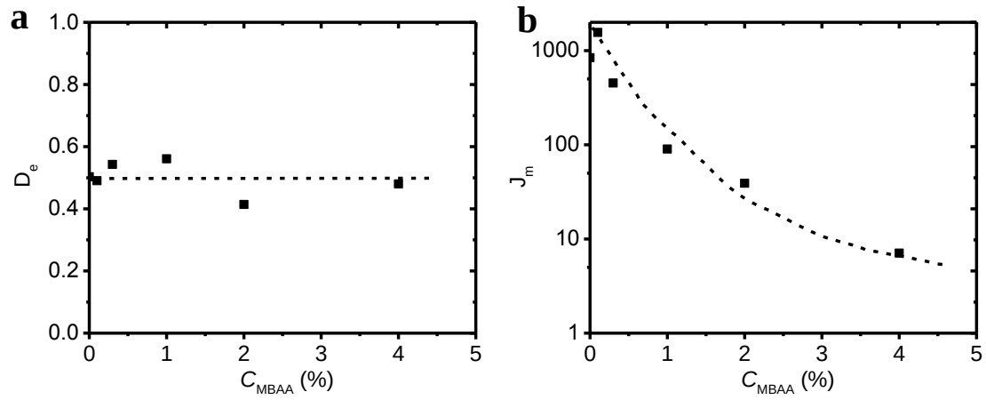
Figure S2. Chemical cross-linker density C_{\text{MBAA}} dependences of Deborah number (a) and theoretical first strain invariant value J_m (b) of PA- C_{\text{MBAA}} samples. The result was estimated from the tensile stress-strain curves performed at a stretching strain rate 0.011\text{s}^{-1} .
