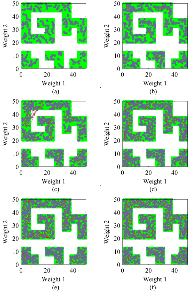
Fig. 4. Snapshots in incremental learning by REISOD. Let n is the number of data which have been learned. (a) n=250 . (b) n=500 . (c) n=750 . (d) n=1000 . (e) n=1250 . (f) n=1386 (final).
