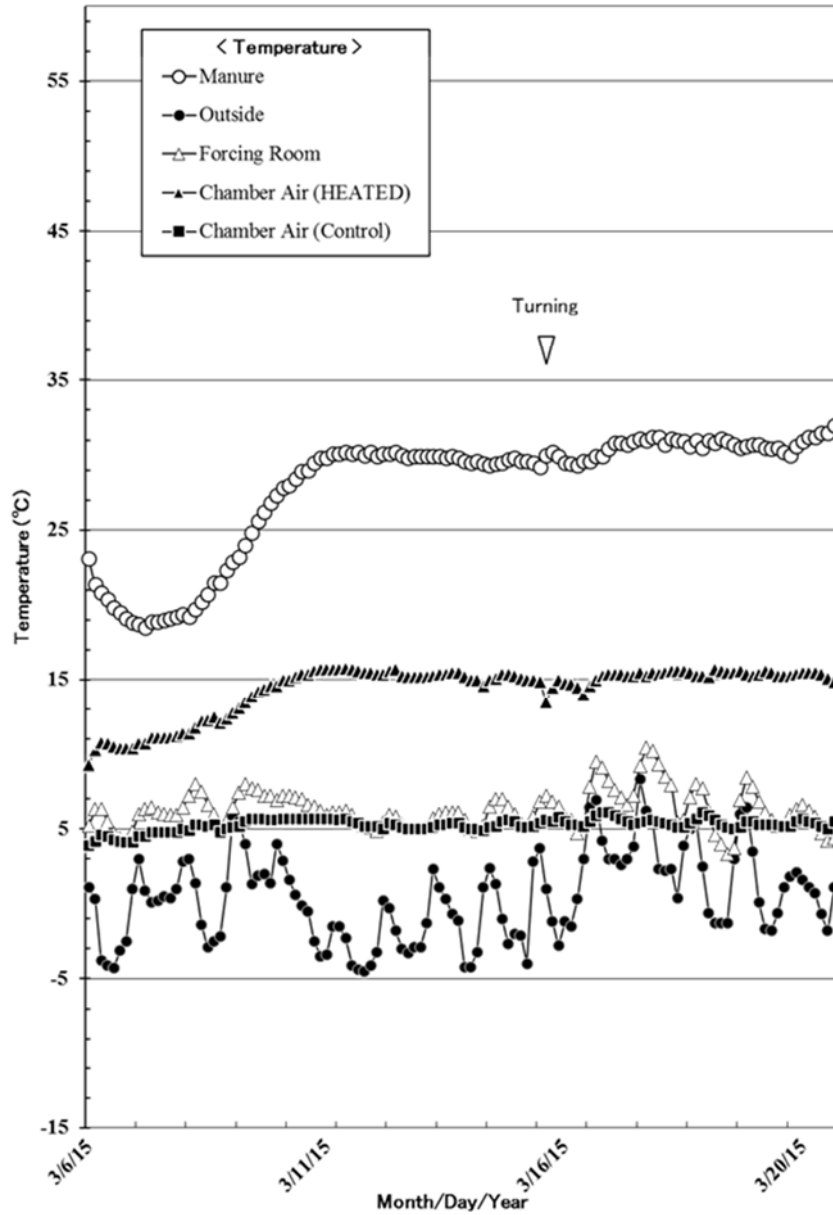
Fig. 2-6 Transition of air temperature during forcing culture (6 to 21 March, 2015). HEATED; temperature in the “HEATED” forcing chanber and Control; the temperature in the “CONTROL” forcing chamber.
