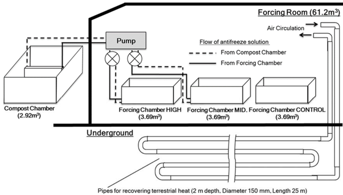
Fig. 2-1 Experimental facility used in semi-cold season, in 2013. The capacity of compost chamber was 2.92m 3 (1.8 × 1.8 × 0.9 (m)). The capacity of forcing chambers were 3.69m 3 (6.3 × 0.9 × 0.65 (m)), and those forcing chambers were installed in the forcing room (61.2m 3 ; 12.6 × 1.8 × 2.7 (m)). The forcing room was connected with a terrestrial heat recovery system, and the air was circulated between the forcing room and underground pipes for recovering terrestrial heat by electric fan through the system. The inside temperature of the forcing chambers was controlled manually at 3 temperatures, 19° C (HIGH), 17° C (MID.) and non-heating (CONTROL).
