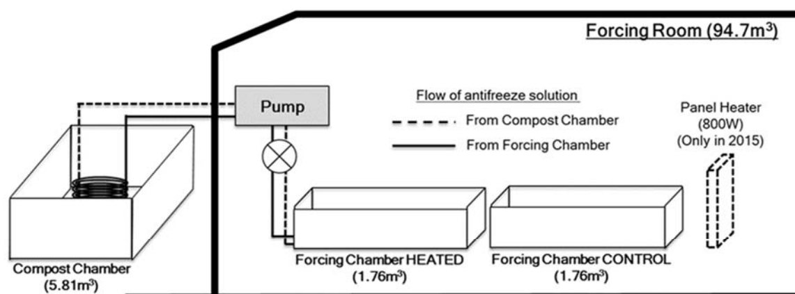
Fig. 2-2 Experimental facility in cold seasons, in 2014 and 2015. The capacity of compost chamber was 5.81m 3 (2.2 × 2.2 × 1.2 (m)). The capacity of forcing chambers was 1.76m 3 (3.0 × 0.9 × 0.65 (m)), and those forcing chambers were installed into the forcing room (94.7m 3 ; 12.6 × 1.8 × 2.7 (m)). A electric panel heater (800W) was used to maintain the air temperature of forcing room higher than 0°C, only in 2015. One chamber was used for the treated treatment (HEATED) and another for the non-treated control (CONTROL).
