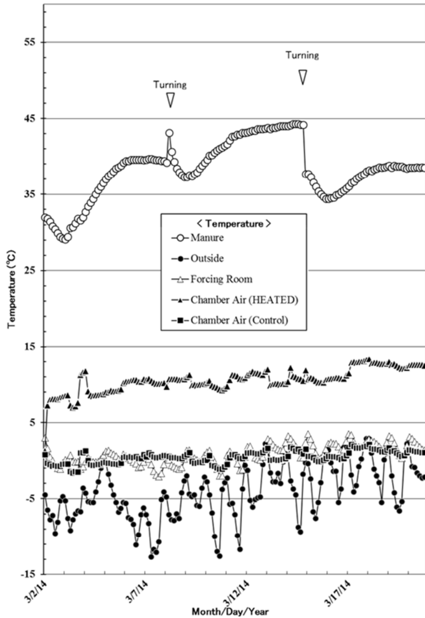
Fig. 2-5 Transition of air temperature during forcing culture (2 to 21 March, 2014). ). HEATED; temperature in the “HEATED” forcing chanber and Control; the temperature in the “CONTROL” forcing chamber.
