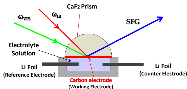
SFG setup with internal reflection geometry.
