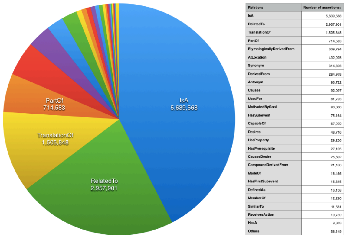
Figure 2.4: Relations of ConceptNet 5.3.
