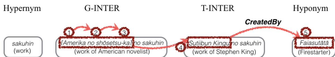
Figure 3.8: Procedure of CreatedBy relation extraction module.
