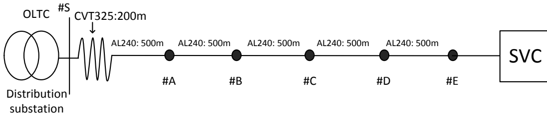
Fig. 4.17 Distribution system model primary nodes with SVC
