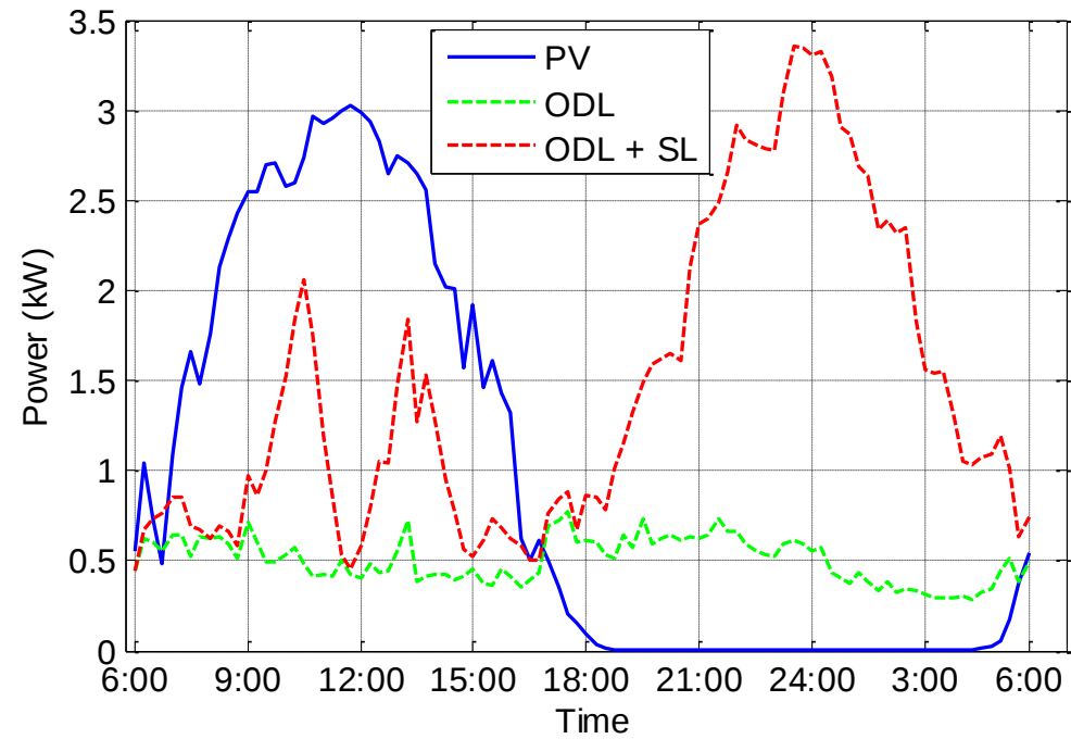
Fig. 3.8 Average PV and load power with running SLs at random time
