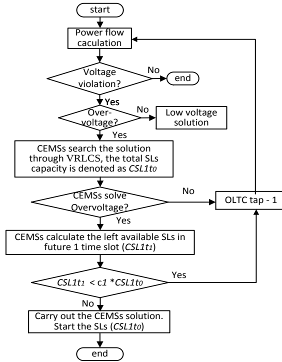
Fig. 4.10 Improved OLTC operation strategy of overvoltage
