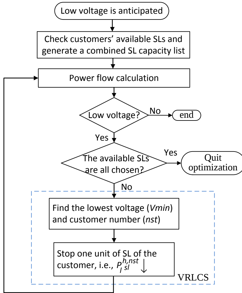
Fig. 4.13 flowchart of the VRLCS search process for low voltage prevention
