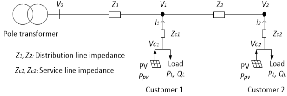
Fig. 1.9 Simple distribution system model with two customers
