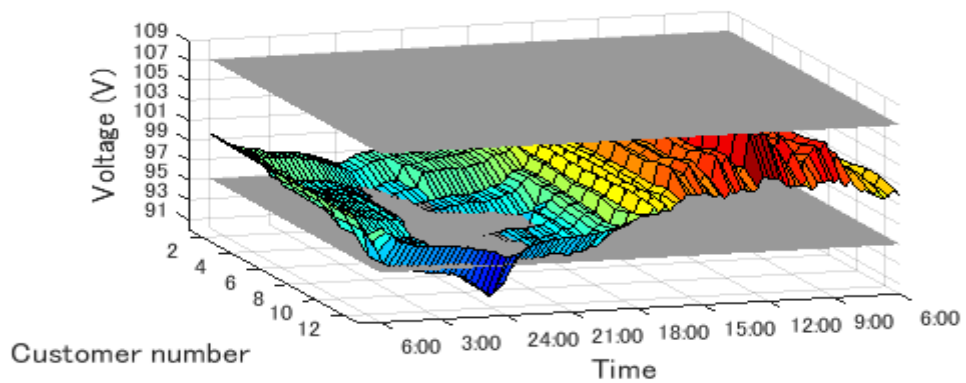
Fig. 3.23 1800-customer voltage condition of case 3 on 2 nd June
