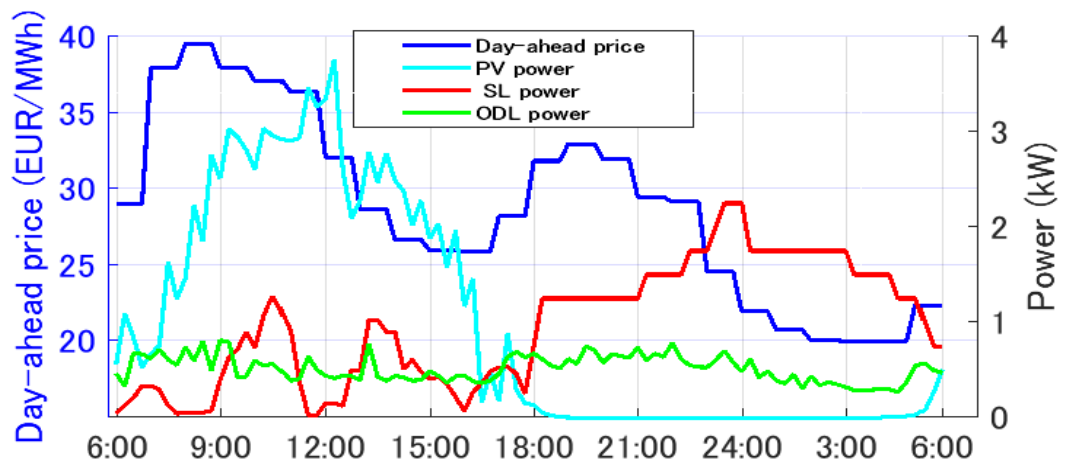
Fig. 3.18 Day-ahead price and PV, SL, ODL average power of case 3
