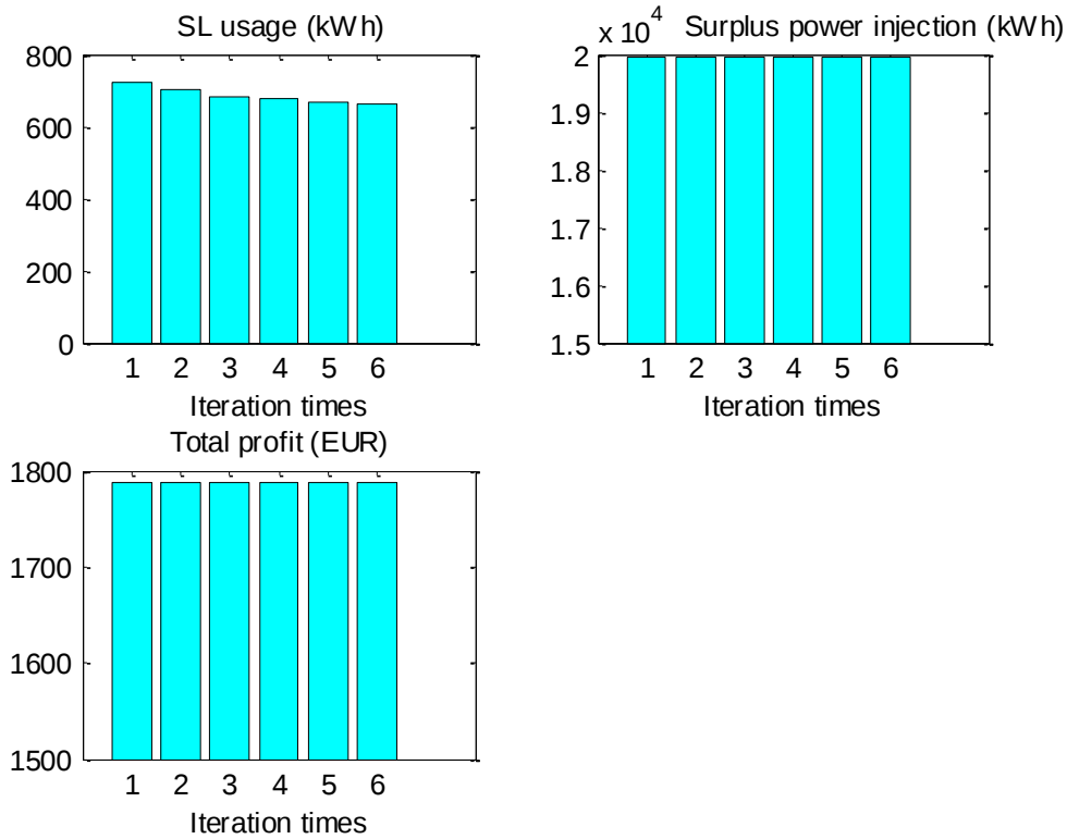
Fig. 4.9 Result of the iteration between the Central CEMS and sub-CEMSs
