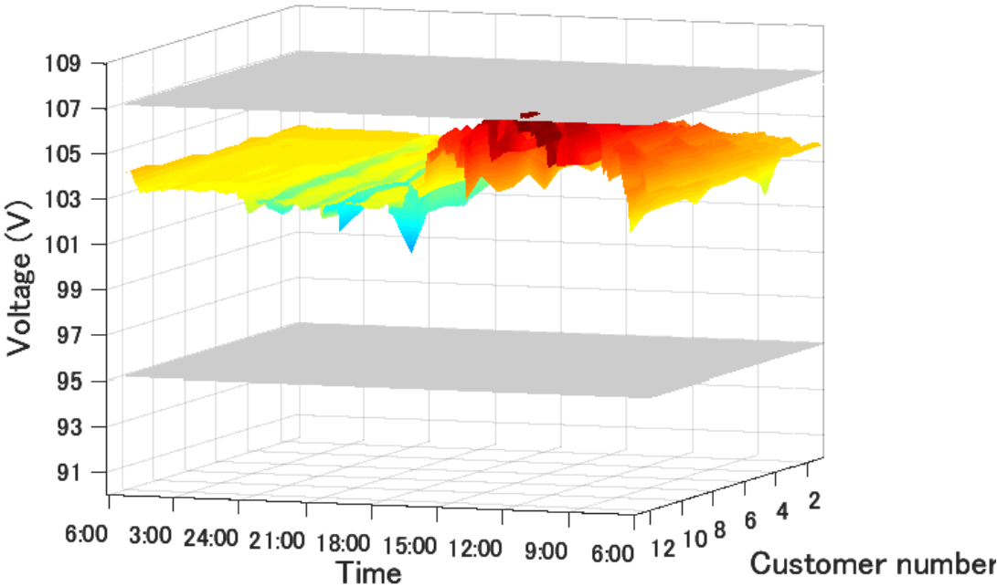
Fig. 4.5 12-customer voltage condition of case 3
