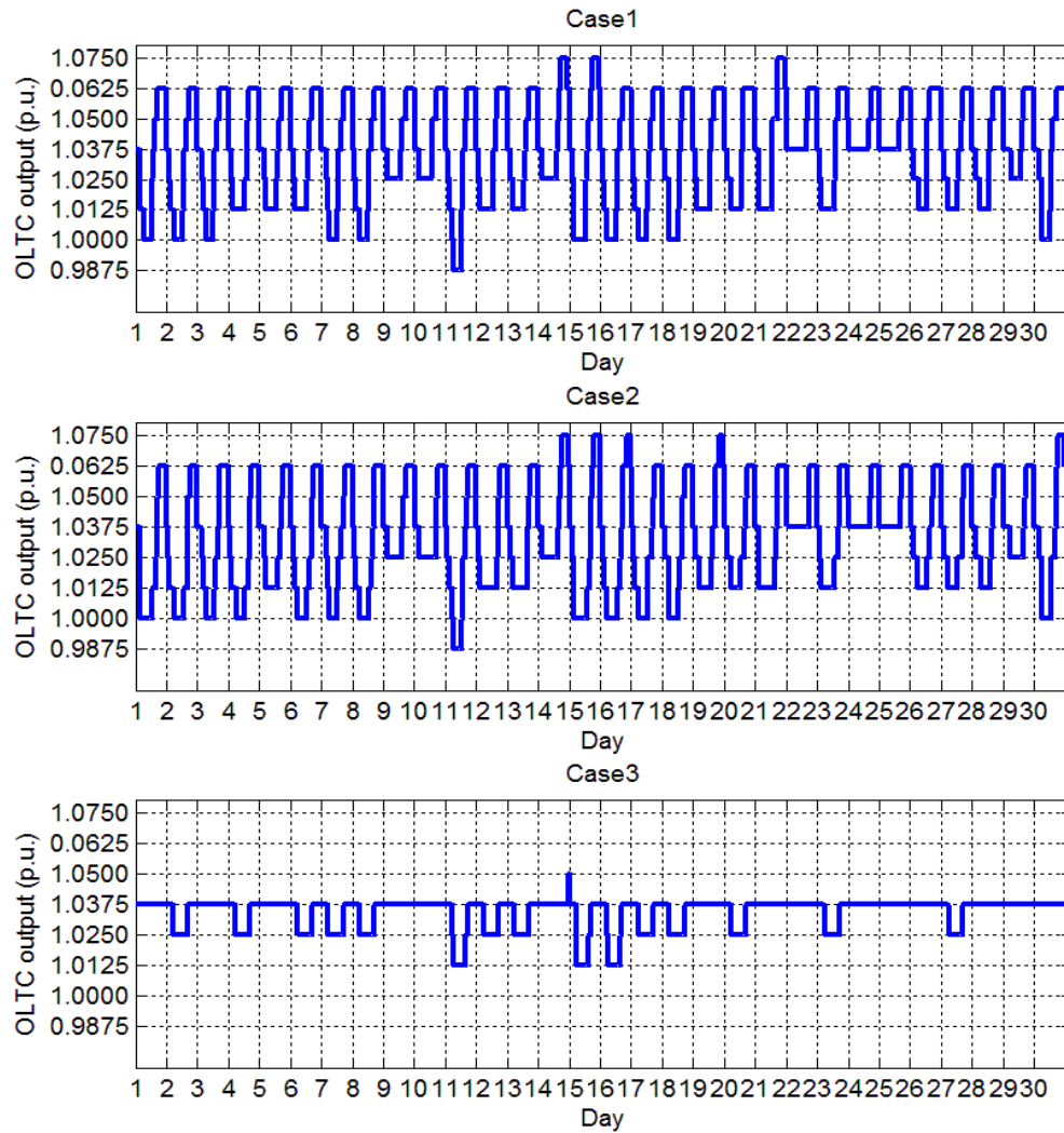
Fig. 4.16 OLTC operation of three cases in 30 days
