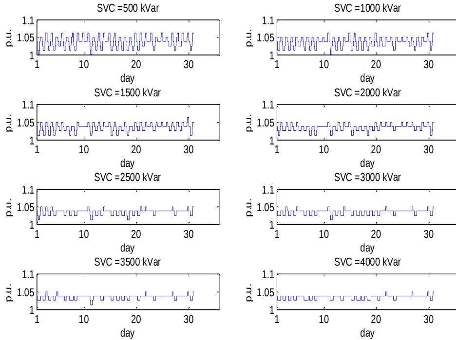
Fig. 4.18 The OLTC operation of the above eight SVC capacity values
