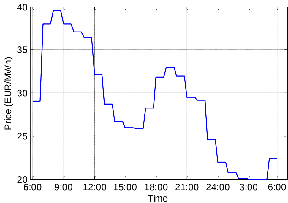
Fig. 3.11 Day-ahead price of 2016.6.2, Denmark
