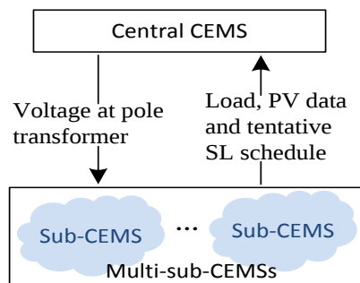
Fig. 3.19 Interaction between central CEMS and multi-sub-CEMS
