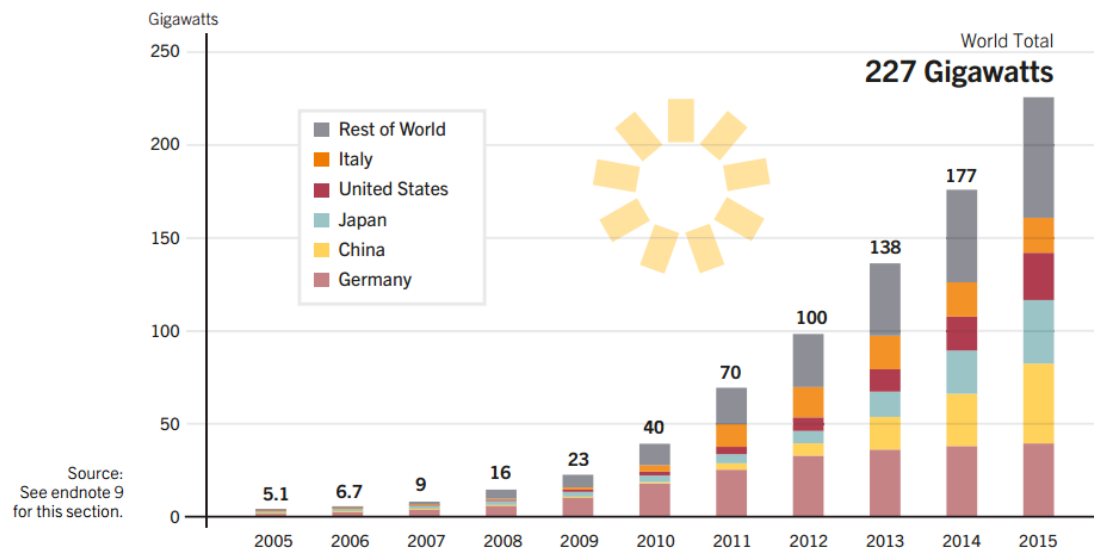
Fig. 1.2 Solar PV Global Capacity, by Country/Region, 2005–2015 [7]
