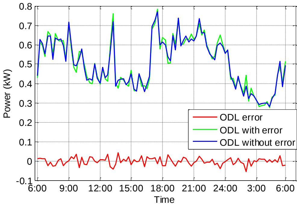
Fig. 3.9 Average ODL data and error
