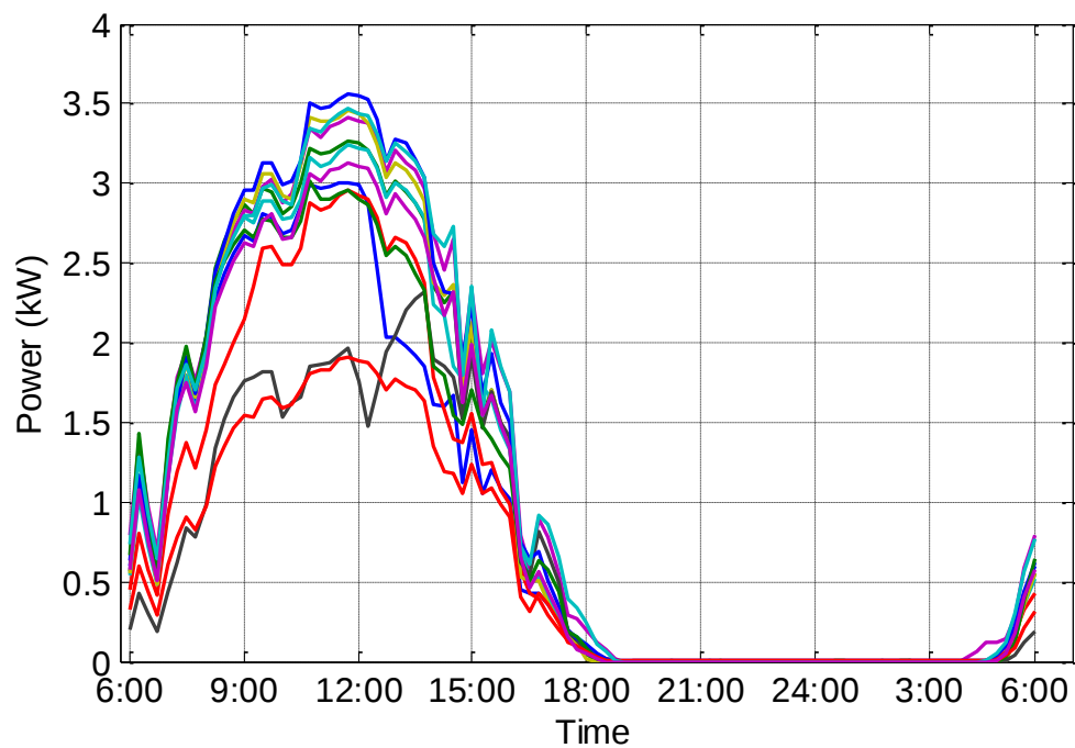
Fig. 3.7 PV profiles of 12 customers
