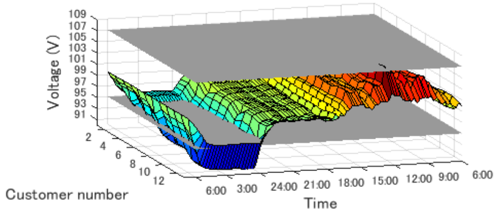
Fig. 3.22 1800-customer voltage condition of case 2 on 2 nd June
