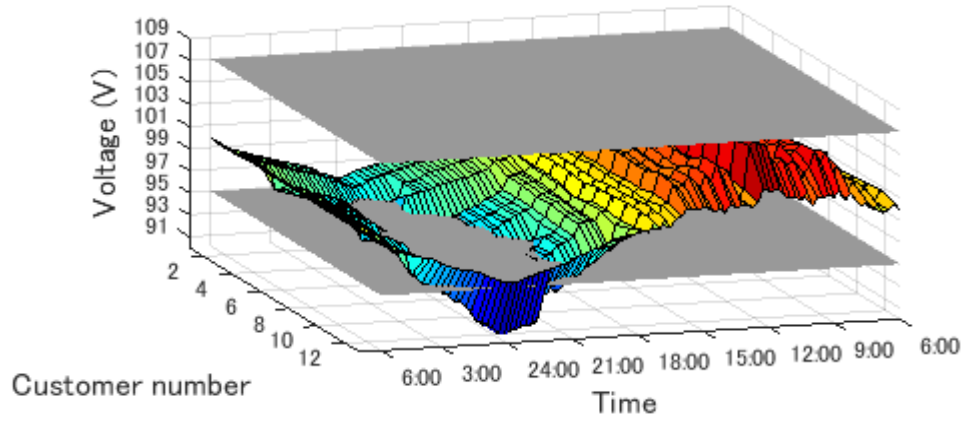
Fig. 3.21 1800-customer voltage condition of case 1 on 2 nd June
