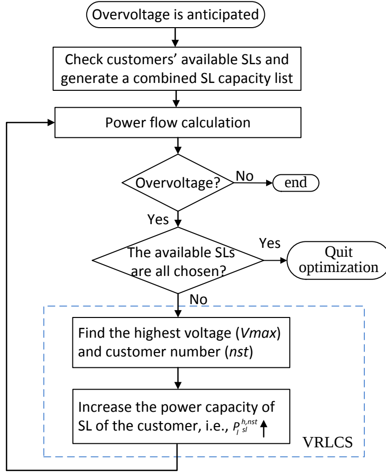
Fig. 4.1 Flowchart of VRLCS process
