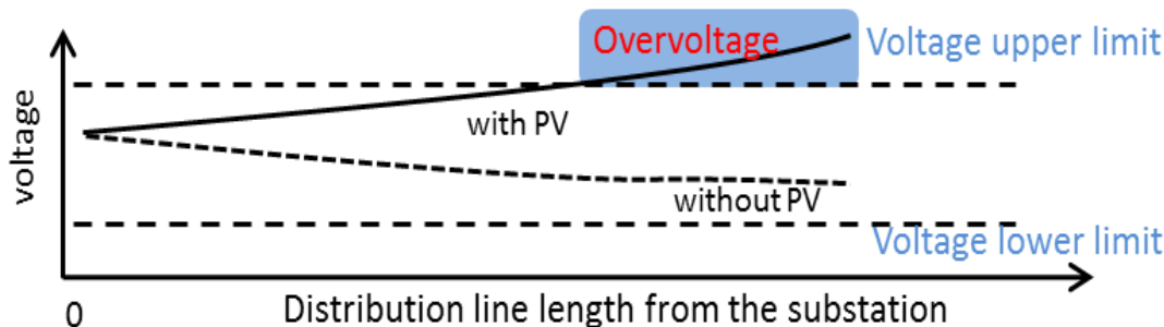
Fig. 1.10 Schematic diagram of overvoltage
