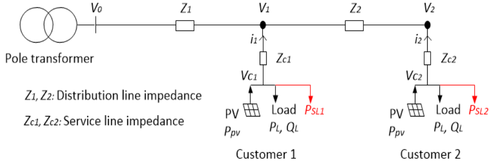
Fig. 1.12 Overvoltage solution by load scheduling
