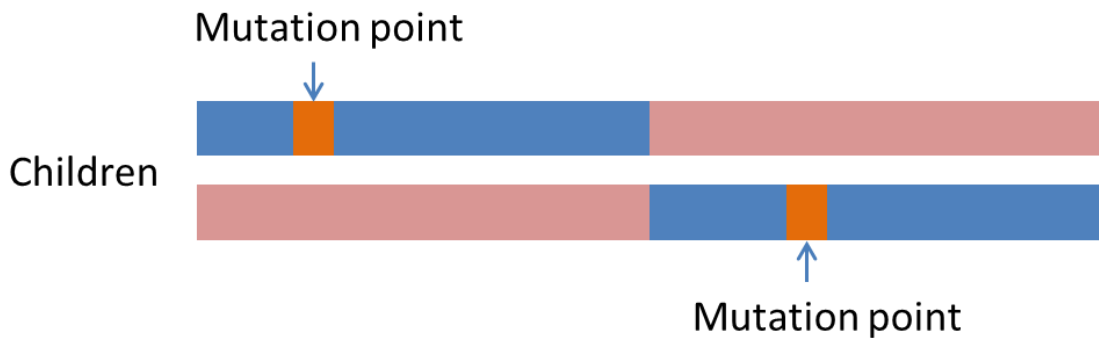
Fig. 3.3 Mutation process
