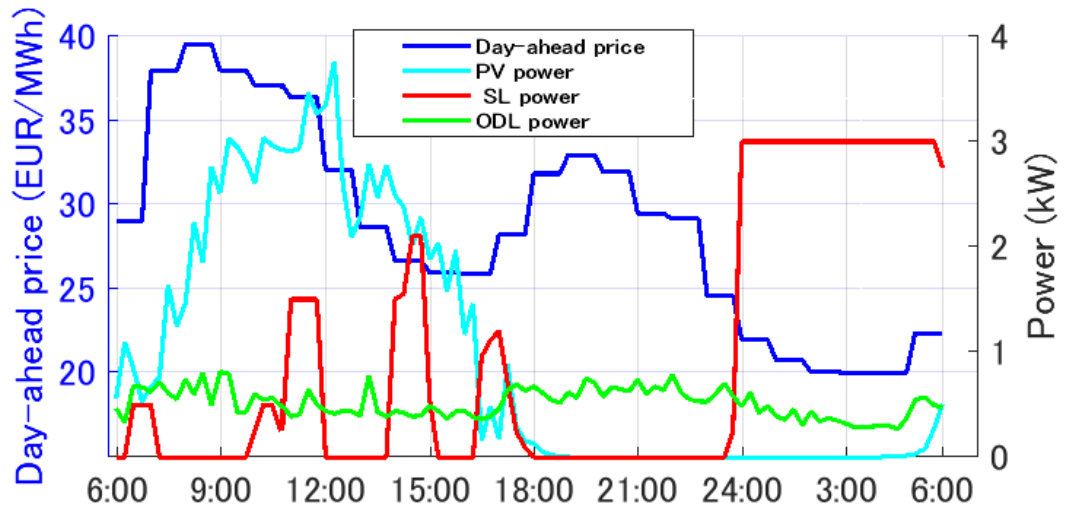
Fig. 3.17 Day-ahead price and PV, SL, ODL average power of case 2
