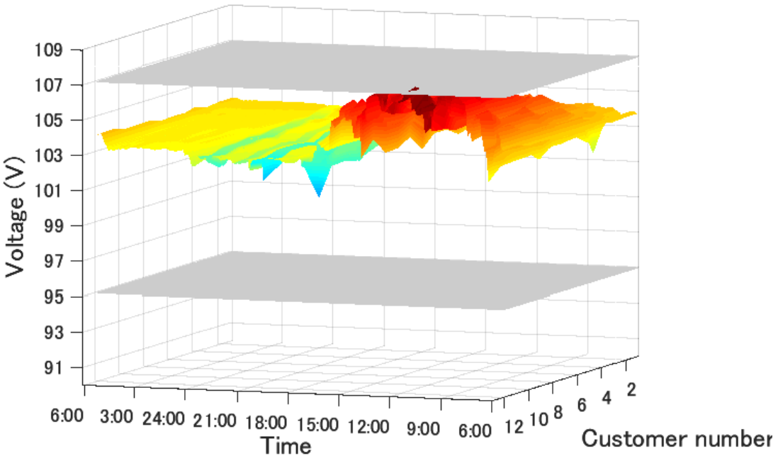
Fig. 4.6 12-customer voltage condition of case 4
