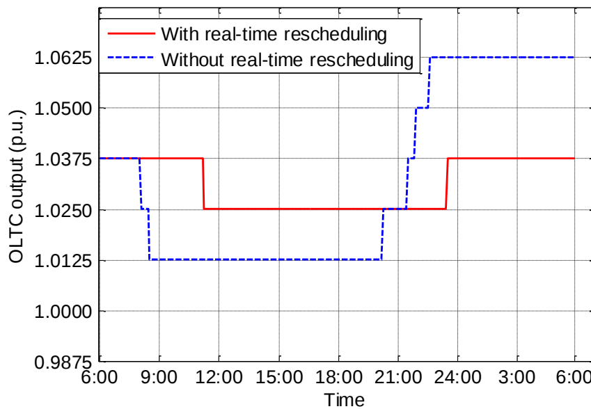
Fig. 4.15 30 days OLTC operation schedule
