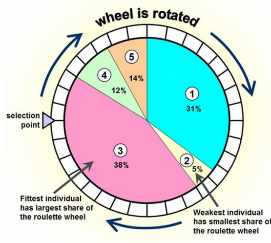
Fig. 3.1 Roulette wheel selection [69]
