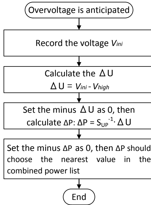
Fig. 4.2 Voltage sensitivity method process
