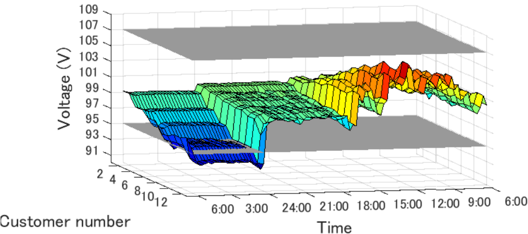
Fig. 3.14 12-customer voltage condition of case 2
