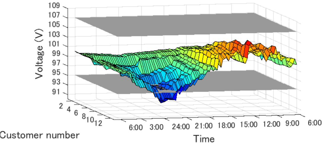
Fig. 3.13 12-customer voltage condition of case 1
