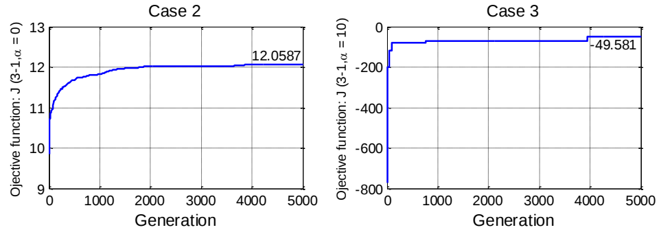
Fig. 3.12 GA iteration result of case 2 and case 3
