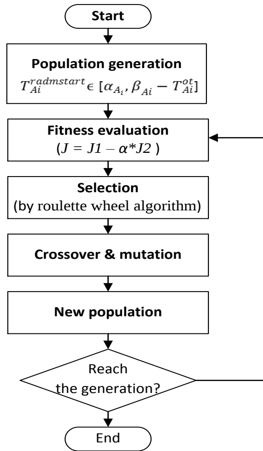
Fig. 3.4 GA optimization process
