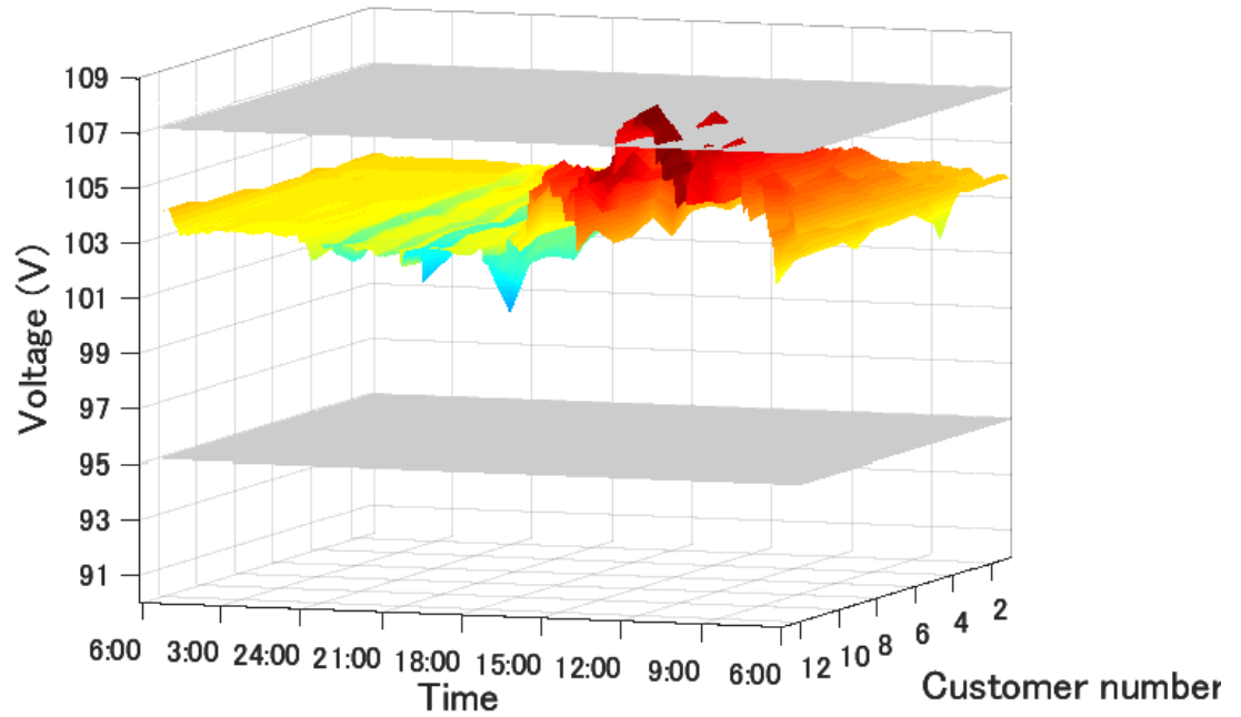
Fig. 4.3 12-customer voltage condition of case 1
