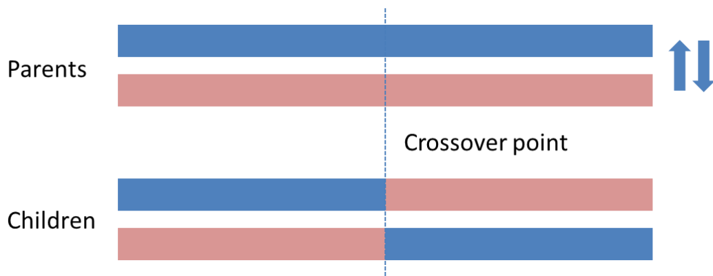
Fig. 3.2 Crossover process
