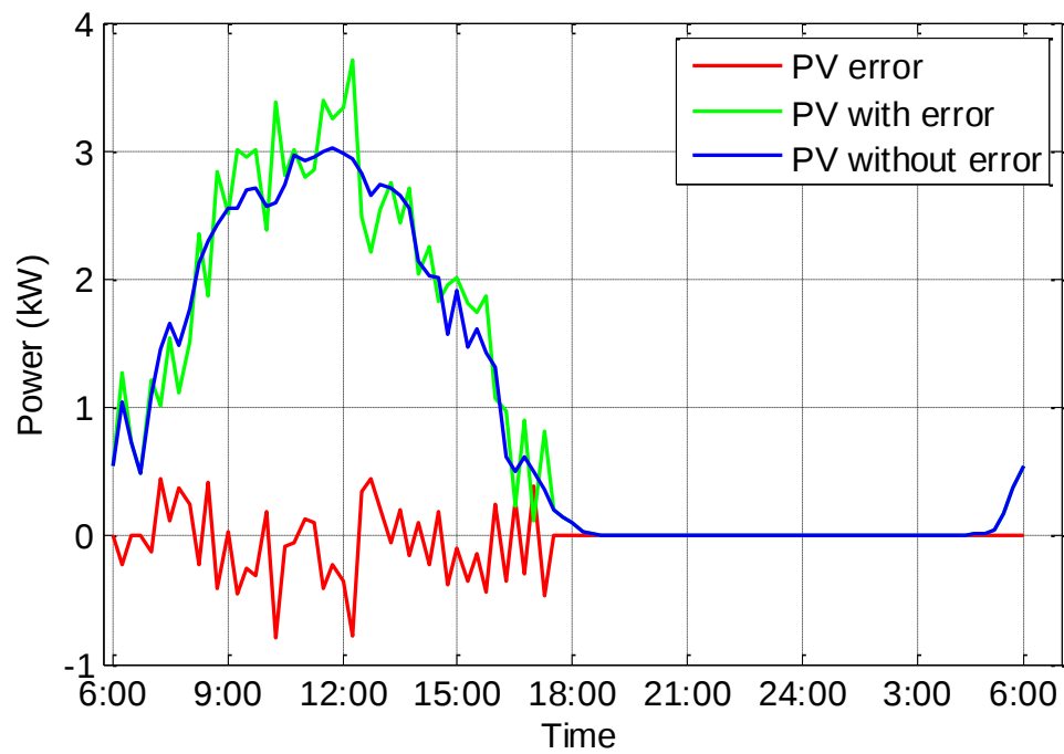
Fig. 3.10 Average PV data and error
