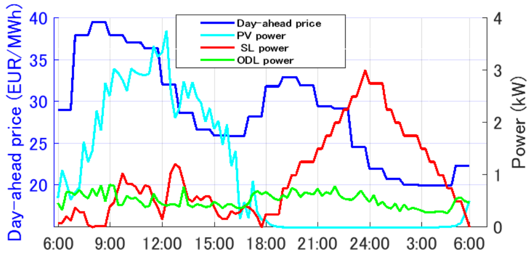
Fig. 3.16 Day-ahead price and PV, SL, ODL average power of case 1
