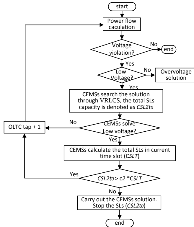
Fig. 4.14 Improved OLTC operation strategy of low voltage
