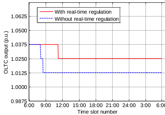
Fig. 4.11 OLTC operation schedule of 2 nd June, 2007
