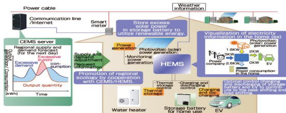
Fig. 1.5 Cooperation of CEMS and HEMS for the total efficient energy using [16]
