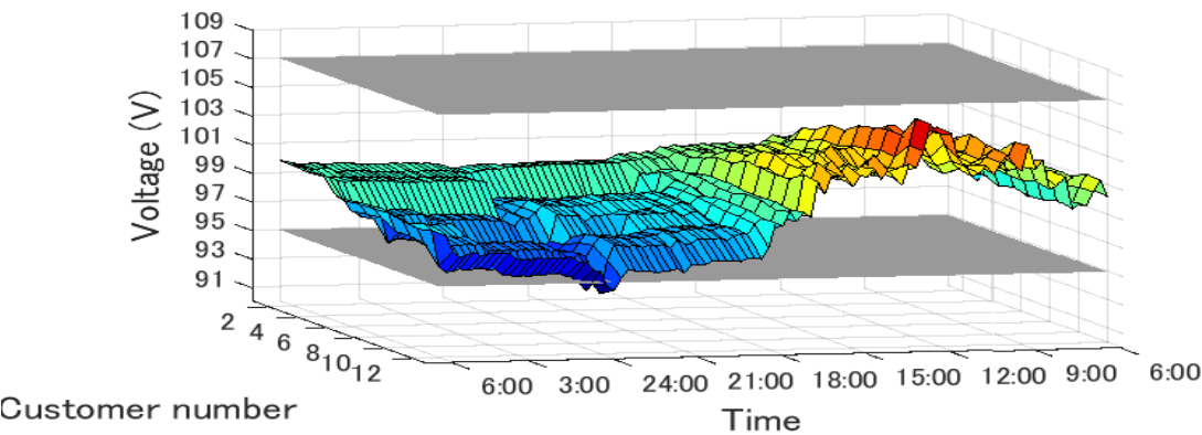
Fig. 3.15 12-customer voltage condition of case 3
