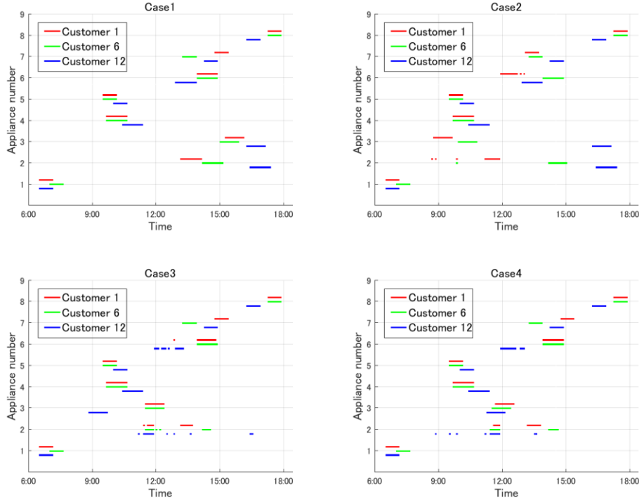
Fig. 4.7 The final SLs working schedule of the four cases
