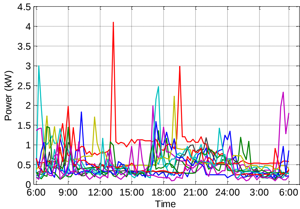
Fig. 3.6 Load profiles of 12 customers
