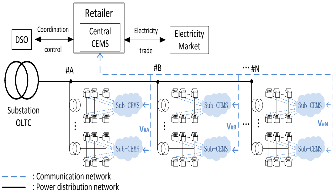
Fig. 2.3 Next generation distribution system model
