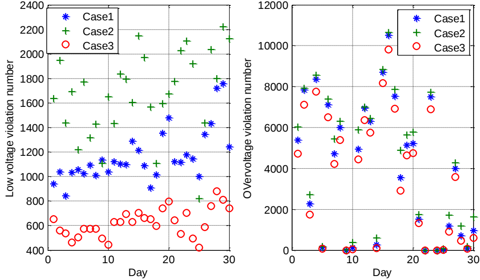
Fig. 3.26 Voltage violation number in 30 days
