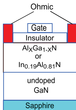
FIG. 1. Scheme of the cross-sectional view of MISH structures used in this study.
