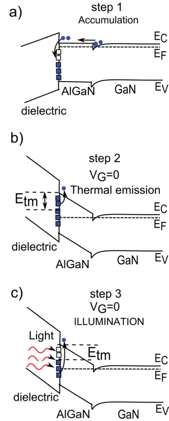
FIG. 4. Schematic band diagrams of an MISH structure illustrating steps of the \Delta V_{th} measurement; E_F is the Fermi level; E_F , E_V , and E_C are the band gap edges.
