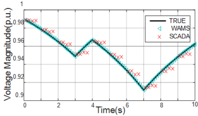
Figure 6.7 Estimation result of SCADA, WAMS Hybrid and true value
