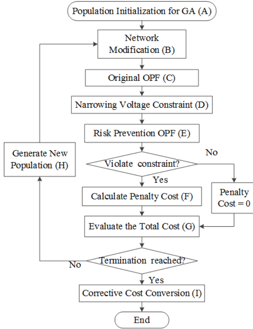
Figure 3.5 Proposed hybrid computation approach for solving opf
