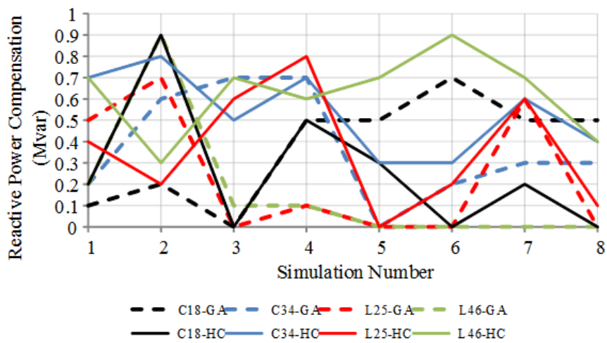
Figure 3.10 Consistency on compensator's tap
