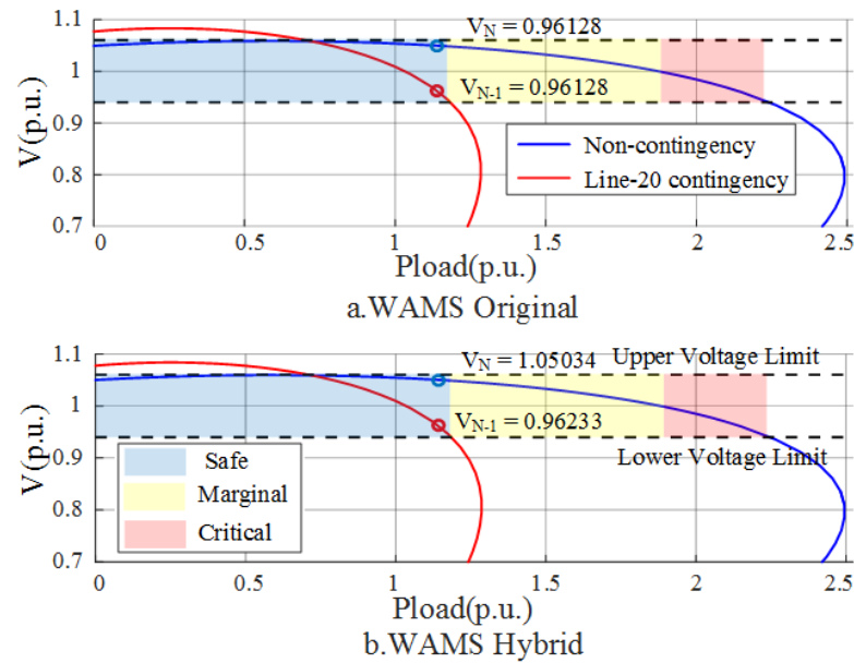
Figure 6.9 Obtained operating condition after RBOPF of WAMS hybrid system
