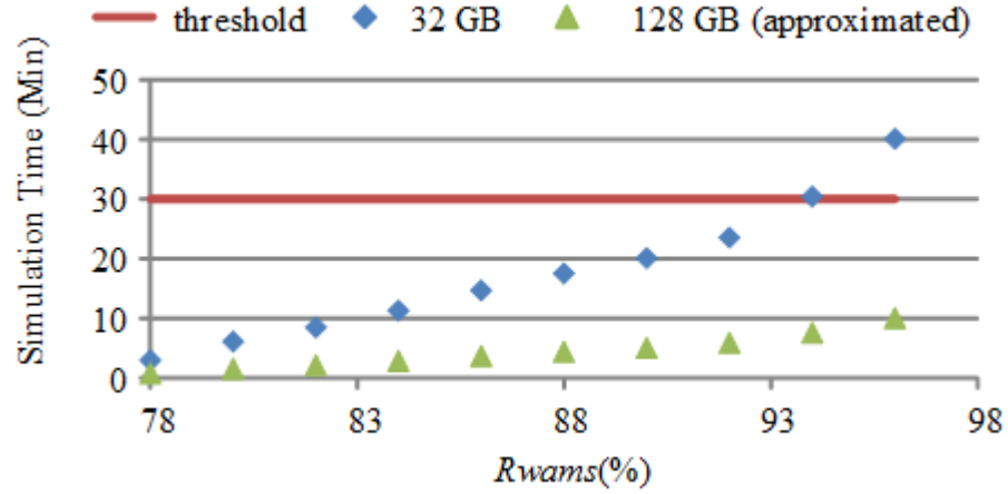
Figure 2.17 Required simulation time at the various R_{wams}
