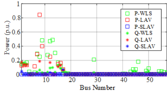
Figure 5.7 Active and reactive power estimation error
