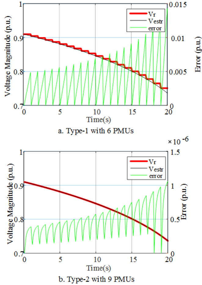
Figure 6.10 Voltage instability case of two different WAMS hybrid types
