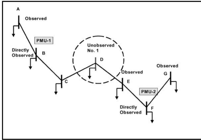
Figure 5.1 Illustration of observable and unobservable of PMU
