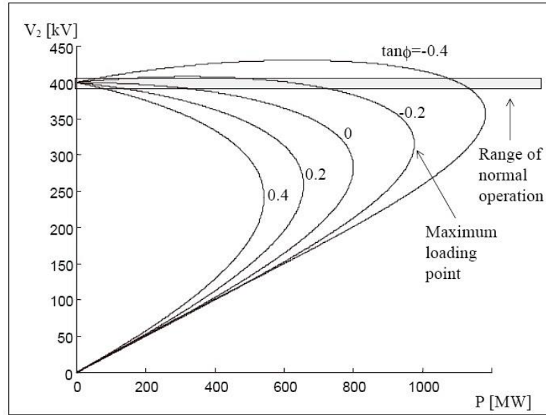
Figure 2.3 P-V curve generated by different operating condition
