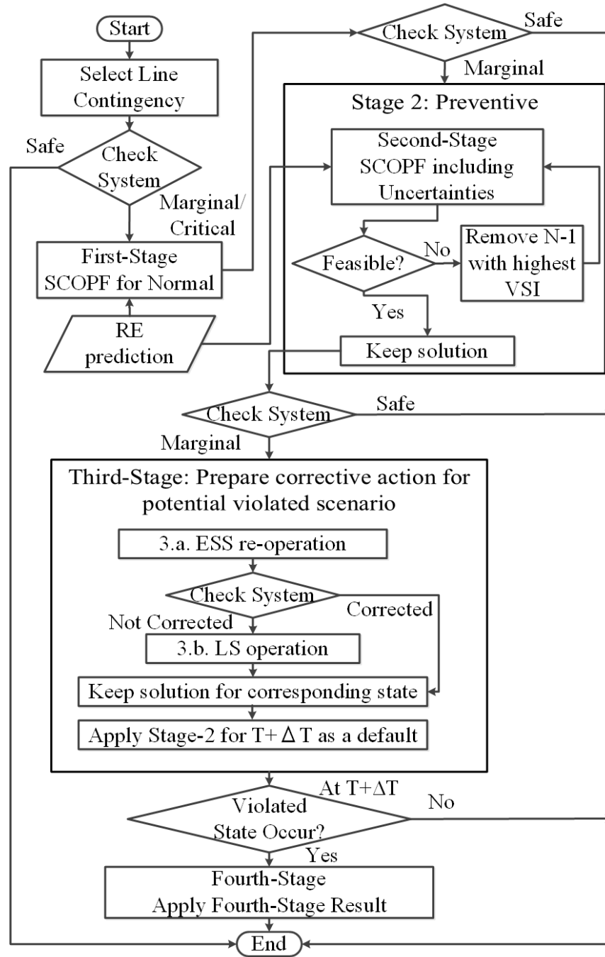
Figure 4.2 Adjustment of preventive scheme with ESS operation
