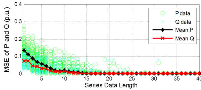
Figure 5.10 MSE of active and reactive power in various data lengths
