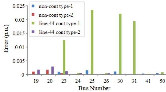
Figure 6.11 Top-10 estimation error for instability case at both WAMS types
