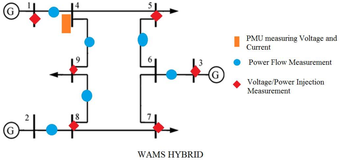
Figure 6.2 Illustration of WAMS hybrid
