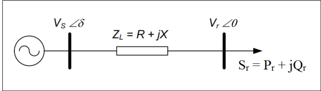
Figure 2.4 Simplified power system model
