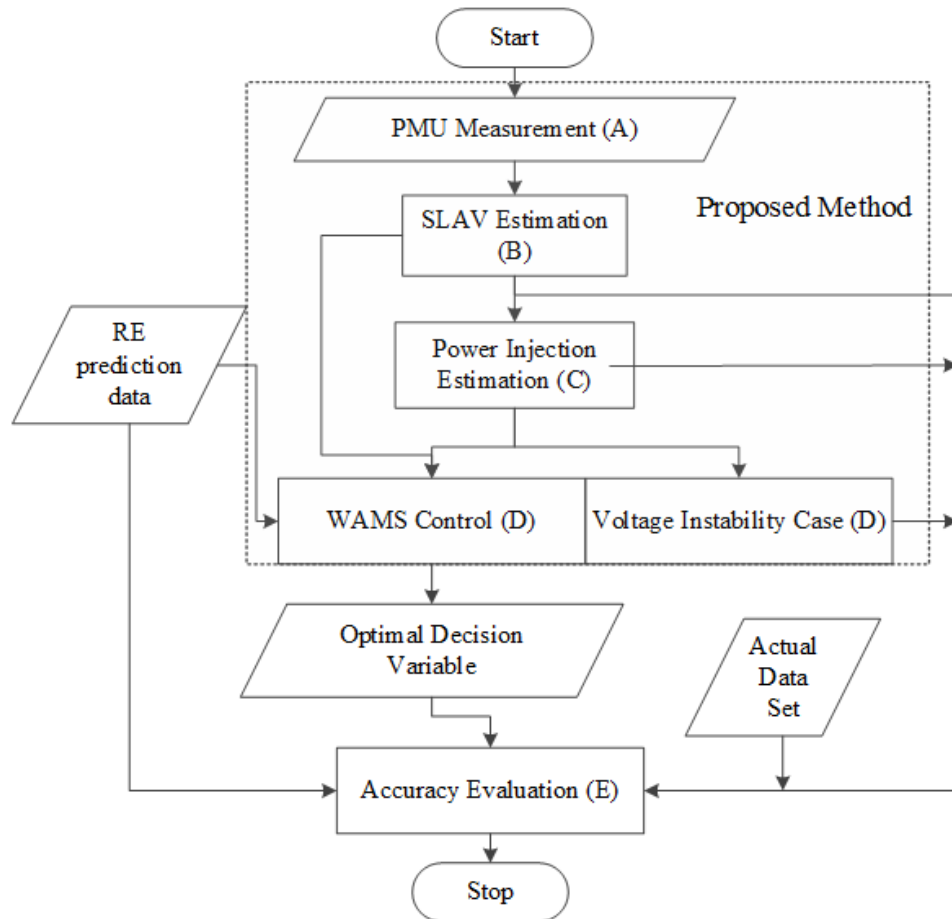
Figure 5.5 State estimation procedure for WAMS voltage stability
