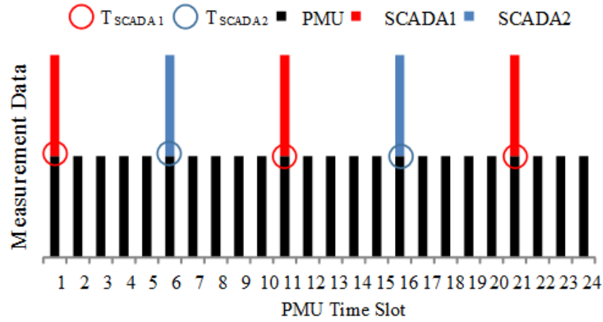
Figure 6.3 Sampling period of PMU and SCADA
