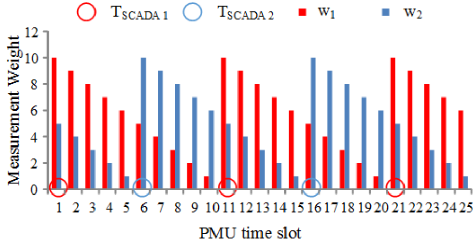
Figure 6.4 Weighting factor of SCADA data in PMU time-slot
