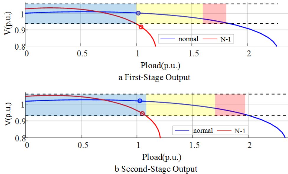
Figure 2.11 Obtained operating condition at moderate RES case
