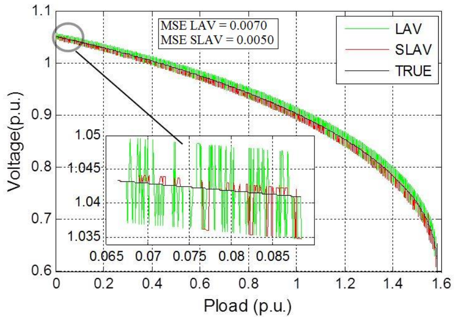
Figure 5.13 Obtained operating point for slow case
