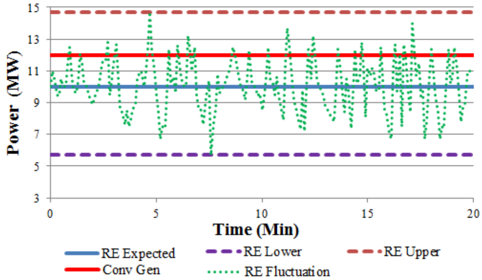
Figure 2.7 Illustration of RES Uncertainty
