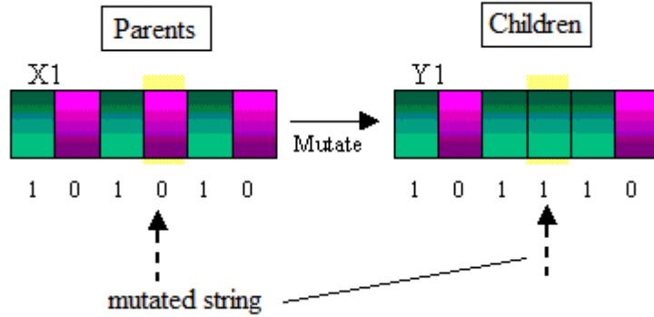
Figure 3.4 Illustration of mutation process
