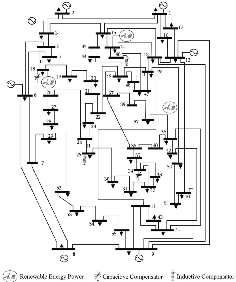
Figure A.1 Modified IEEE 57-bus Test System
