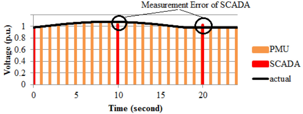
Figure 6.1 Illustration of sampling rates of PMU and SCADA
