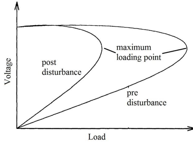
Figure 1.1 P-V curve generated by different operating condition
