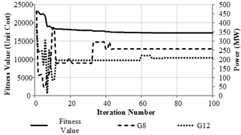
Figure 3.7 Convergence curve of GA-OPF
