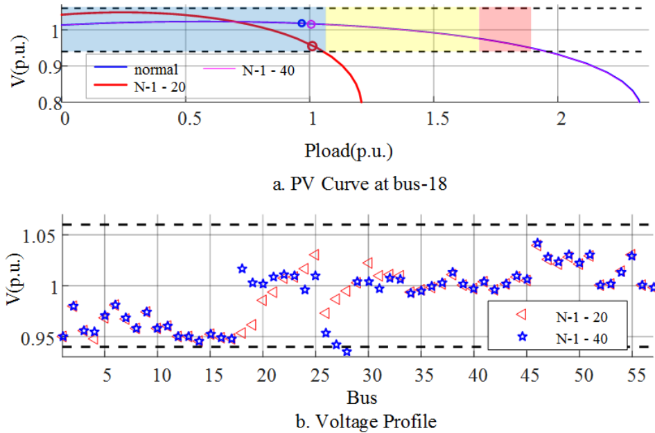
Figure 2.13 Obtained operating condition after second-stage at heavy RES case
