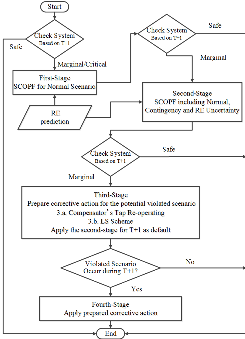
Figure 2.10 Overview of proposed multistage preventive scheme
