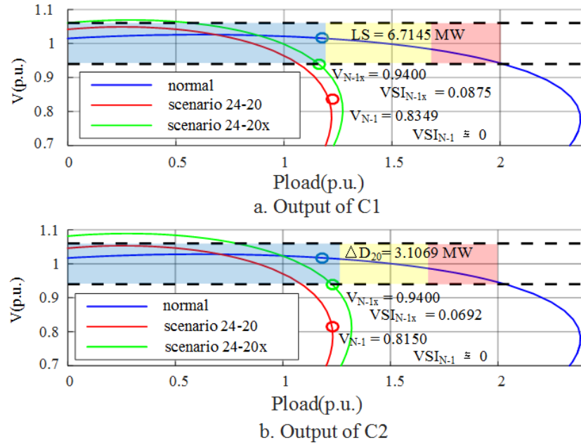
Figure 4.4 Obtained operating condition at 120% loading
