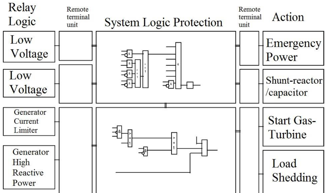
Figure 1.4 Control action logic of Swedish WAMS
