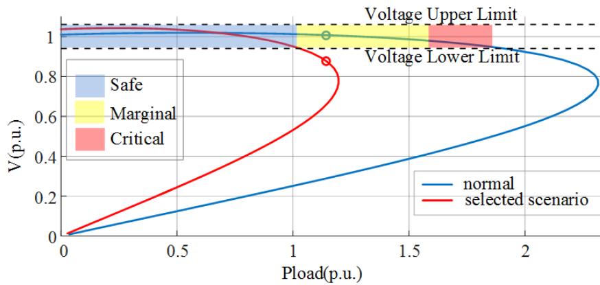
Figure 2.9 Obtained operating point and PV curves for the most severe bus
