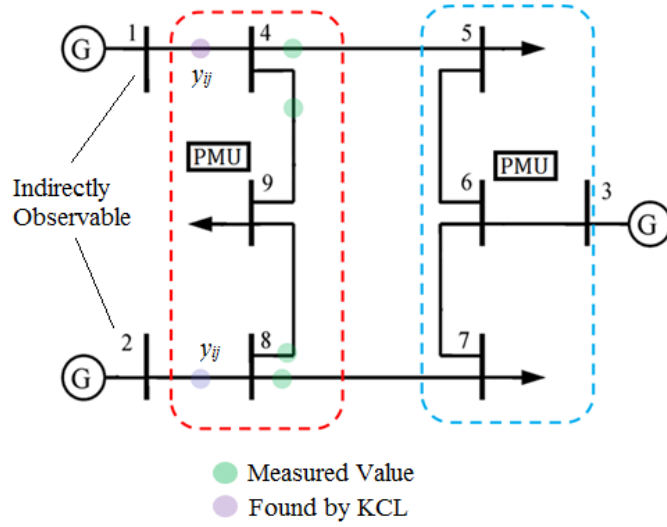
Figure 5.2 Illustration of zero injection bus existence
