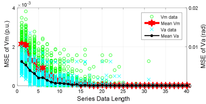
Figure 5.9 MSE of voltage magnitude and angle in various data length
