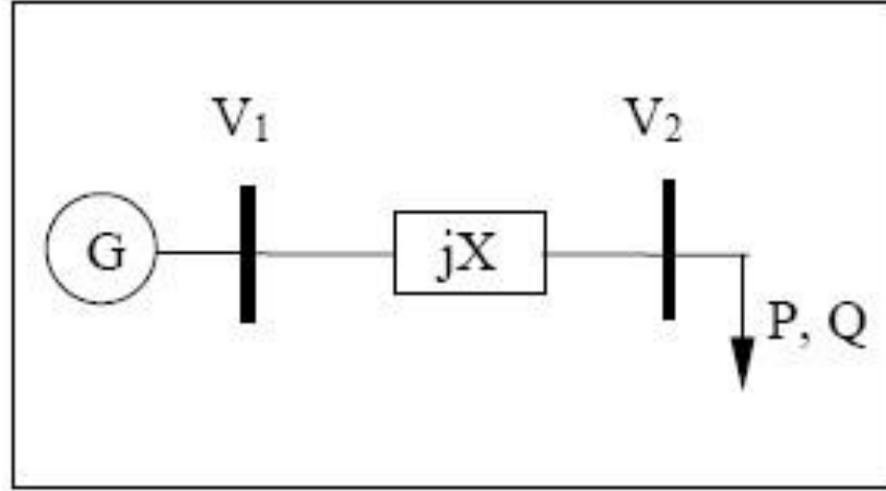
Figure 2.2 Two bus test system
