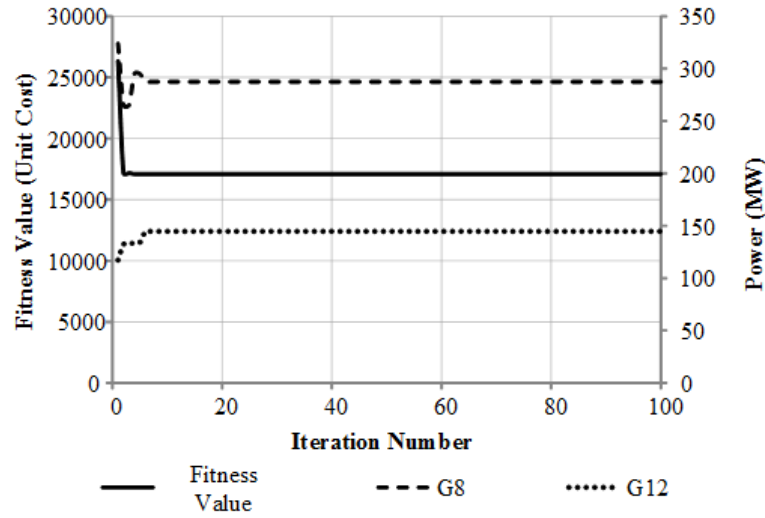
Figure 3.8 Convergence curve of HC-OPF
