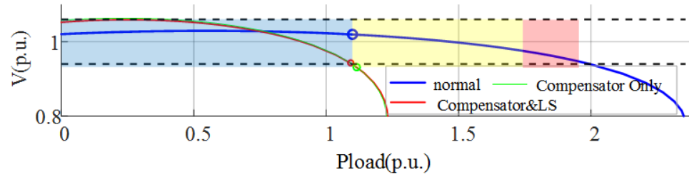
a. PV Curve at bus-18
