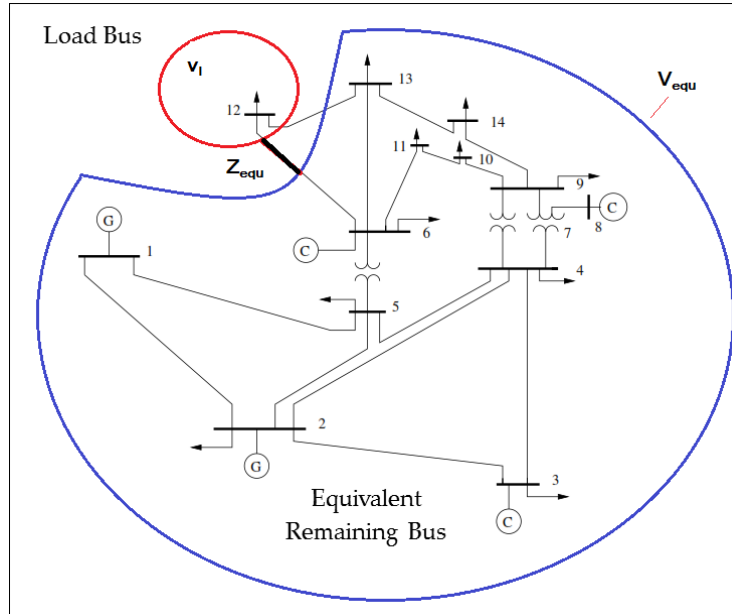
Figure 2.5 Network simplification of power system
