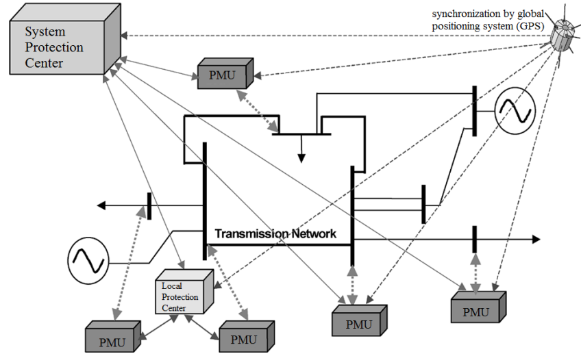
Figure 1.2 Illustration of wide area monitoring system
