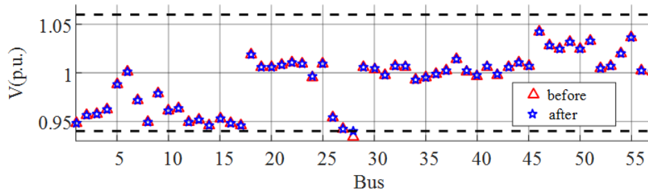
Figure 2.16 Obtained operating condition at stressed load at different stages
