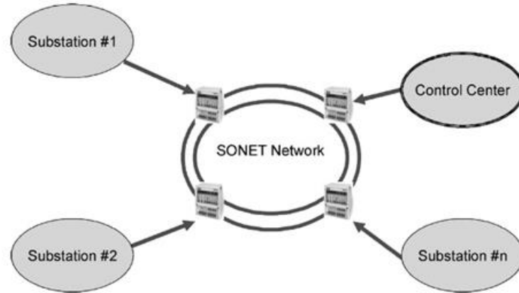
Figure 1.3 Sonet communication system architecture
