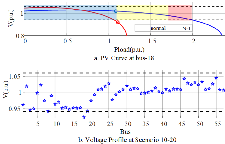
Figure 2.14 Obtained operating condition at stressed load after second-stage
