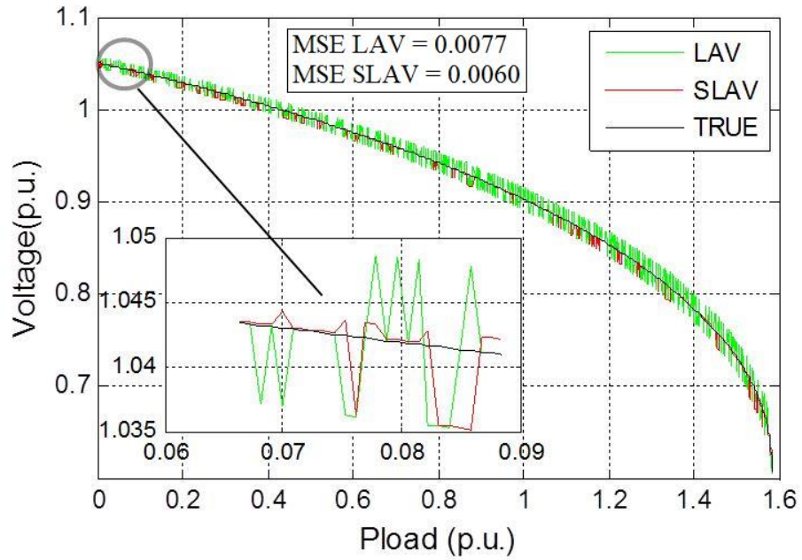
Figure 5.12 Obtained operating point for fast case
