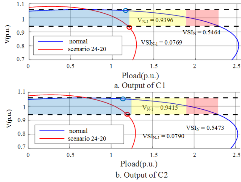
Figure 4.3 Obtained operating condition at 117% loading after second-stage
