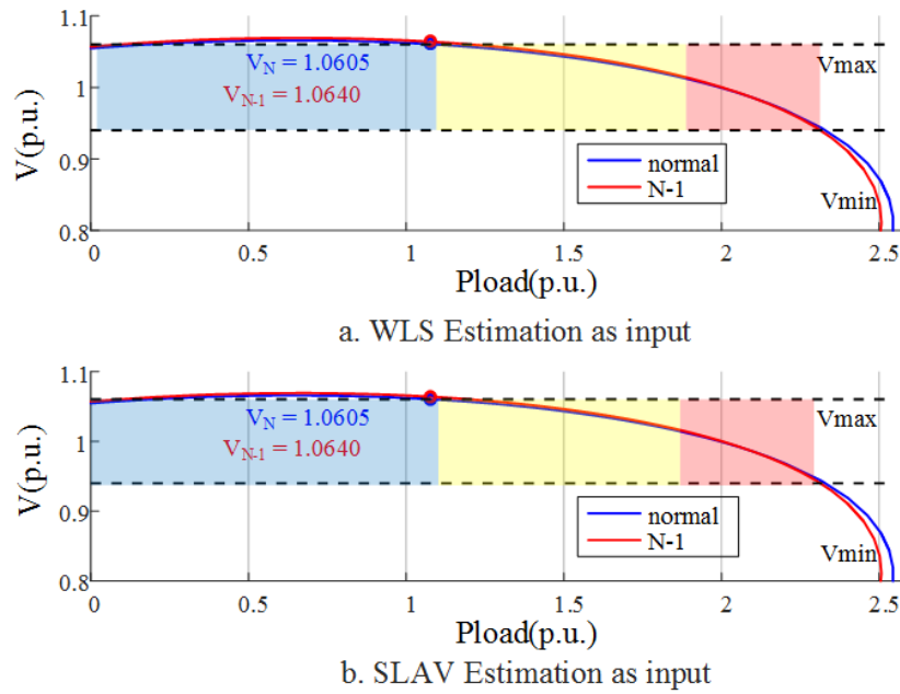
Figure 5.8 Estimation error effect in the obtained operating condition of RBOPF
