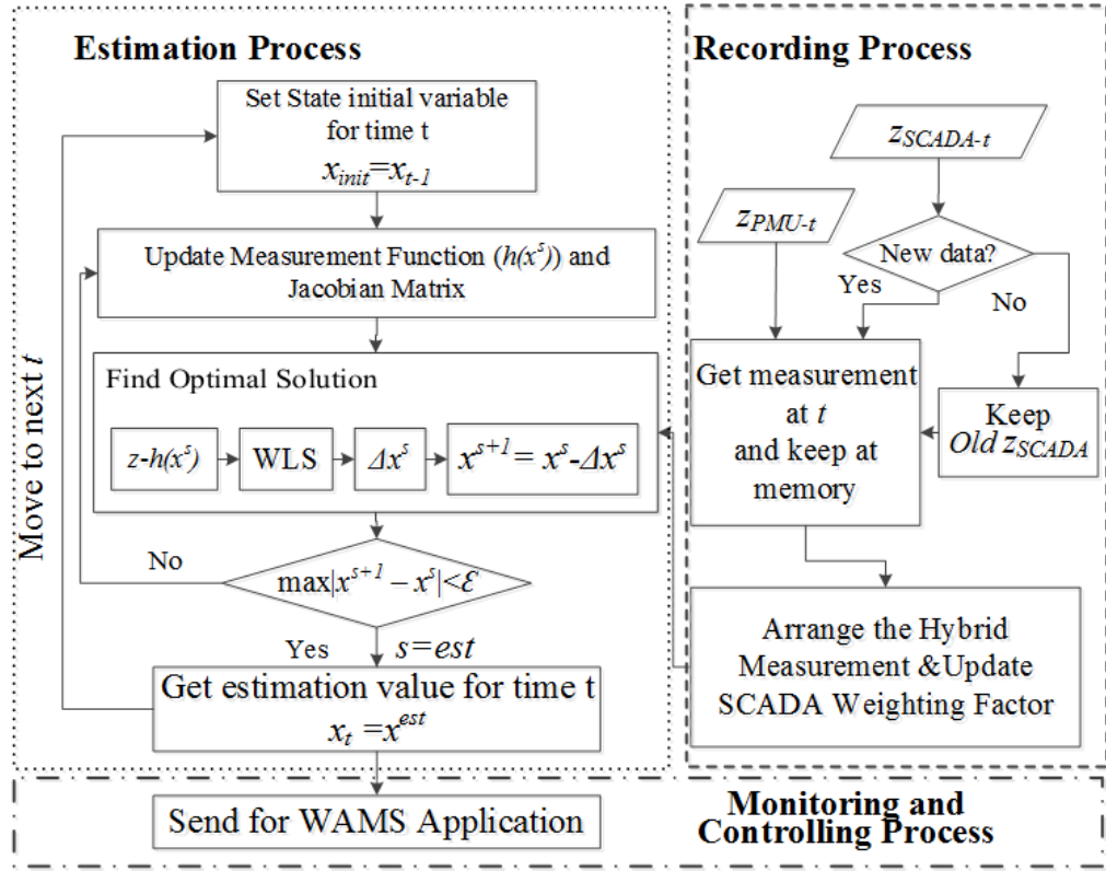
Figure 6.5 Modified state estimation procedure for WAMS hybrid
