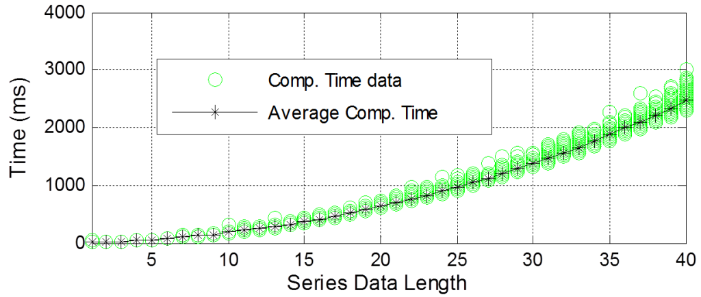
Figure 5.11 Required computation time in various data lengths
