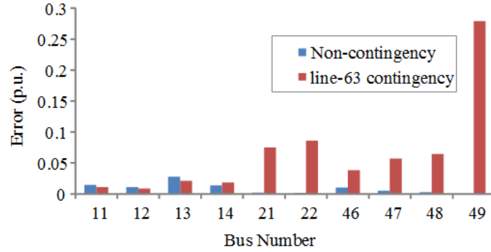
Figure 6.8 Comparison of top-10 individual estimation error of buses voltage
