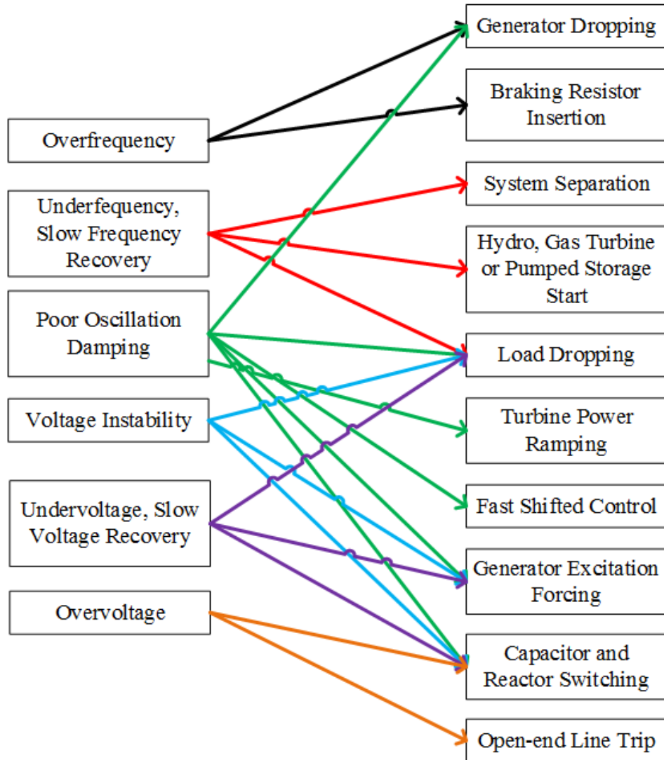
Figure 1.6 WECC RAS emergency control design guideline
