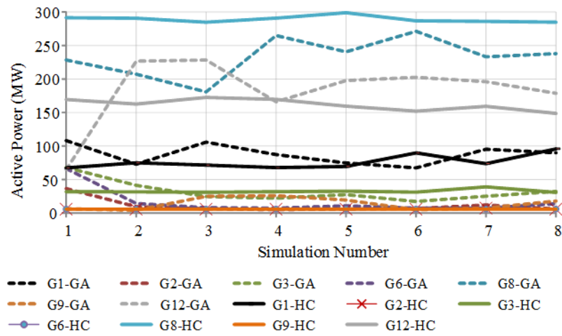
Figure 3.9 Consistency on generator power output
