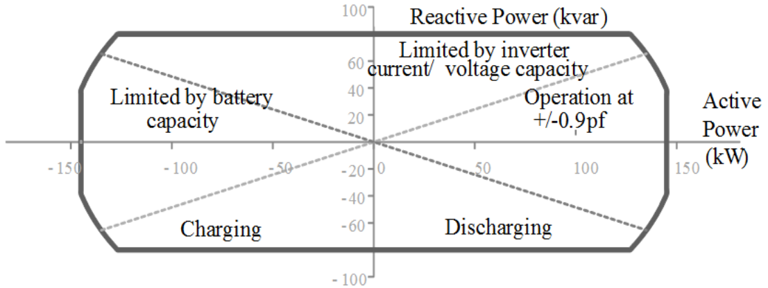
Figure 4.1 Inverter capability curve of ESS with inverter
