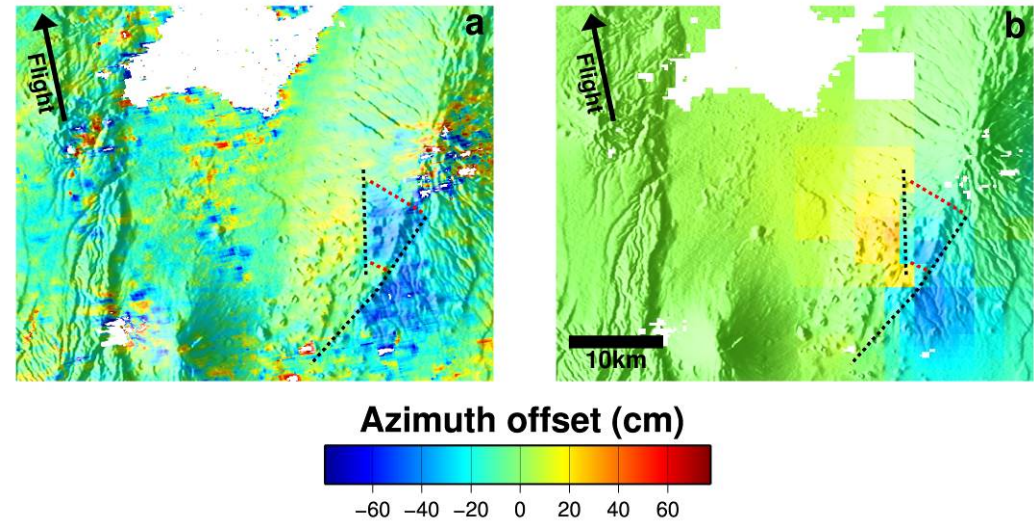
Fig. 3. (a) Observed azimuth offset derived from the ascending pair. (b) Calculated azimuth offset from the estimated slip distributions in the estimated from fault source modeling. Black dashed lines mark the top of the two facing faults. The two phase discontinuities along the direction orthogonal to the fault strike as indicated by the red dashed lines. The arrow in the top left indicates the flight direction of the satellite, and the unit vector is (e_e, e_n, e_z) = (-0.209, 0.978, 0) .
