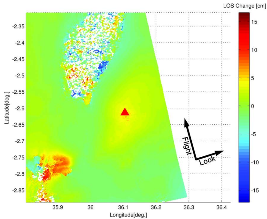
Fig. S2. The post-rifting ascending interferogram spanning 7 Oct. 2007 - 15 Jul. 2010.
