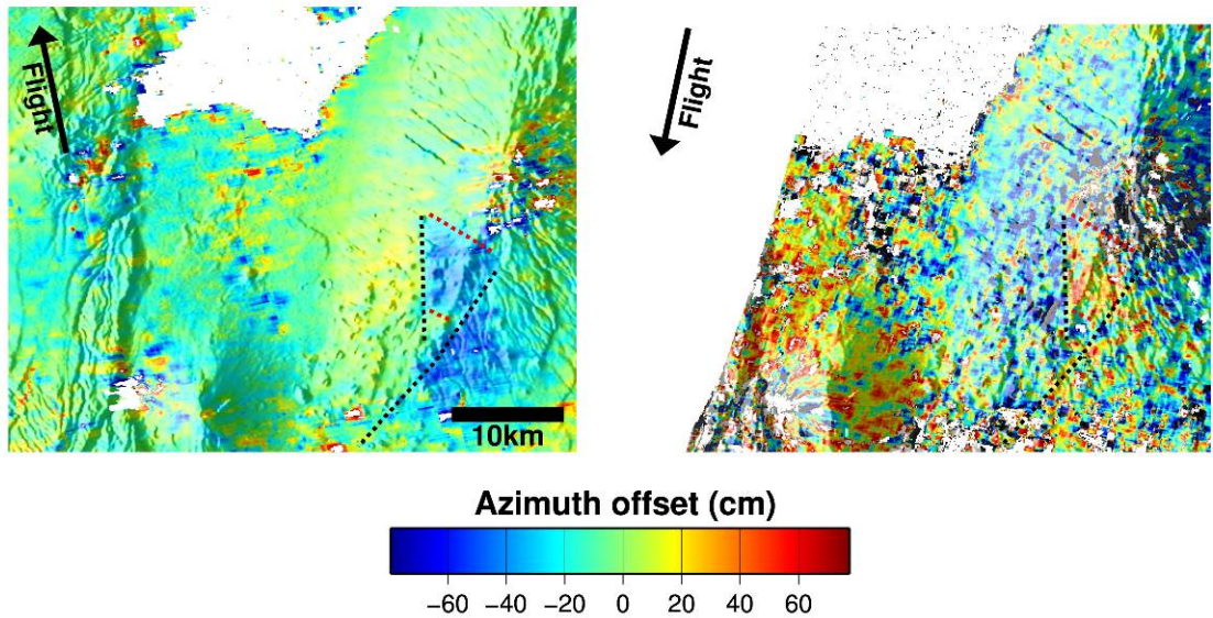
Fig. S1. The observed azimuth offset derived from the ascending (left) and descending data (right) respectively; the left one is the same as Fig 3a. Arrows show the satellite flight directions, and the azimuth offsets are sensitive to such displacements that are parallel to the flight direction. Incoherent area is masked. Black dots lines indicate the top location of the confronted faults (see section 3).
