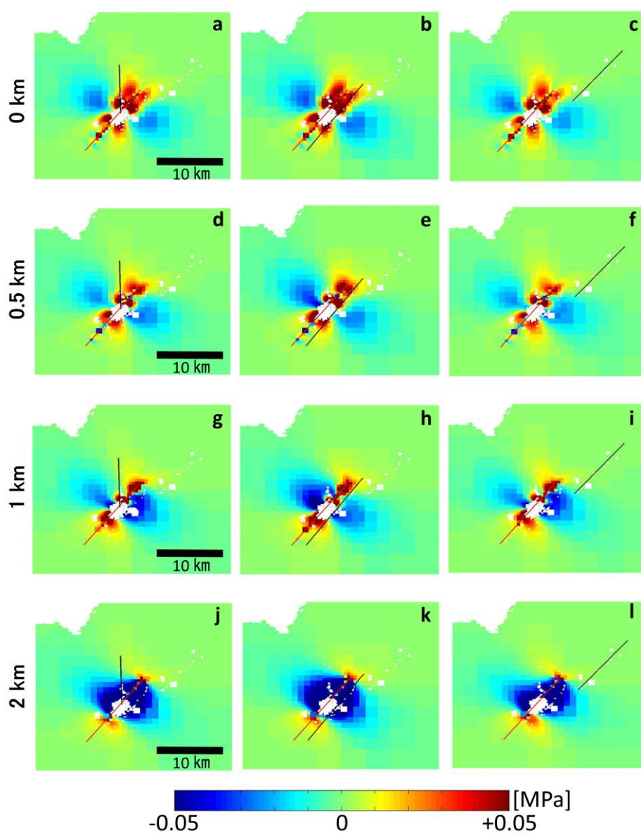
Fig. 7. Coulomb stress changes for the receiver faults (black lines) due to the dike
