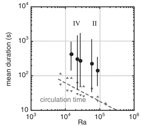
FIG. 9. Plot of the Rayleigh number vs the mean duration of flow patterns (black circles). Bars extending from the circles indicate the range of maximum and minimum durations observed at a Ra . The circulation times estimated from the flow velocities in Figs. 3 and 7 are indicated by a gray dashed line and gray triangles. The imposed horizontal magnetic field here is 18.5 mT ( Q = 1.1 \times 10^3 ).
