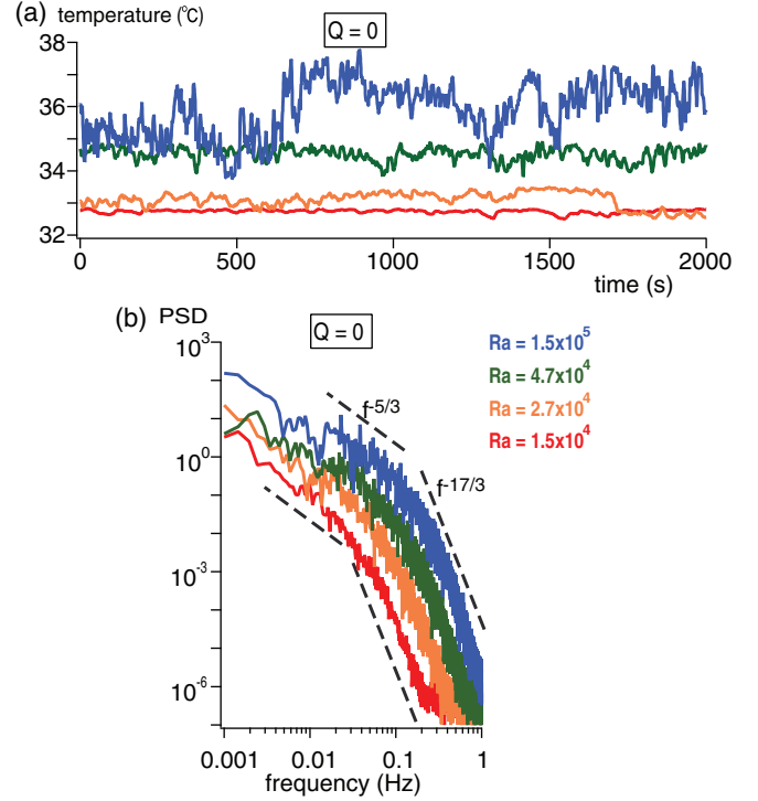
FIG. 4. (Color online) (a) Time series of the temperature and (b) the PSD, for four Ra values without an imposed magnetic field Q = 0 . The dashed lines in the PSD graph indicate the slopes of -5/3 (inertial-convective subrange) and -17/3 (inertial-conductive subrange) expected by the model of developed turbulence for low Pr fluids.
