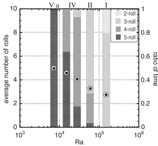
FIG. 8. Plot of the Rayleigh number vs the ratios of the observed times for each number of rolls (columns, right axis) and the average of the number of rolls (concentric circles, left axis). There is an imposed horizontal magnetic field of 18.5 mT ( Q = 1.1 \times 10^3 ).
