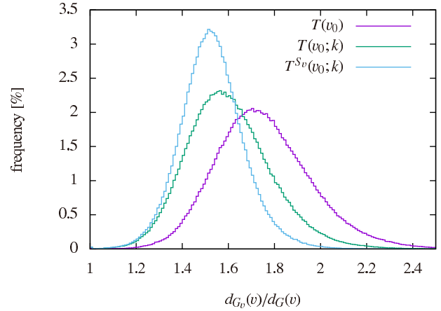
Fig. 2 Distribution of approximation ratio d_{G_v}(v)/d_G(v) of v \in V in ca-AstroPh for G_v = T(v_0) , T(v_0;k) , T^{S_v}(v_0;k) . For T^{S_v}(v_0;k) , the distribution is not for d_{T^{S_v}(v_0;k)}(v) but for their upper bounds d_{T(v_0;k)}(v) - \sum_{e \in S_v} \bar{\delta}_{T(v_0;k),e}(v) . The frequency for range [a, a + 0.01] ( a = 1.00, 1.01, \dots, 2.50 ) is the ratio of the number of vertices v that took the approximation ratio in that range for randomly chosen 100 initial vertices v_0 .
