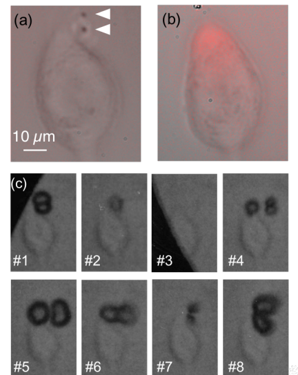
Fig. 8. High-speed and fluorescence observation of bubble dynamics and cell damage. (a) PI fluoresce-overlaid BF image before ultrasound exposure. A cell has two adjacent 1- \mu\text{m} bubbles of Levovist. (b) Image after exposure to one-shot pulsed ultrasound of 0.5 MPa in peak negative pressure. (c) High-speed frames taken at the framing rate of 4 million fps.
