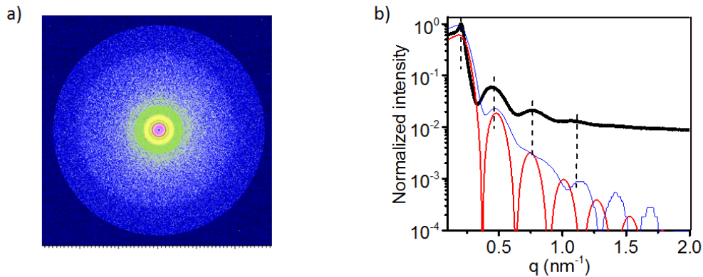
Figure S2. a) Small angle X-ray scattering patterns of B gel. b) SAXS profile of B gel with normalized intensity vs q . The black line is the tested data; the red line is Percus-Yevick fit with parameters R_{HS} = 12.2\text{nm} , \eta = 0.21 ; and the blue line is Percus-Yevick fit considering the size distribution of hard sphere with parameters of R_{HS} = 12.2\text{nm} , \eta = 0.21 , \sigma = 1.4 , where \sigma is variance of R_{HS} in Gaussian distribution.
