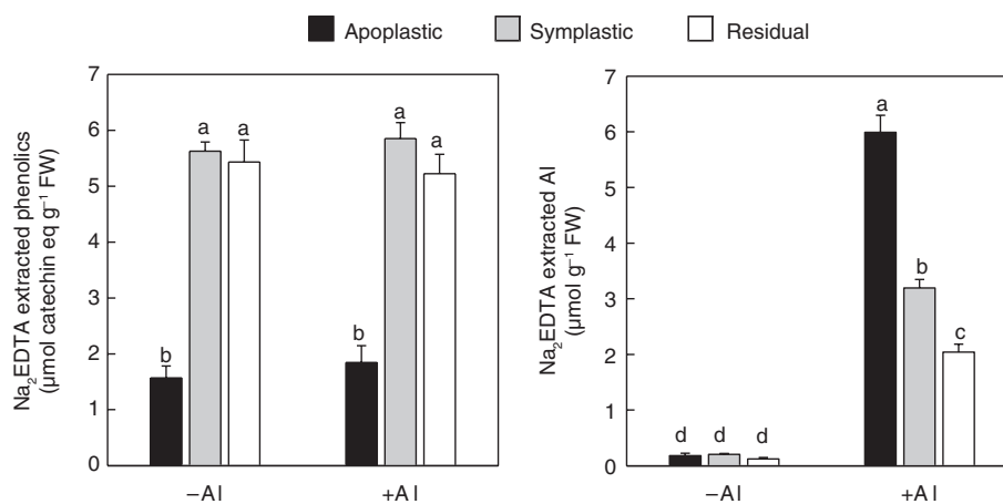
Fig. 5. Na 2 EDTA extracted phenolics and Al concentrations in root of Melastoma malabathricum . Fresh root samples of M. malabathricum were cut into 2 cm segments, and phenolics and Al were extracted with 0.1 M Na 2 EDTA (apoplastic; black bars). Symplastic phenolics and Al were then extracted with 0.1 M Na 2 EDTA by the freeze–thaw method (gray bars). The residue was then ground and extracted again with 0.1 M Na 2 EDTA (residual; white bars). Values are means (n = 4), and error bars indicate se. Different letters indicate significant differences between them.
