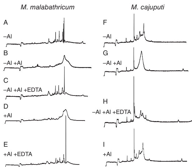
Fig. 6. Profiles of phenolics. Phenolic profiles of Melastoma malabathricum (A–E) and Melaleuca cajuputi (F–I) detected by CE. –Al (A, F) phenolics extracted from roots under –Al treatment; –Al + Al (B, G) mixture of phenolics extracted from roots under –Al treatment and 2 mM AlCl 3 ; –Al + Al + EDTA (C, H) mixture of phenolics extracted from roots under –Al treatment, 2 mM AlCl 3 , and 25 mM EDTA; +Al (D, I): phenolics extracted from roots under +Al treatment; +Al + EDTA (E) mixture of phenolics extracted from roots under +Al treatment and 25 mM EDTA.
